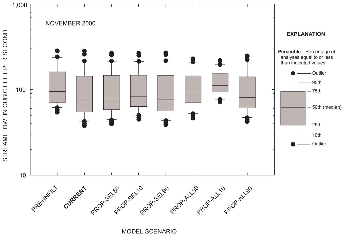
Figure 5-74. Comparison of daily streamflow for observed and simulated conditions at the Marmaton River near the Missouri-Kansas state line, Missouri, November 2000.
