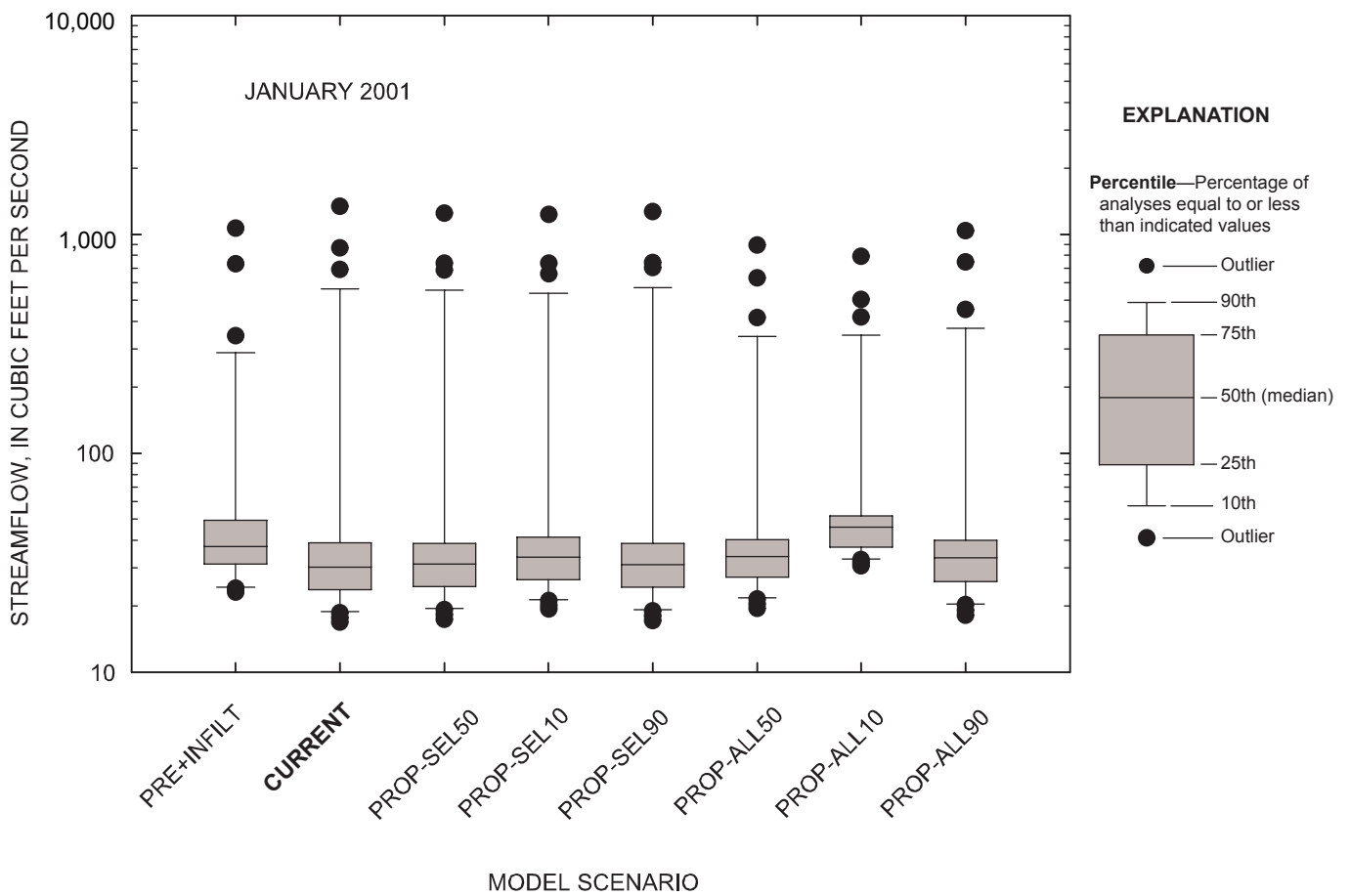
Figure 5-76. Comparison of daily streamflow for observed and simulated conditions at the Marmaton River near the Missouri-Kansas state line, Missouri, January 2001.
