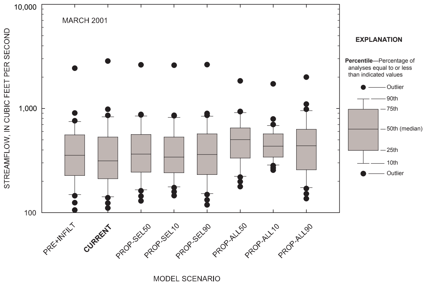
Figure 5-78. Comparison of daily streamflow for observed and simulated conditions at the Marmaton River near the Missouri-Kansas state line, Missouri, March 2001.
