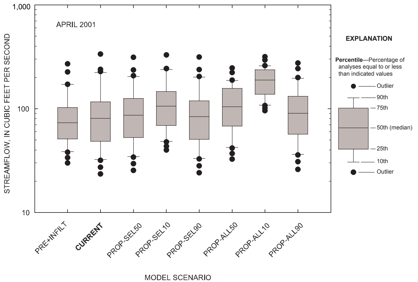
Figure 5-79. Comparison of daily streamflow for observed and simulated conditions at the Marmaton River near the Missouri-Kansas state line, Missouri, April 2001.
