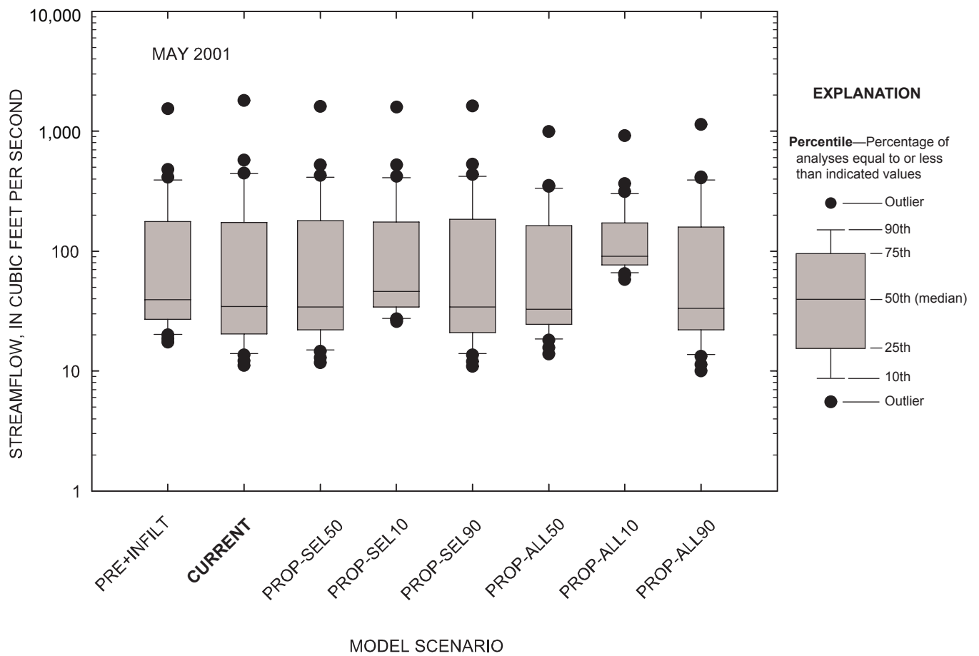
Figure 5-80. Comparison of daily streamflow for observed and simulated conditions at the Marmaton River near the Missouri-Kansas state line, Missouri, May 2001.
