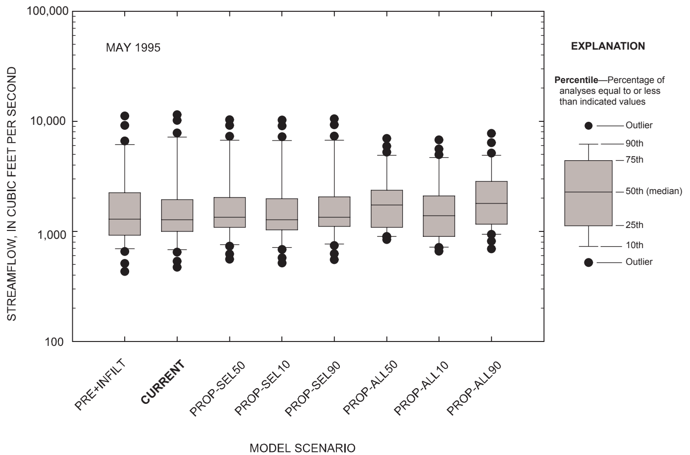
Figure 5-8. Comparison of daily streamflow for observed and simulated conditions at the Marmaton River near the Missouri-Kansas state line, Missouri, May 1995.
