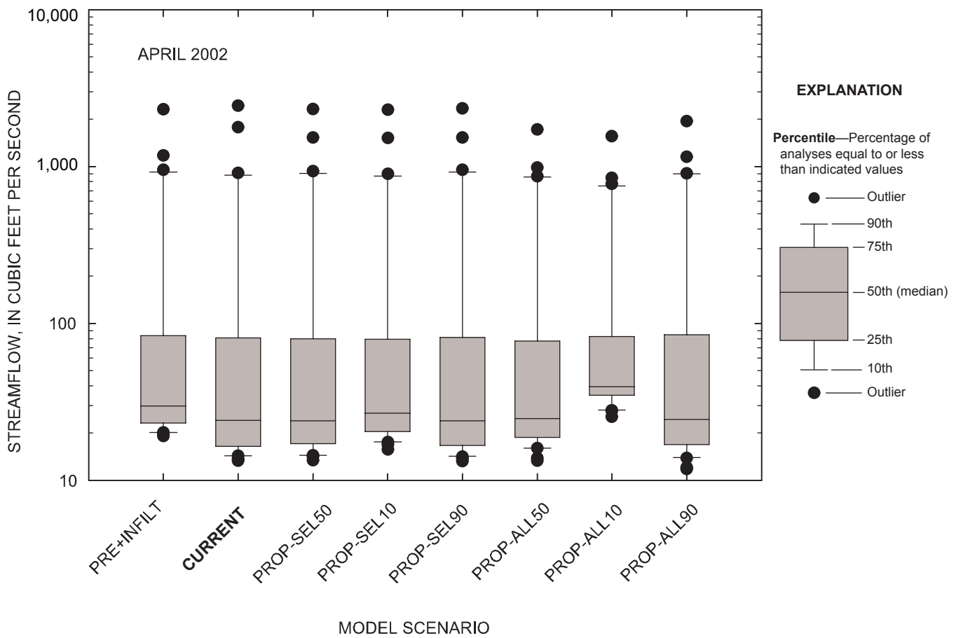
Figure 5-91. Comparison of daily streamflow for observed and simulated conditions at the Marmaton River near the Missouri-Kansas state line, Missouri, April 2002.
