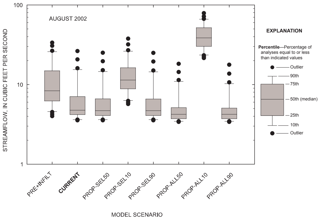
Figure 5-95. Comparison of daily streamflow for observed and simulated conditions at the Marmaton River near the Missouri-Kansas state line, Missouri, August 2002.
