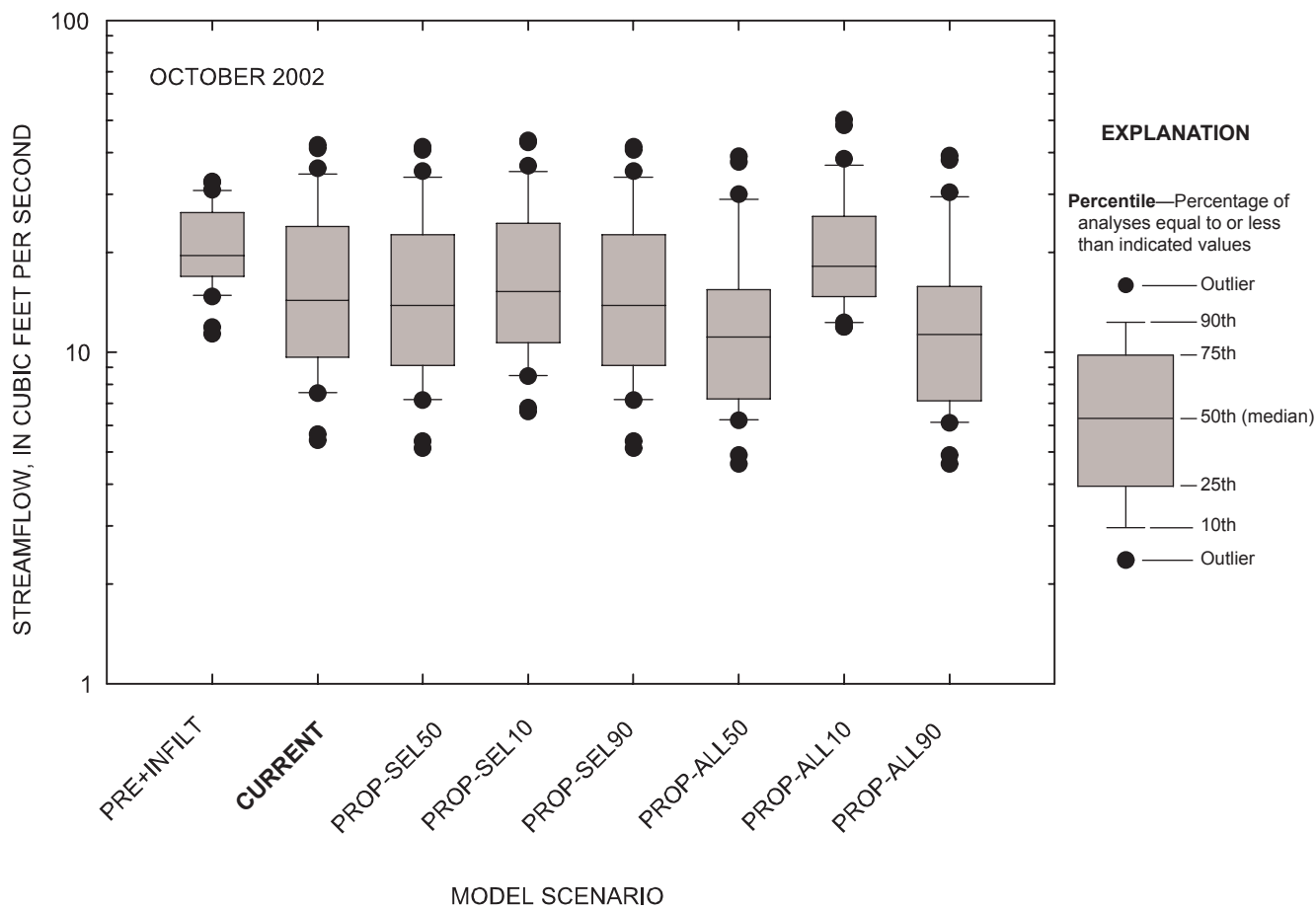
Figure 5-97. Comparison of daily streamflow for observed and simulated conditions at the Marmaton River near the Missouri-Kansas state line, Missouri, October 2002.
