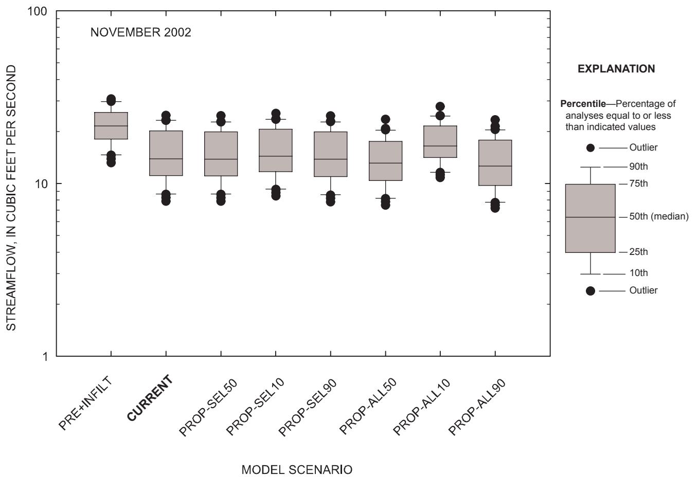
Figure 5-98. Comparison of daily streamflow for observed and simulated conditions at the Marmaton River near the Missouri-Kansas state line, Missouri, November 2002.
