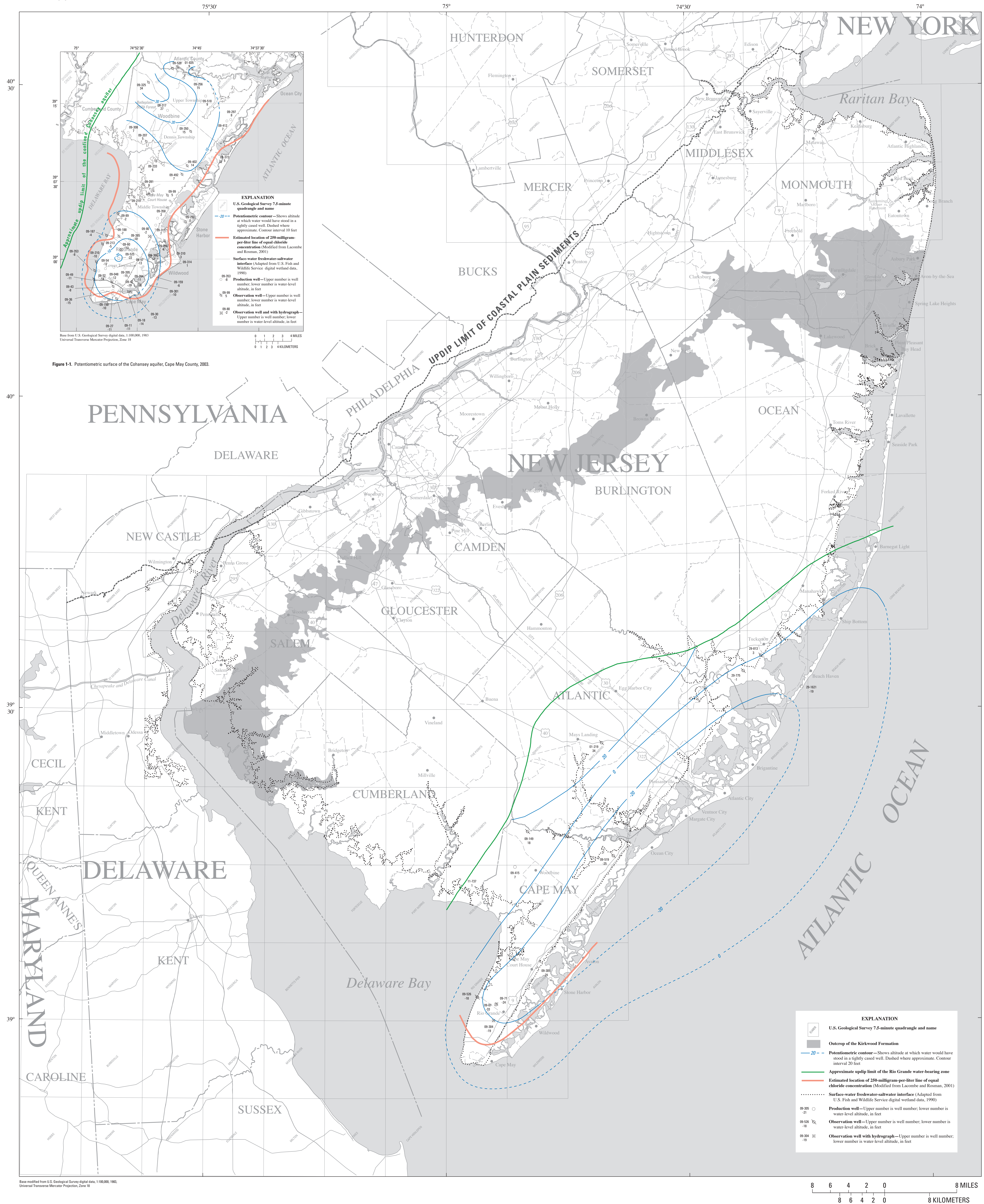
Figure 1-2. Potentiometric surface of the Rio Grande water-bearing zone, New Jersey Coastal Plain, 2003.
