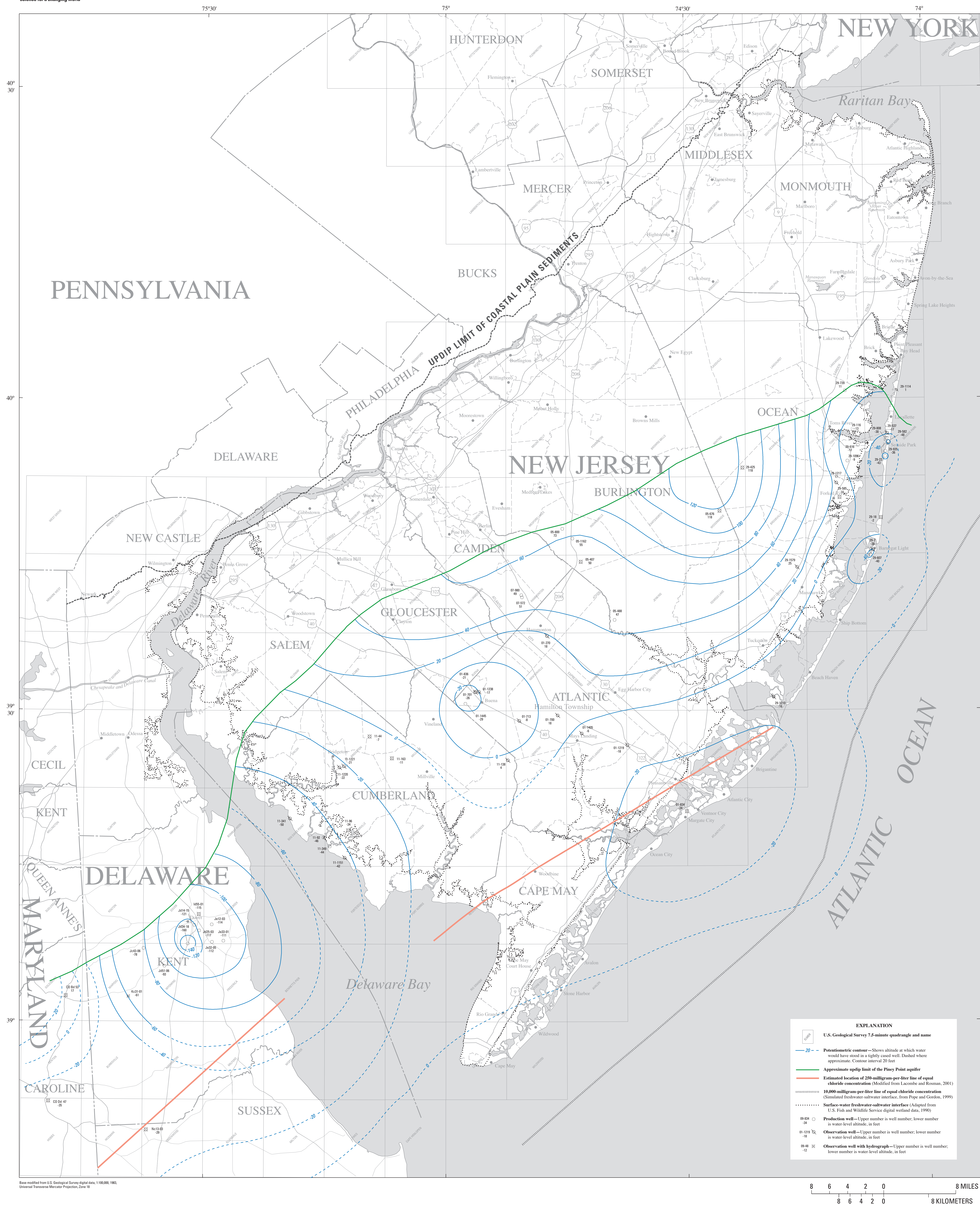
Potentiometric Surface of the Piney Point aquifer, 2003
