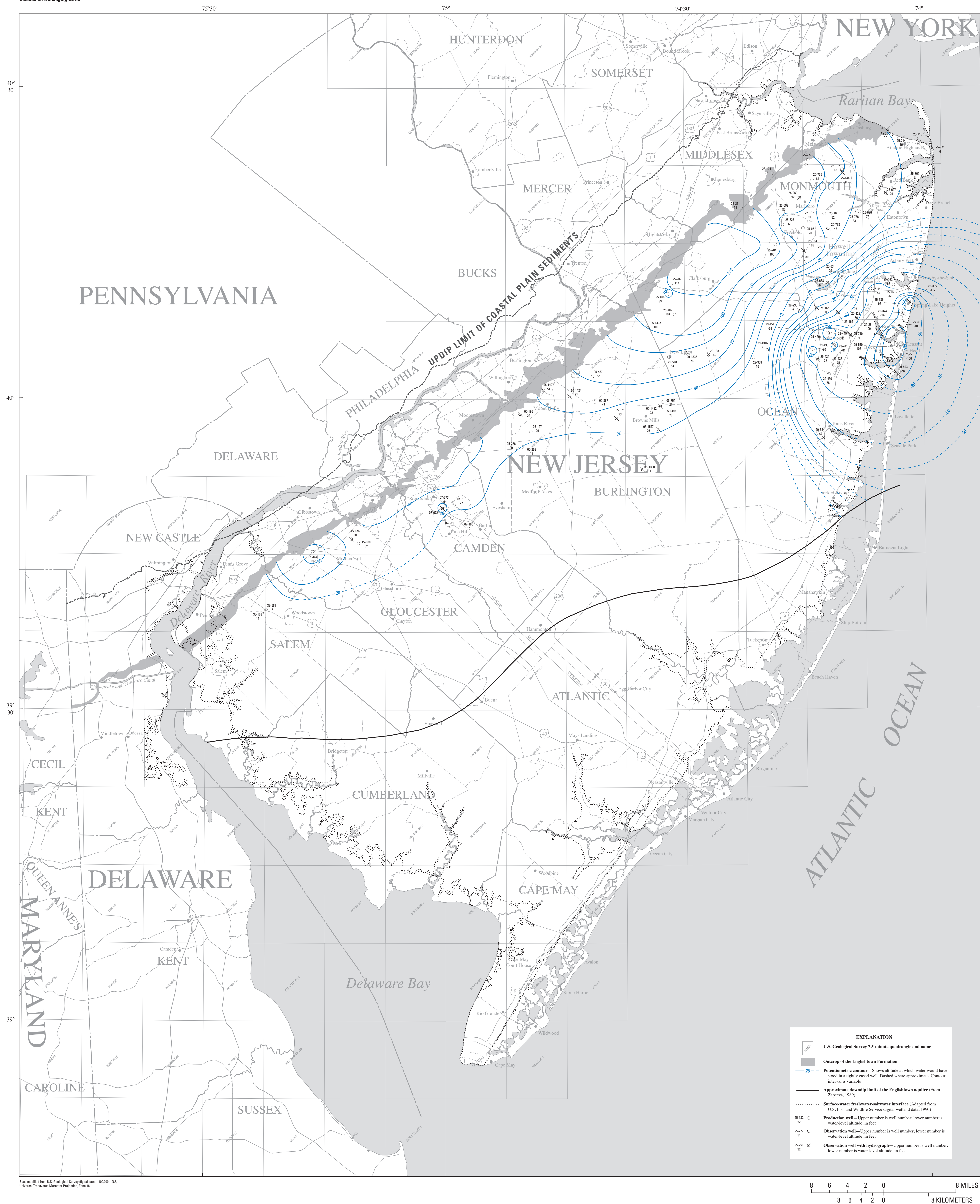
Potentiometric Surface of the Englishtown aquifer system, 2003
