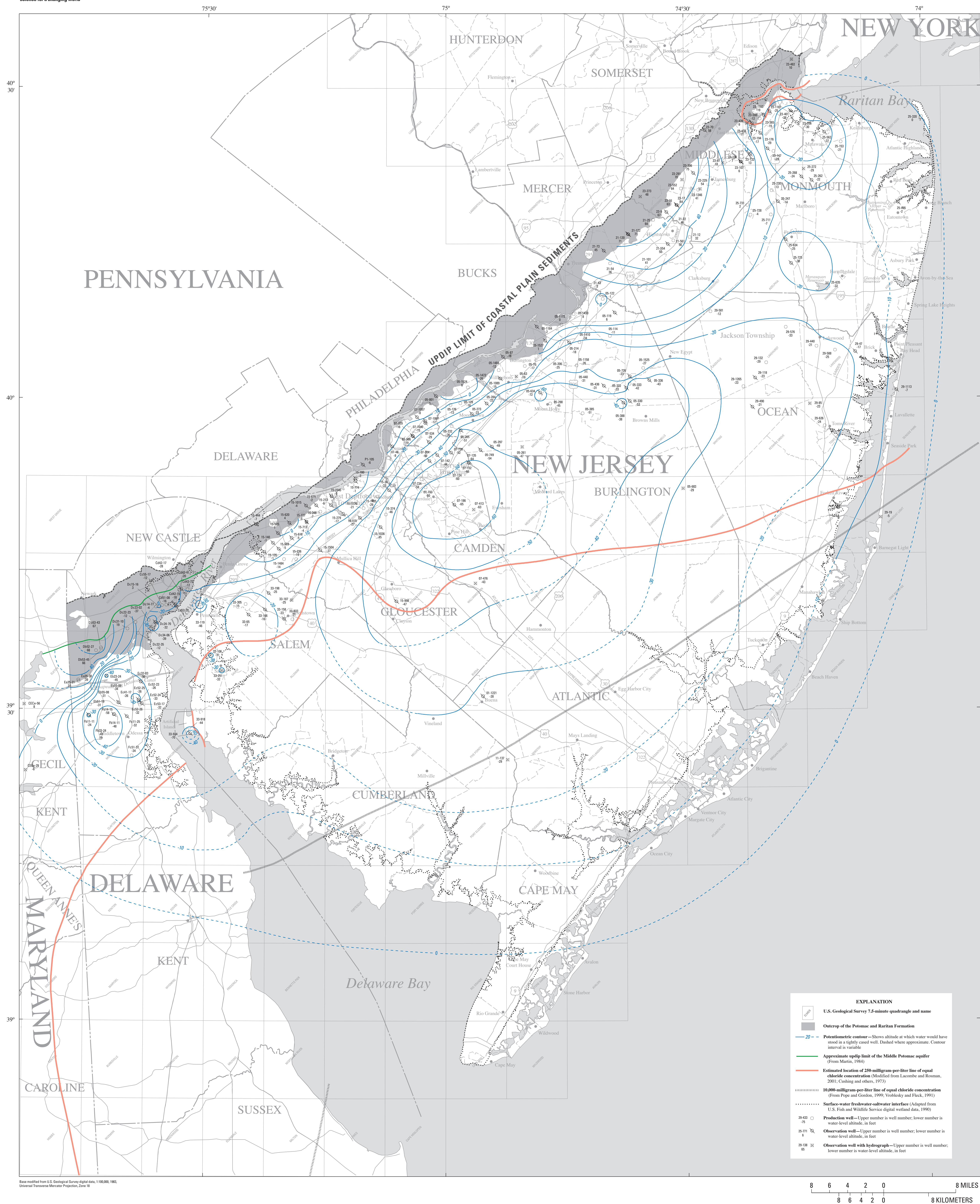
Potentiometric Surface of the Middle and undifferentiated Potomac-Raritan-Magothy aquifer, 2003
