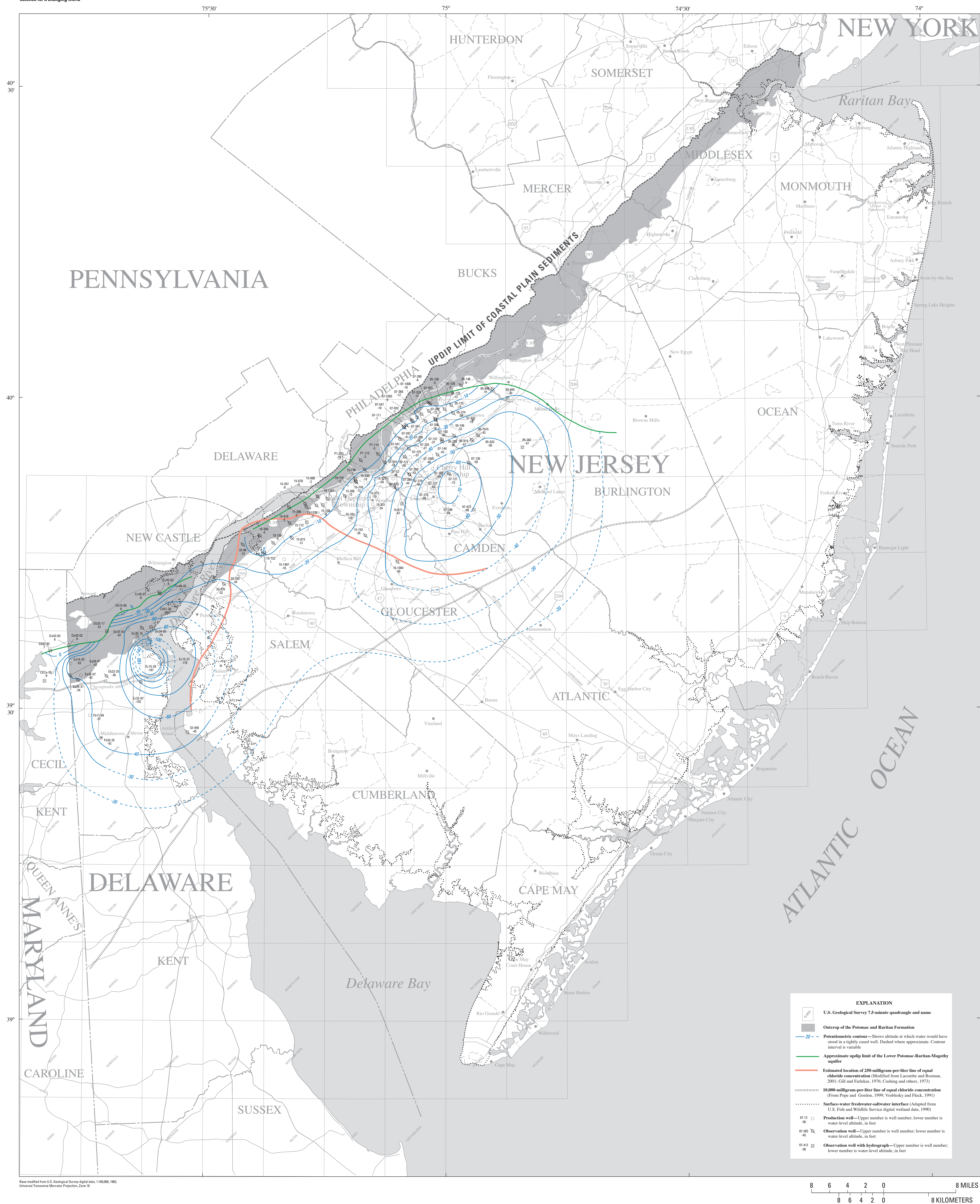
Potentiometric Surface of the Lower Potomac-Raritan-Magothy aquifer, 2003
