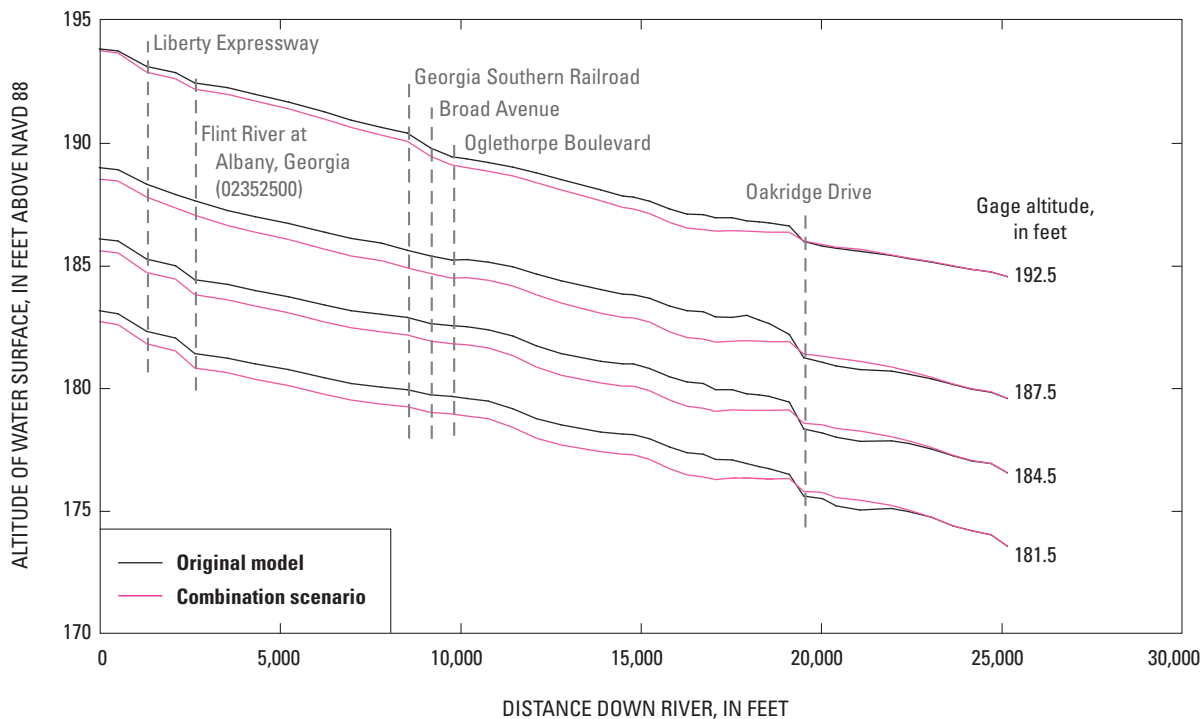
Figure 5. Simulated water surface profiles for the original model and the combination scenario for the Flint River at Albany, Georgia.
