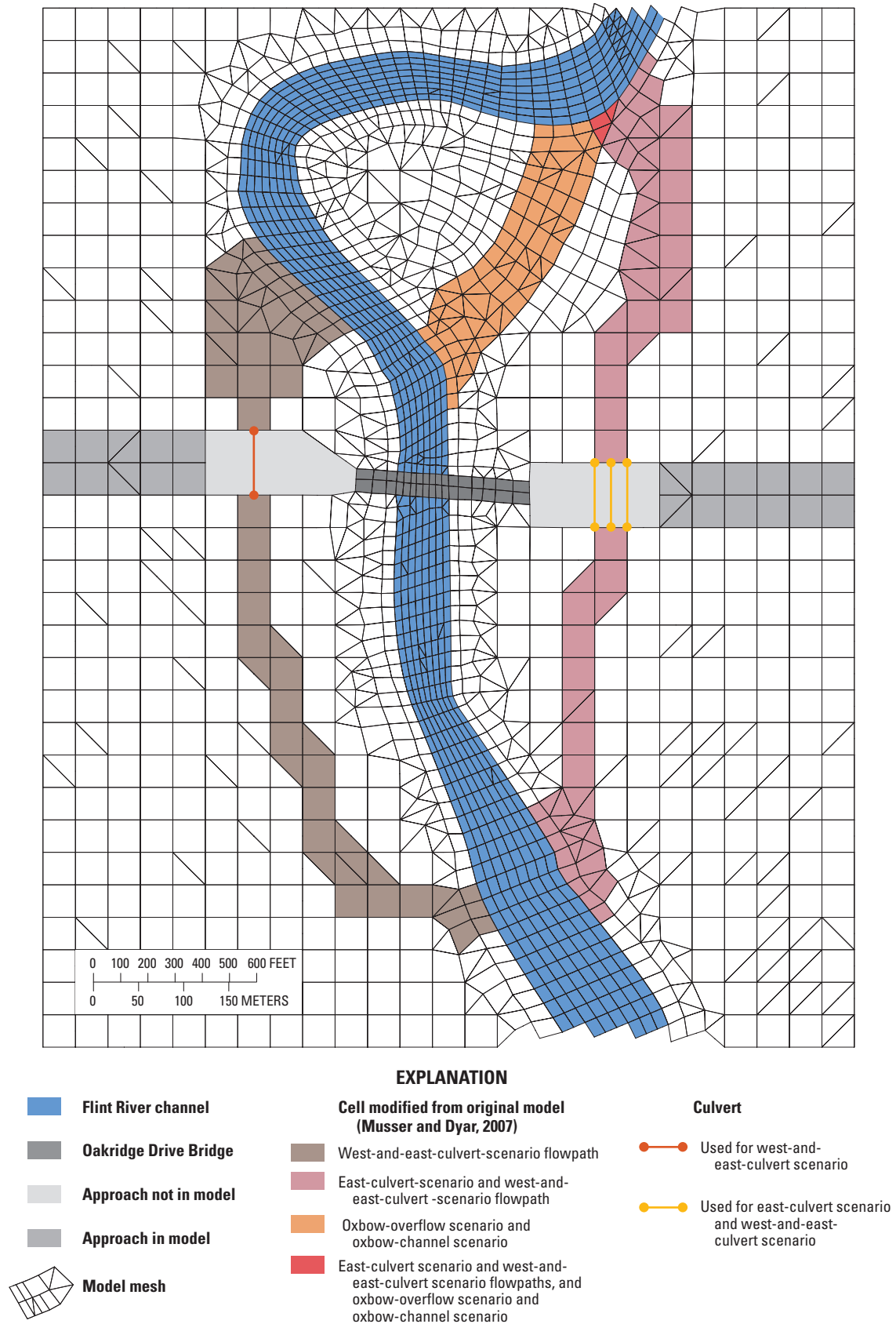
Figure 4. Cells modified from original finite-element mesh used for two-dimensional model of the Flint River at Albany, Georgia. Modified cells include west-and-east-culvert-scenario flowpath, east-culvert-scenario flowpath, oxbow-overflow scenario, and oxbow-channel scenario.
