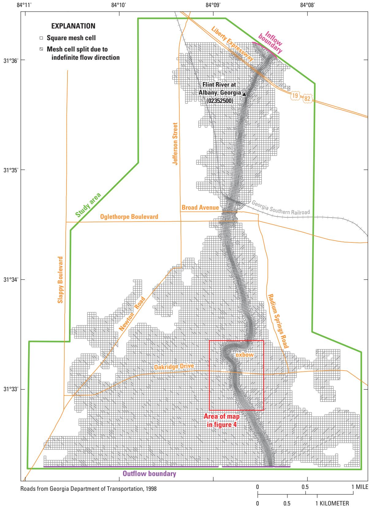
Figure 3. Original finite-element mesh used for two-dimensional model of the Flint River at Albany, Georgia. Inflow and outflow boundary conditions are for a water-surface altitude of 192.5 feet at the Albany streamgauge (modified from Musser and Dyar, 2007).
