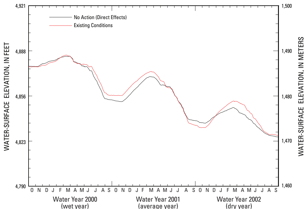
Figure 10. Comparison of water-surface elevations in Pueblo Reservoir for the Existing Conditions (water years 2000 through 2002) and No Action scenarios.
