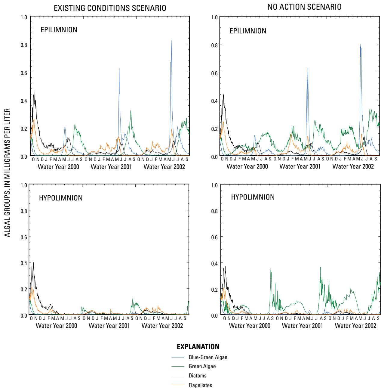
Figure 19. Relation between various algal groups in the epilimnion and hypolimnion at site 7B for the Existing Conditions (water years 2000 through 2002) and No Action (direct-effects analysis) scenarios.
