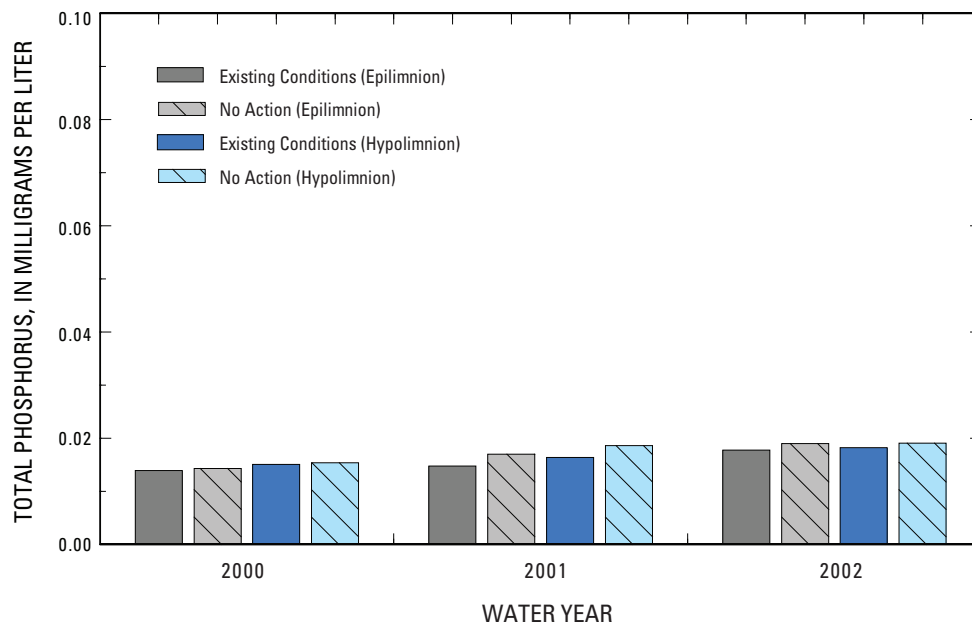
Figure 16. Annual median total-phosphorus concentrations in the epilimnion and hypolimnion at site 7B for the Existing Conditions (water years 2000 through 2002) and No Action (direct-effects analysis) scenarios.
