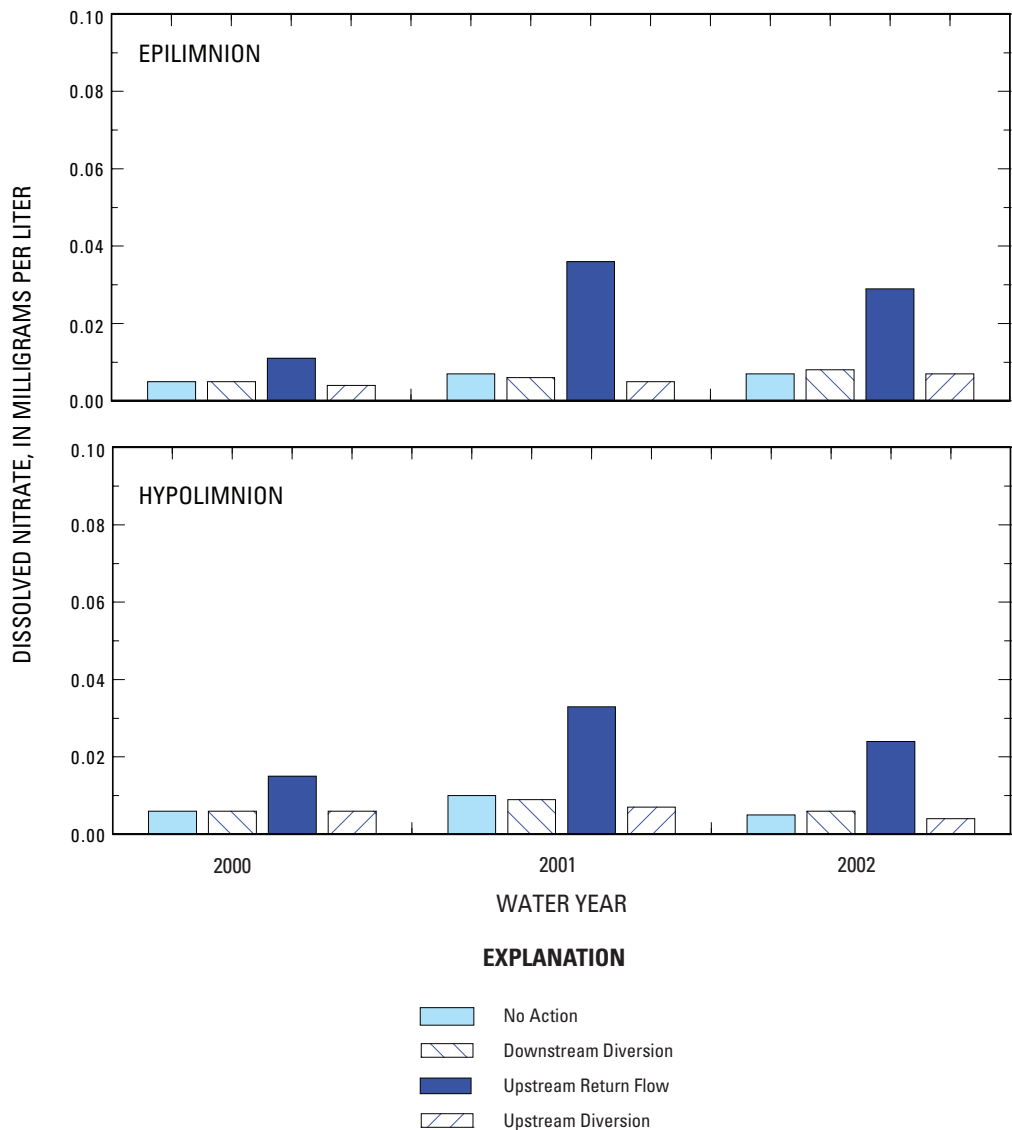
Figure 27. Annual median dissolved-nitrate concentrations in the epilimnion and hypolimnion at site 7B for the No Action, Downstream Diversion, Upstream Return-Flow, and Upstream Diversion scenarios (direct-effects analyses).
