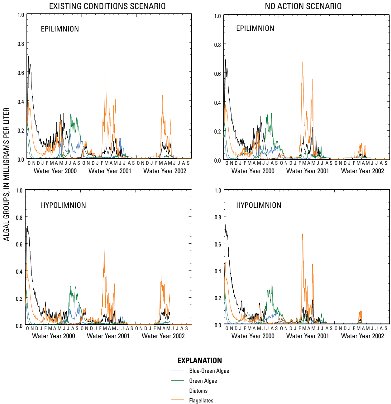
Figure 20. Relation between various algal groups in the epilimnion and hypolimnion at site 3B for the Existing Conditions (water years 2000 through 2002) and No Action (direct-effects analysis) scenarios.
