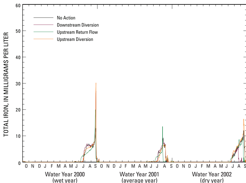
Figure 30. Comparison of total-iron concentrations in the hypolimnion at site 7B in Pueblo Reservoir for the No Action, Downstream Diversion, Upstream Return-Flow, and Upstream Diversion scenarios (direct-effects analyses).
