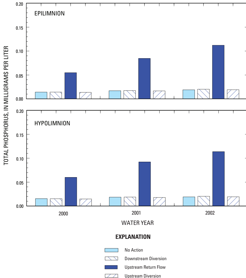
Figure 28. Annual median total-phosphorus concentrations in the epilimnion and hypolimnion at site 7B for the No Action, Downstream Diversion, Upstream Return-Flow, and Upstream Diversion scenarios (direct-effects analyses).
