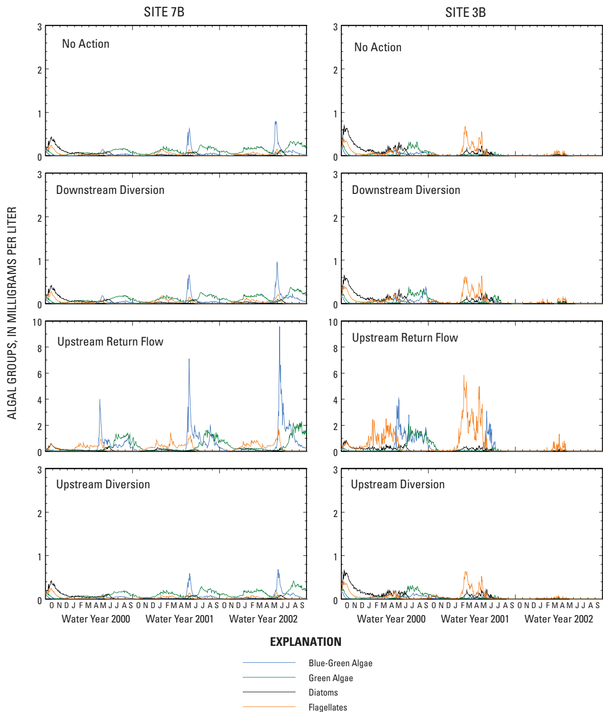
Figure 31. Relation between various algal groups in the epilimnion at sites 7B and 3B for the No Action, Downstream Diversion, Upstream Return-Flow, and Upstream Diversion scenarios (direct-effects analyses). Note scales for y-axis of Upstream Return-Flow scenario are different from the other scenarios.
