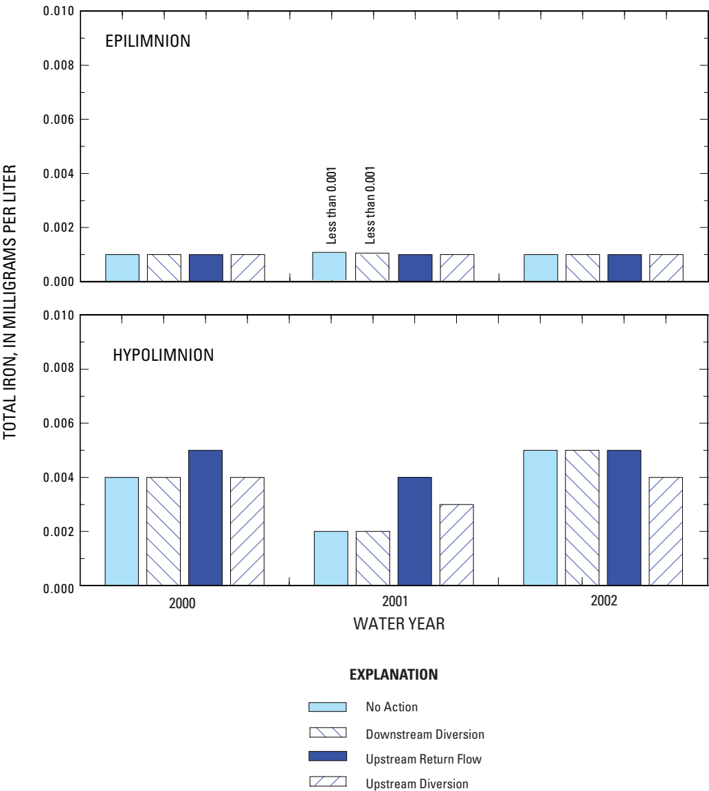
Figure 29. Annual median total-iron concentrations in the epilimnion and hypolimnion at site 7B for the No Action, Downstream Diversion, Upstream Return-Flow, and Upstream Diversion scenarios (direct-effects analyses).
