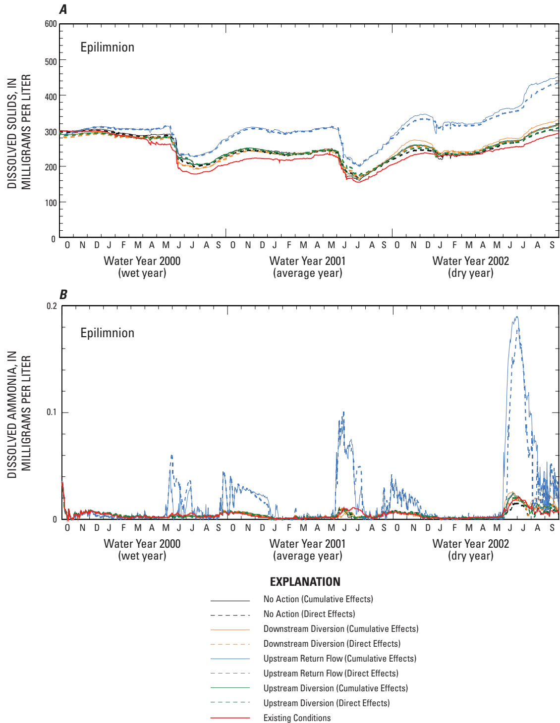
Figure 9. Comparison of dissolved-solids and dissolved-ammonia concentrations at site 7B in Pueblo Reservoir for the Existing Conditions scenario (water years 2000 through 2002) and cumulative- and direct-effects analyses for selected simulation scenarios.
