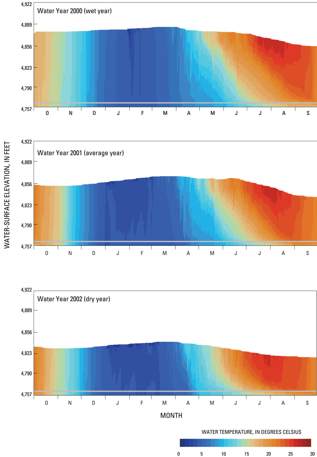
Figure 5. Simulated water temperature at site 7B near the dam for the No Action scenario, water years 2000 through 2002. Gray line represents approximate elevation of Arkansas outlet.
