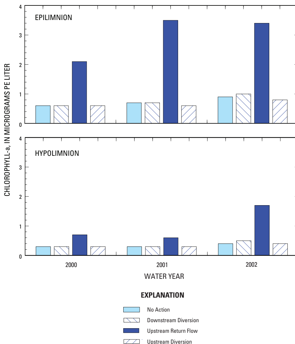
Figure 32. Annual median chlorophyll- a concentrations in the epilimnion and hypolimnion at site 7B for the No Action, Downstream Diversion, Upstream Return-Flow, and Upstream Diversion scenarios (direct-effects analyses).
