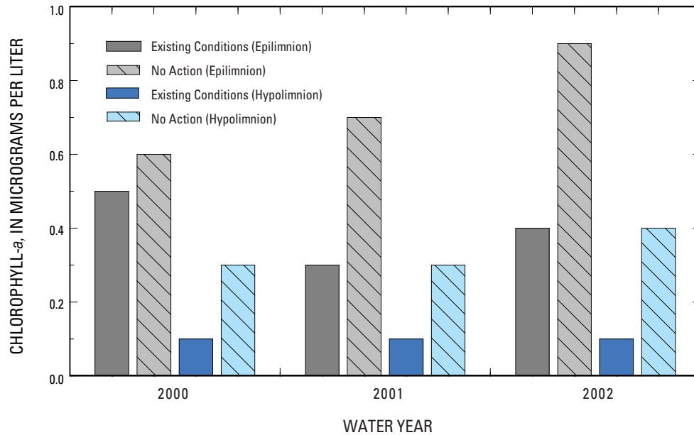
Figure 21. Annual median chlorophyll- a concentrations in the epilimnion and hypolimnion at site 7B for the Existing Conditions (water years 2000 through 2002) and No Action (direct-effects analysis) scenarios.
