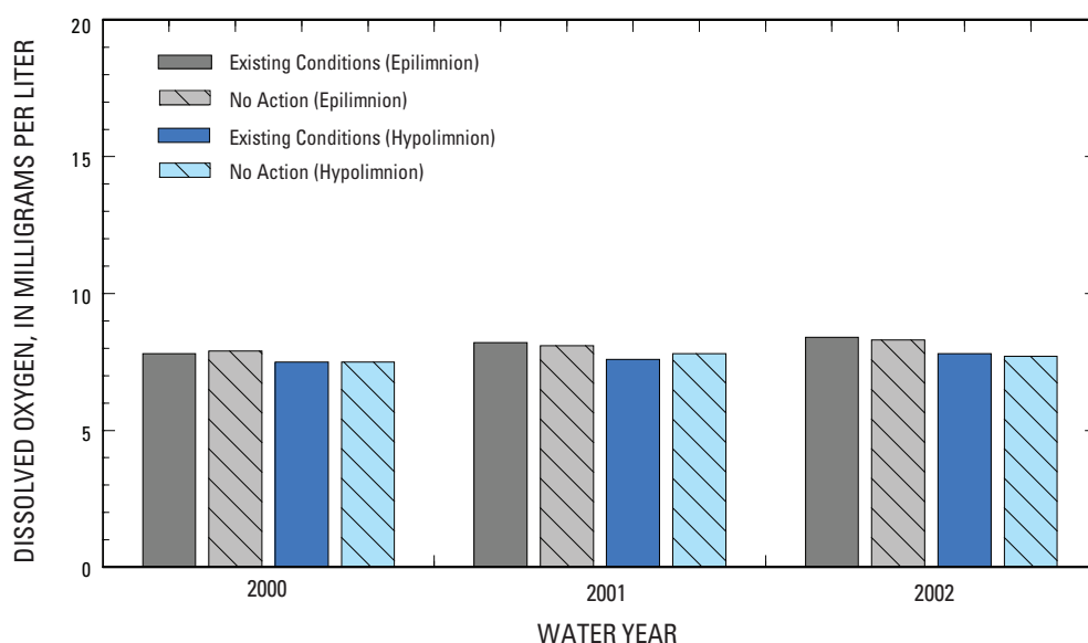
Figure 12. Annual median dissolved-oxygen concentrations in the epilimnion and hypolimnion at site 7B for the Existing Conditions (water years 2000 through 2002) and No Action (direct-effects analysis) scenarios.
