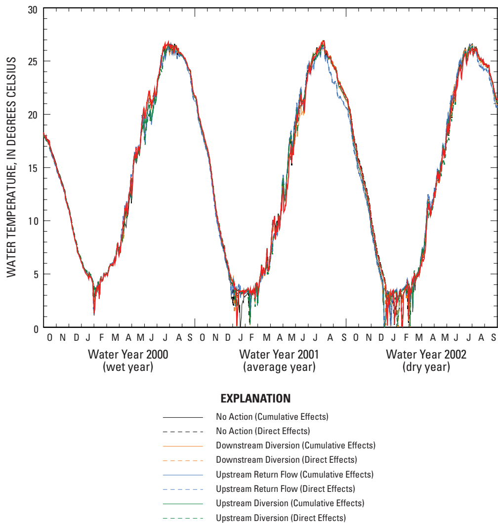
Figure 6. Comparison of water temperatures at site 7B in Pueblo Reservoir for the Existing Conditions scenario (water years 2000 through 2002) and cumulative- and direct-analyses for selected simulation scenarios.
