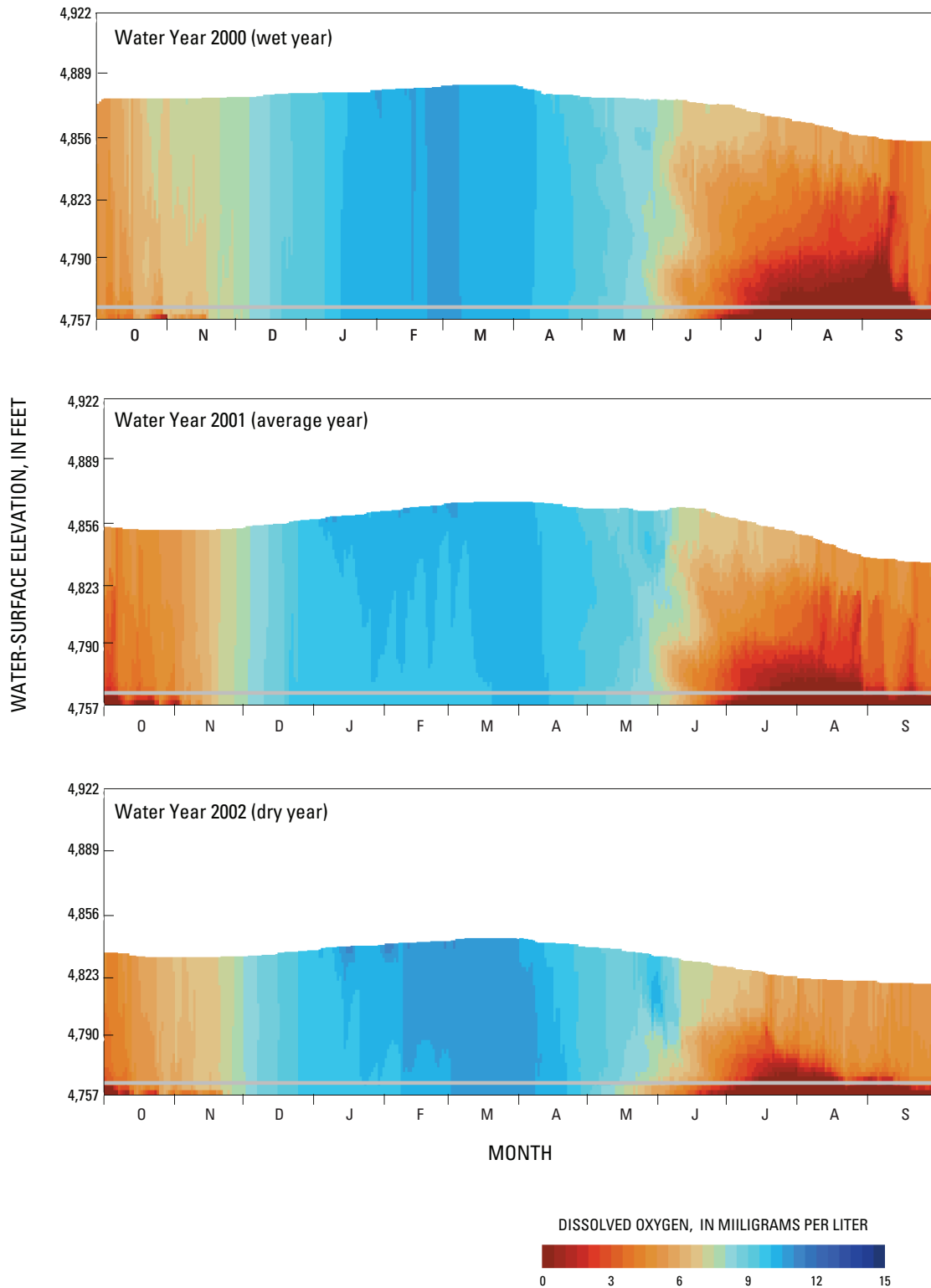
Figure 7. Simulated dissolved-oxygen concentrations at site 7B near the dam for the No Action (direct-effects analysis) scenario. Gray line represents approximate elevation of Arkansas outlet.
