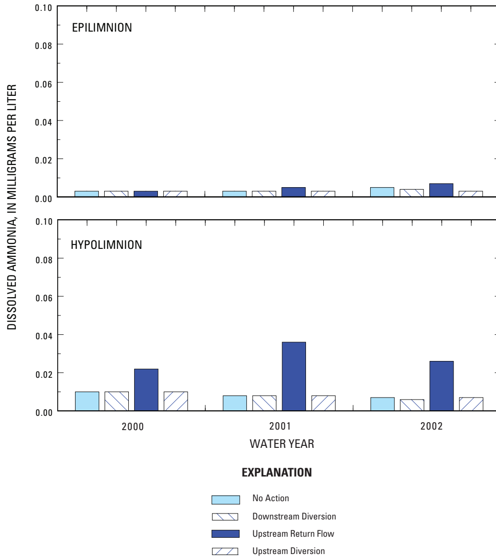
Figure 26. Annual median dissolved-ammonia concentrations in the epilimnion and hypolimnion at site 7B for the No Action, Downstream Diversion, Upstream Return-Flow, and Upstream Diversion scenarios (direct-effects analyses).
