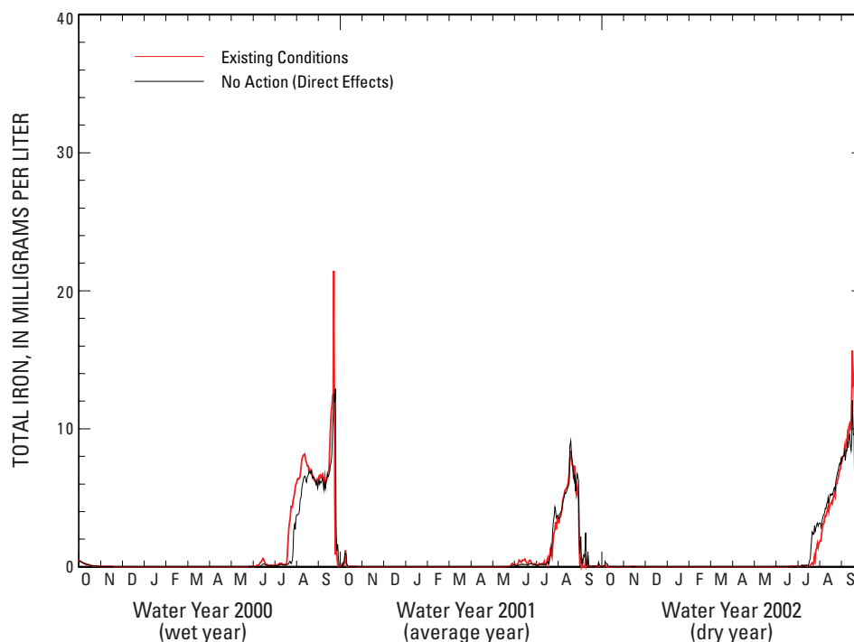
Figure 18. Comparison of total-iron concentrations in the hypolimnion at site 7B in Pueblo Reservoir for the Existing Conditions (water years 2000 through 2002) and No Action (direct-effects analysis) scenarios.
