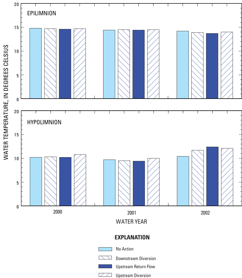
Figure 23. Annual median water temperature in the epilimnion and hypolimnion at site 7B for the No Action, Downstream Diversion, Upstream Return-Flow, and Upstream Diversion scenarios (direct-effects analyses).
