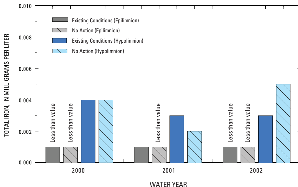
Figure 17. Annual median total-iron concentrations in the epilimnion and hypolimnion at site 7B for the Existing Conditions (water years 2000 through 2002) and No Action (direct-effects analysis) scenarios.
