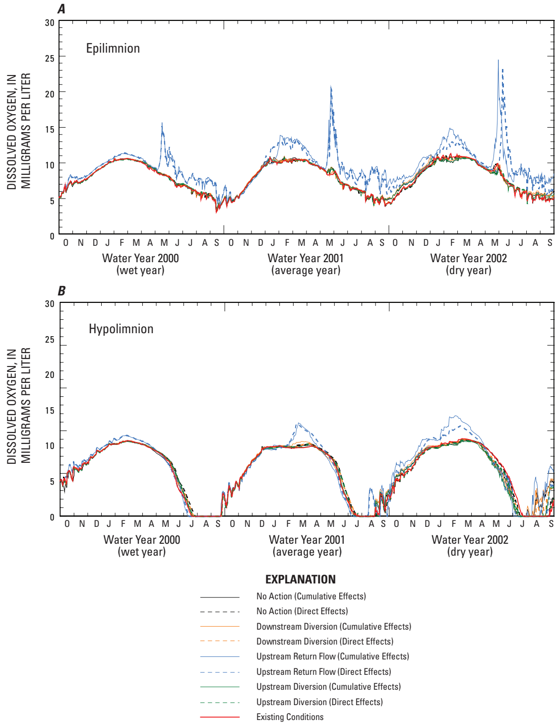
Figure 8. Comparison of dissolved-oxygen concentrations at site 7B in Pueblo Reservoir for the Existing Conditions scenario (water years 2000 through 2002) and cumulative- and direct-effects analyses for selected simulation scenarios.
