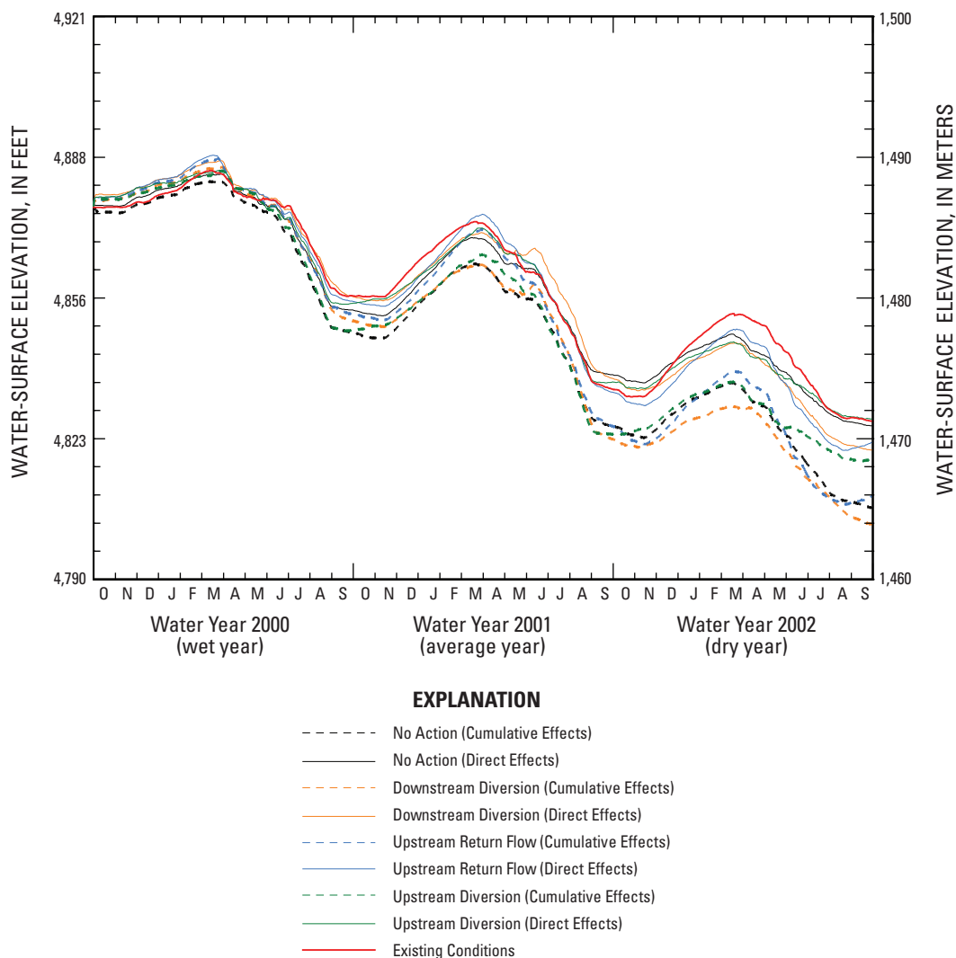
Figure 4. Comparison of water-surface elevations in Pueblo Reservoir for the Existing Conditions scenario (water years 2000 through 2002) and cumulative- and direct-effects analyses for selected simulation scenarios.
