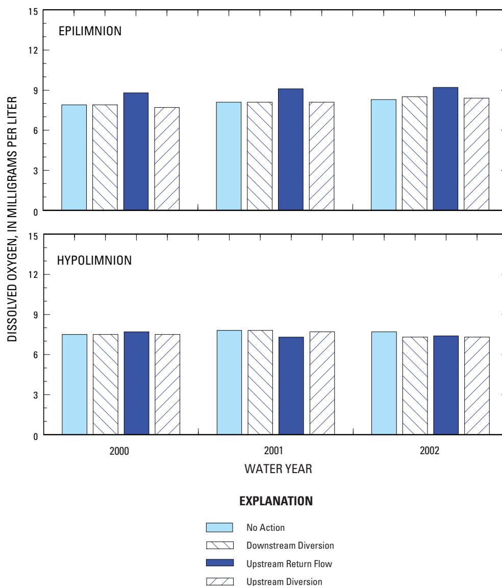
Figure 24. Annual median dissolved-oxygen concentrations in the epilimnion and hypolimnion at site 7B for the No Action, Downstream Diversion, Upstream Return-Flow, and Upstream Diversion scenarios (direct-effects analyses).
