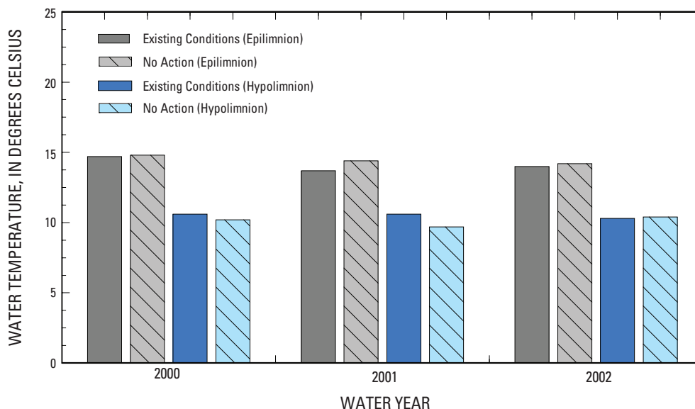
Figure 11. Annual median water temperature in the epilimnion and hypolimnion at site 7B for the Existing Conditions (water years 2000 through 2002) and No Action (direct-effects analysis) scenarios.
