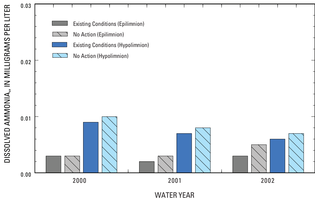
Figure 14. Annual median dissolved-ammonia concentrations in the epilimnion and hypolimnion at site 7B for the Existing Conditions (water years 2000 through 2002) and No Action (direct-effects analysis) scenarios.
