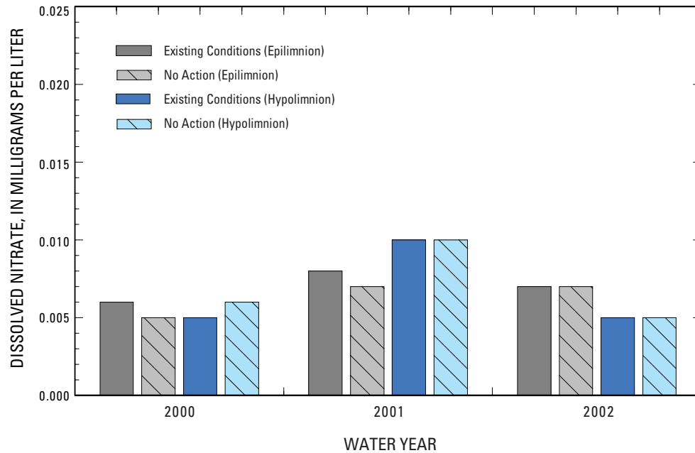
Figure 15. Annual median dissolved-nitrate concentrations in the epilimnion and hypolimnion at site 7B for the Existing Conditions (water years 2000 through 2002) and No Action (direct-effects analysis) scenarios.
