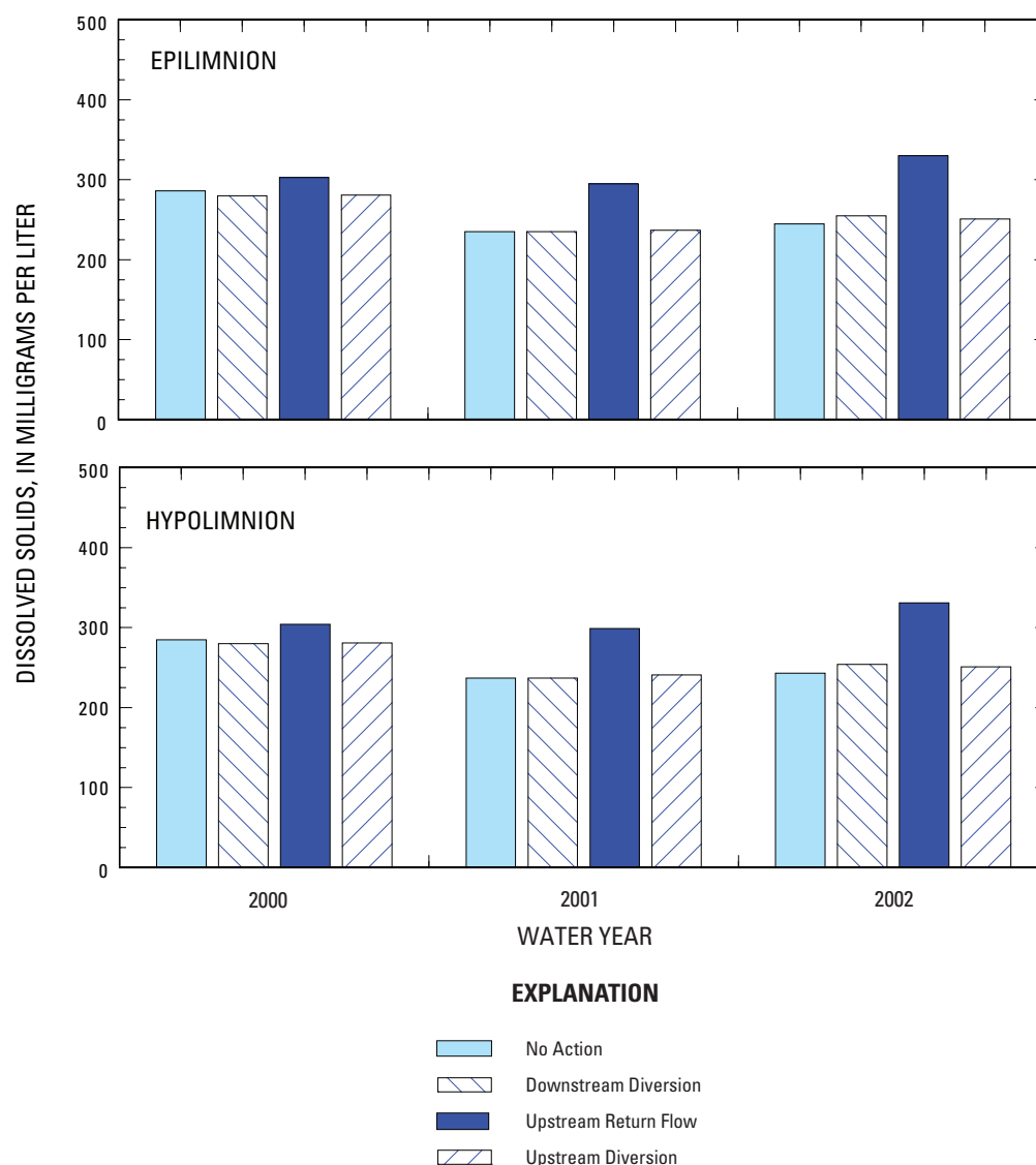
Figure 25. Annual median dissolved-solids concentrations in the epilimnion and hypolimnion at site 7B for the No Action, Downstream Diversion, Upstream Return-Flow, and Upstream Diversion scenarios (direct-effects analyses).
