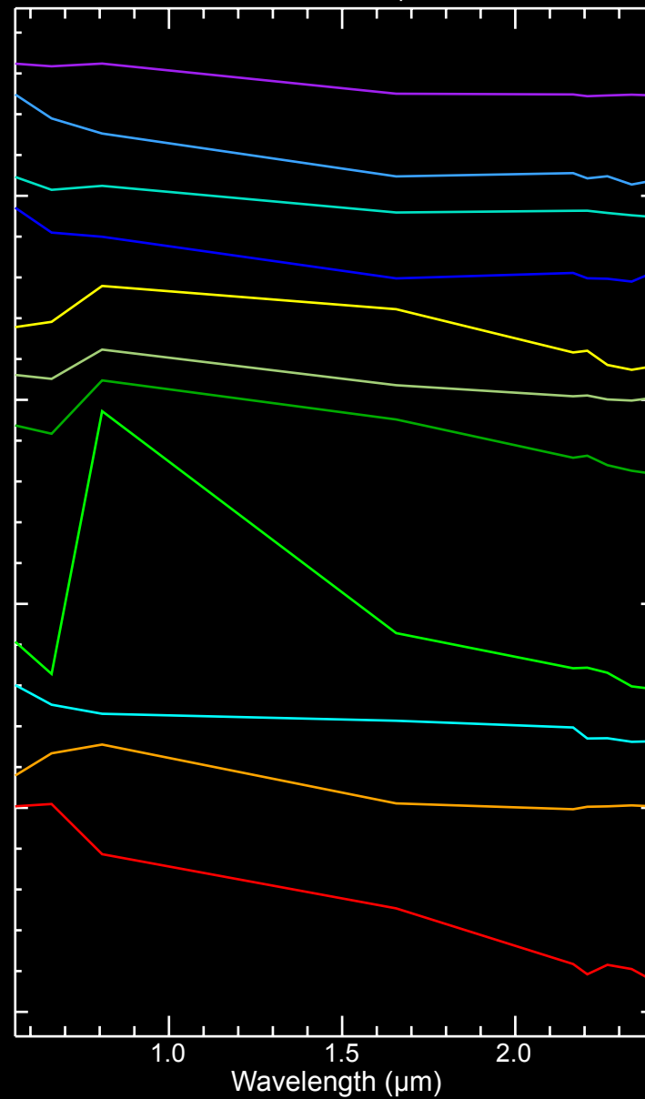
Identified ASTER Spectra
