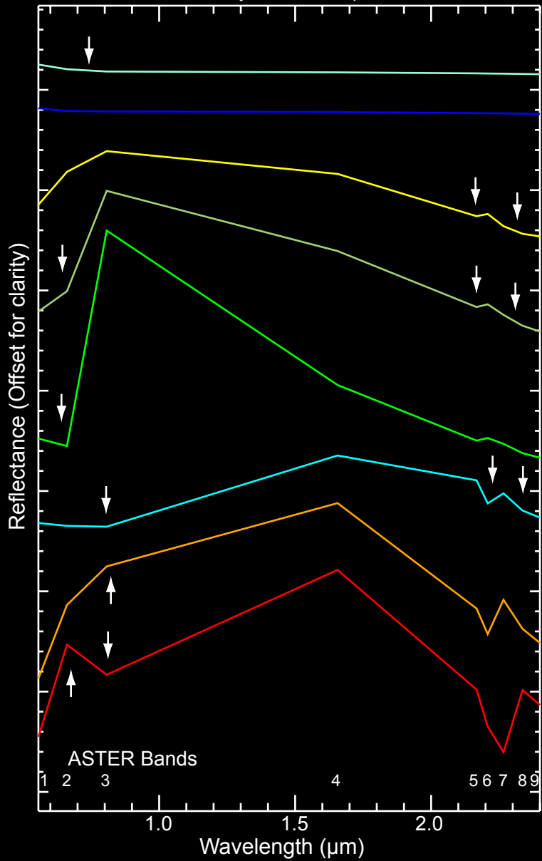
Laboratory Reference Spectra
