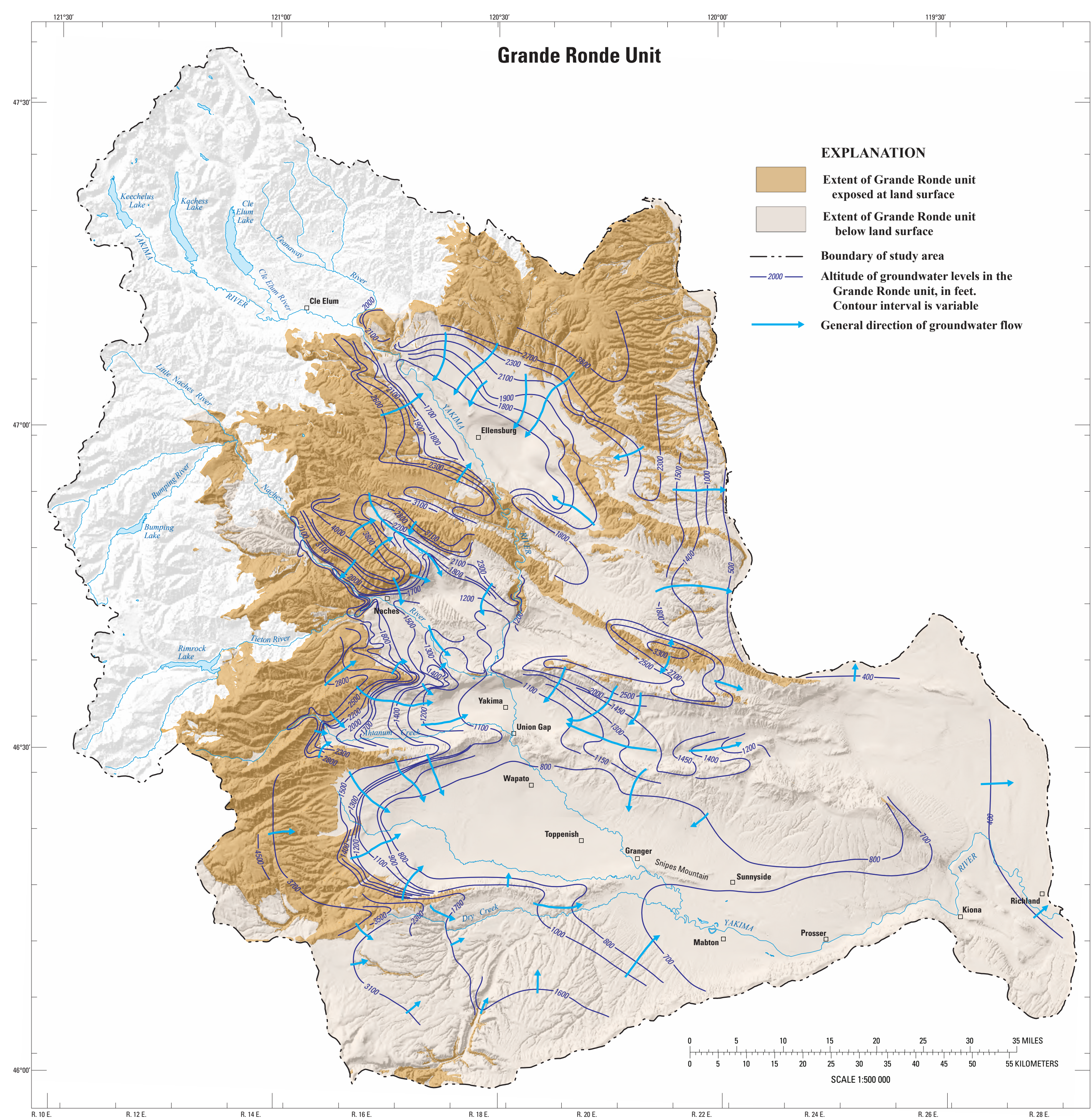
Maps Showing Generalized Altitude of Groundwater Levels for the Saddle Mountains, Wanapum, and Grande Ronde Units, Approximating Spring 2001 Conditions, Yakima River Basin Aquifer System, Washington
