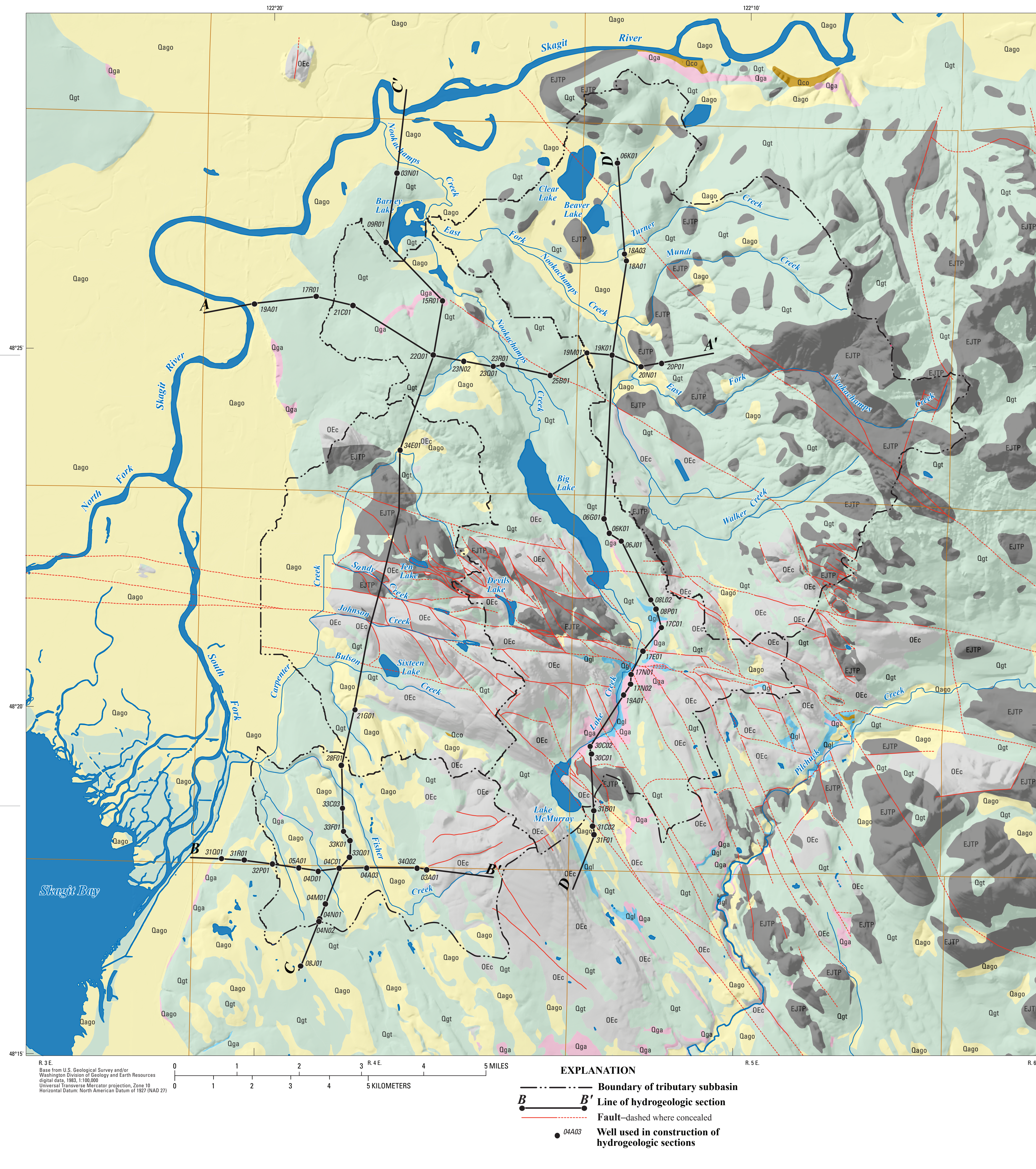
Map and Hydrogeologic Sections Showing Surficial Hydrogeology, Hydrogeologic Units, and Locations of Selected Wells in Tributary Subbasins and Vicinity, Lower Skagit River Basin, Washington
