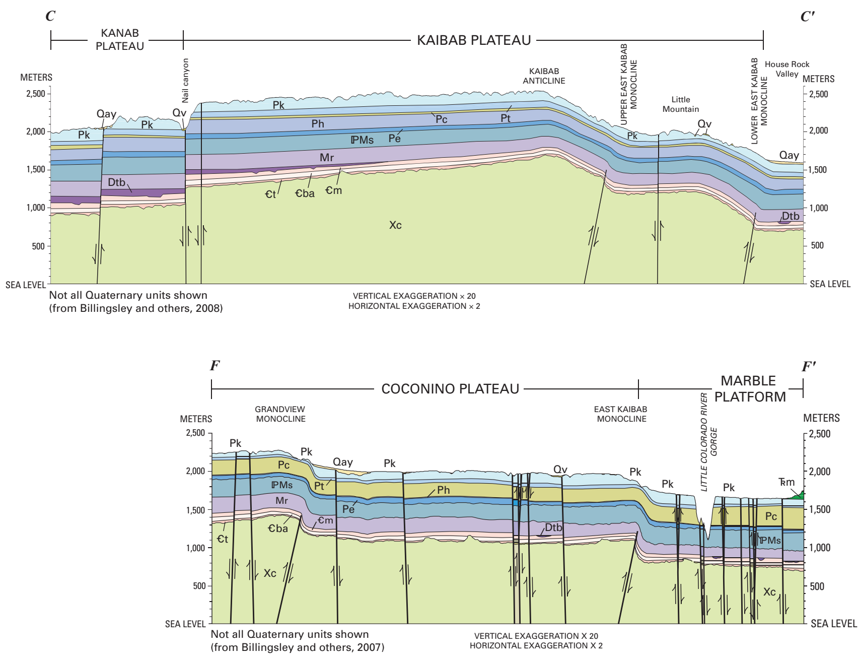
MAP SHOWING GEOLOGIC STRUCTURE, CULTURAL AND GEOGRAPHIC FEATURES, AND GEOLOGIC CROSS SECTIONS OF NORTHWESTERN ARIZONA
