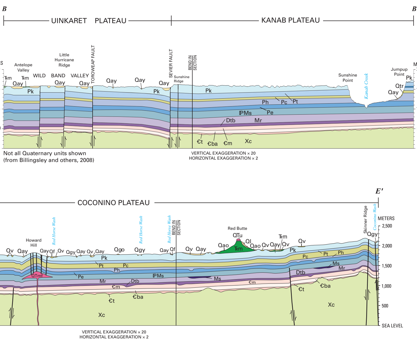
MAP SHOWING GEOLOGIC STRUCTURE, CULTURAL AND GEOGRAPHIC FEATURES, AND GEOLOGIC CROSS SECTIONS OF NORTHWESTERN ARIZONA
