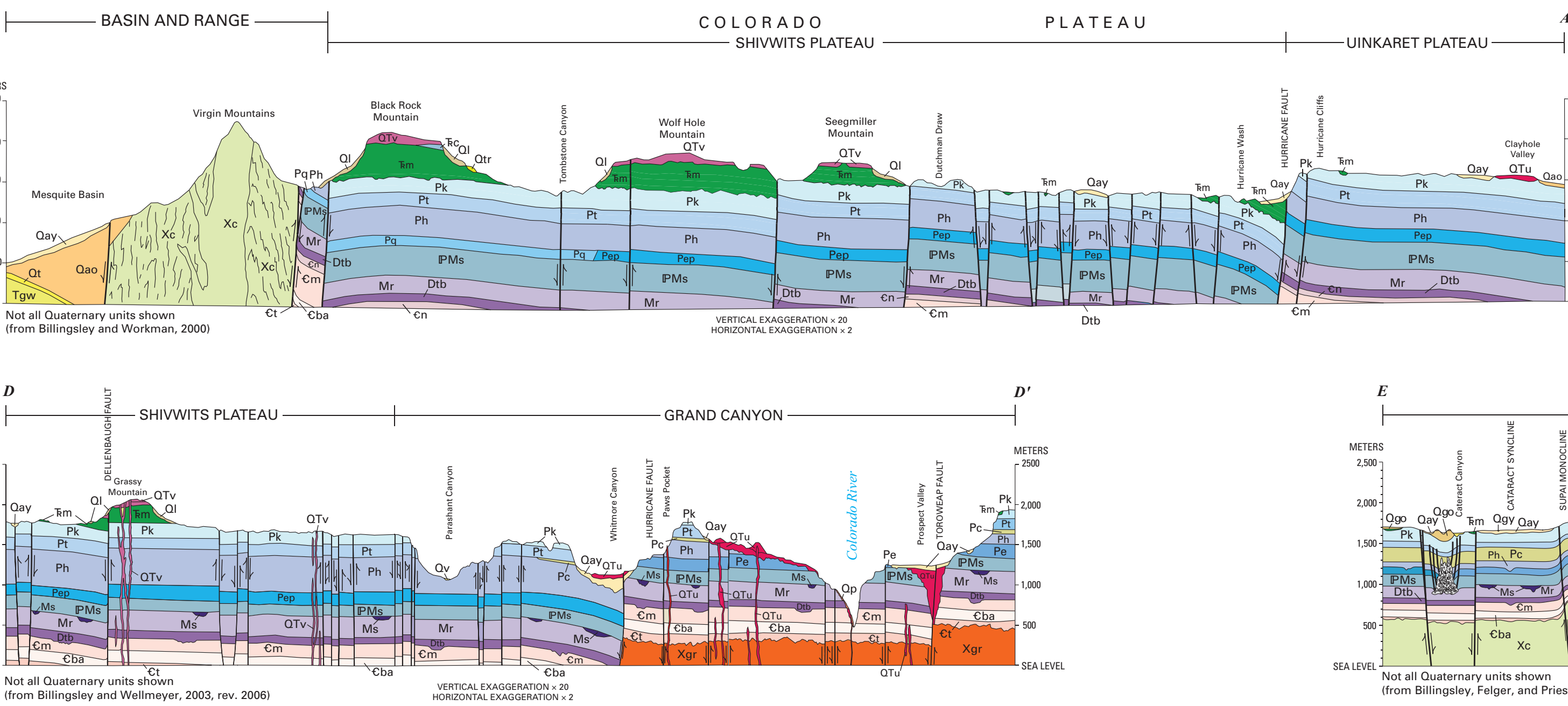
MAP SHOWING GEOLOGIC STRUCTURE, CULTURAL AND GEOGRAPHIC FEATURES, AND GEOLOGIC CROSS SECTIONS OF NORTHWESTERN ARIZONA
