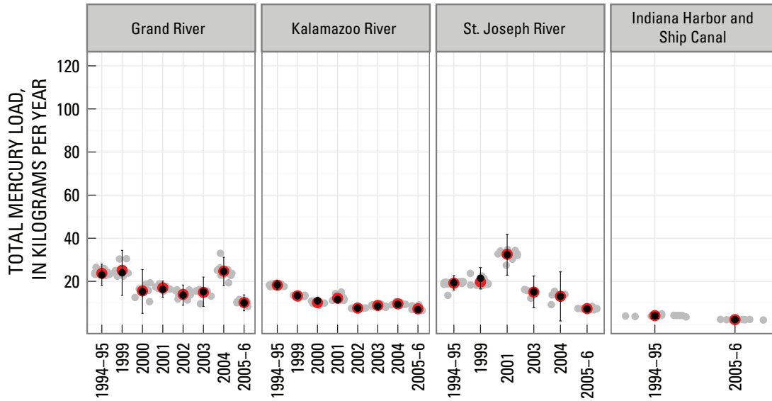
Figure 10. Calculated mercury loads at four Lake Michigan tributary monitoring sites.
