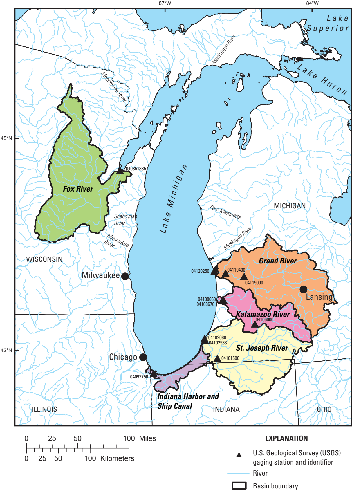
Figure 1. Location of tributary sampling sites for the Lake Michigan Tributary Monitoring Project. USGS gaging stations are described in table 2.
