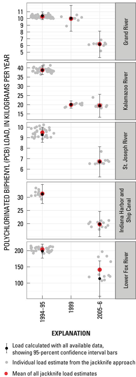
Figure 13. Calculated polychlorinated biphenyl (PCB) loads at five Lake Michigan tributary monitoring sites.
