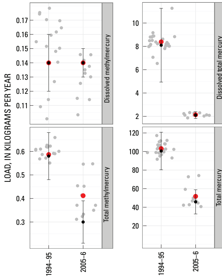
Figure 11. Calculated mercury loads at the Fox River tributary monitoring site.
