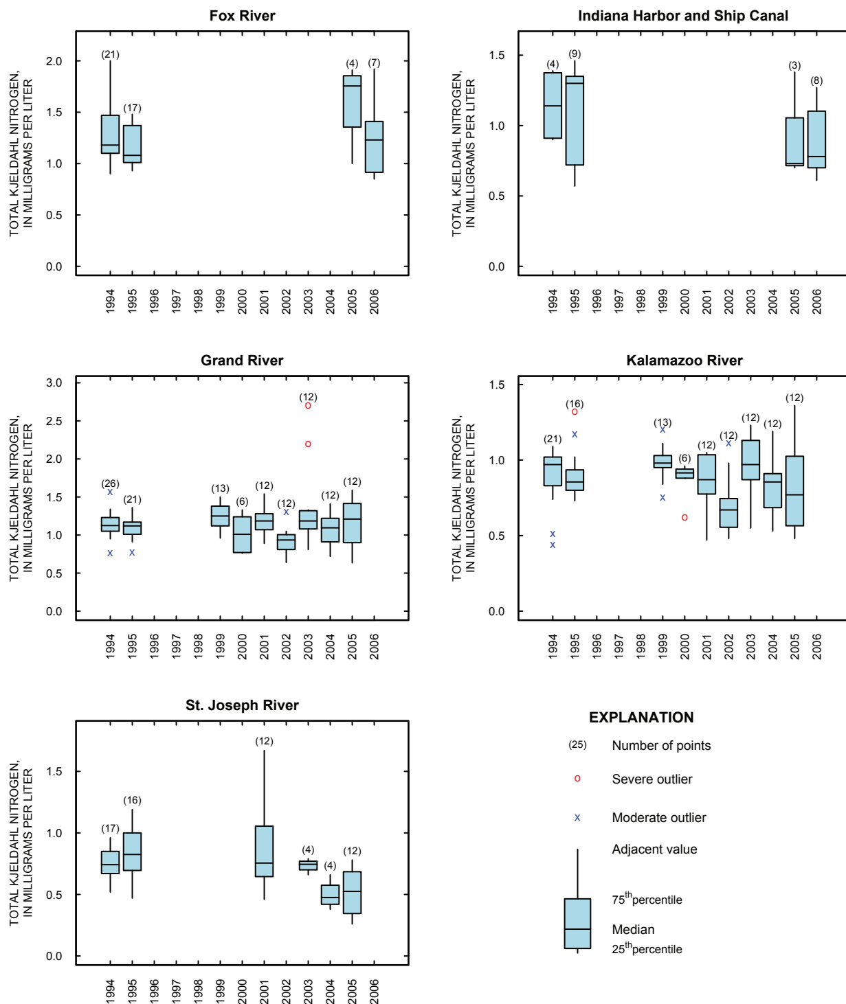
Figure 4-2. Concentrations of total Kjeldahl nitrogen at five Lake Michigan tributary monitoring sites, 1994–2006.
