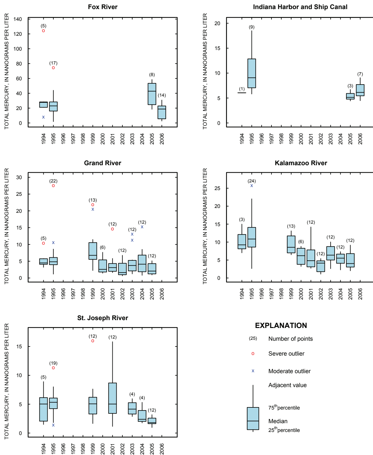
Figure 9. Total mercury concentrations at five Lake Michigan tributary monitoring sites, 1994–2006. (Note differences in y-axis scales among the plots.)
