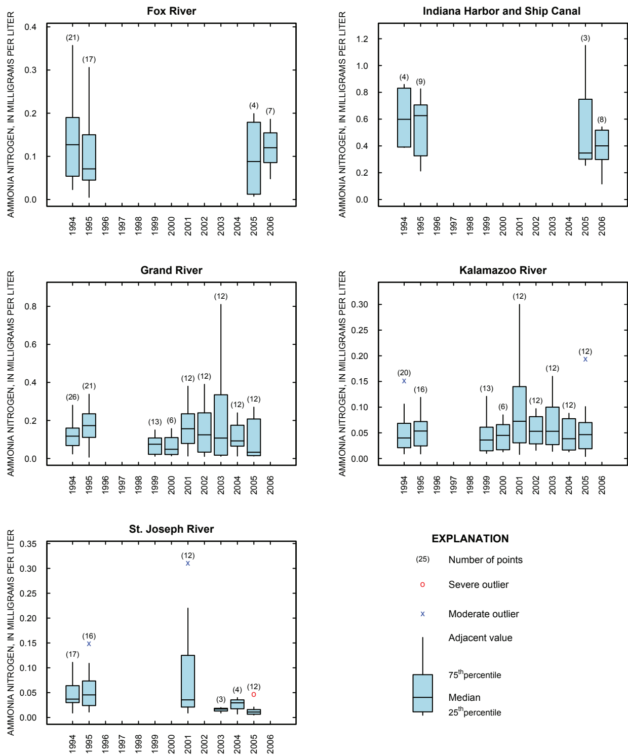
Figure 4–1. Concentrations of ammonia nitrogen at five Lake Michigan tributary monitoring sites, 1994–2006.
