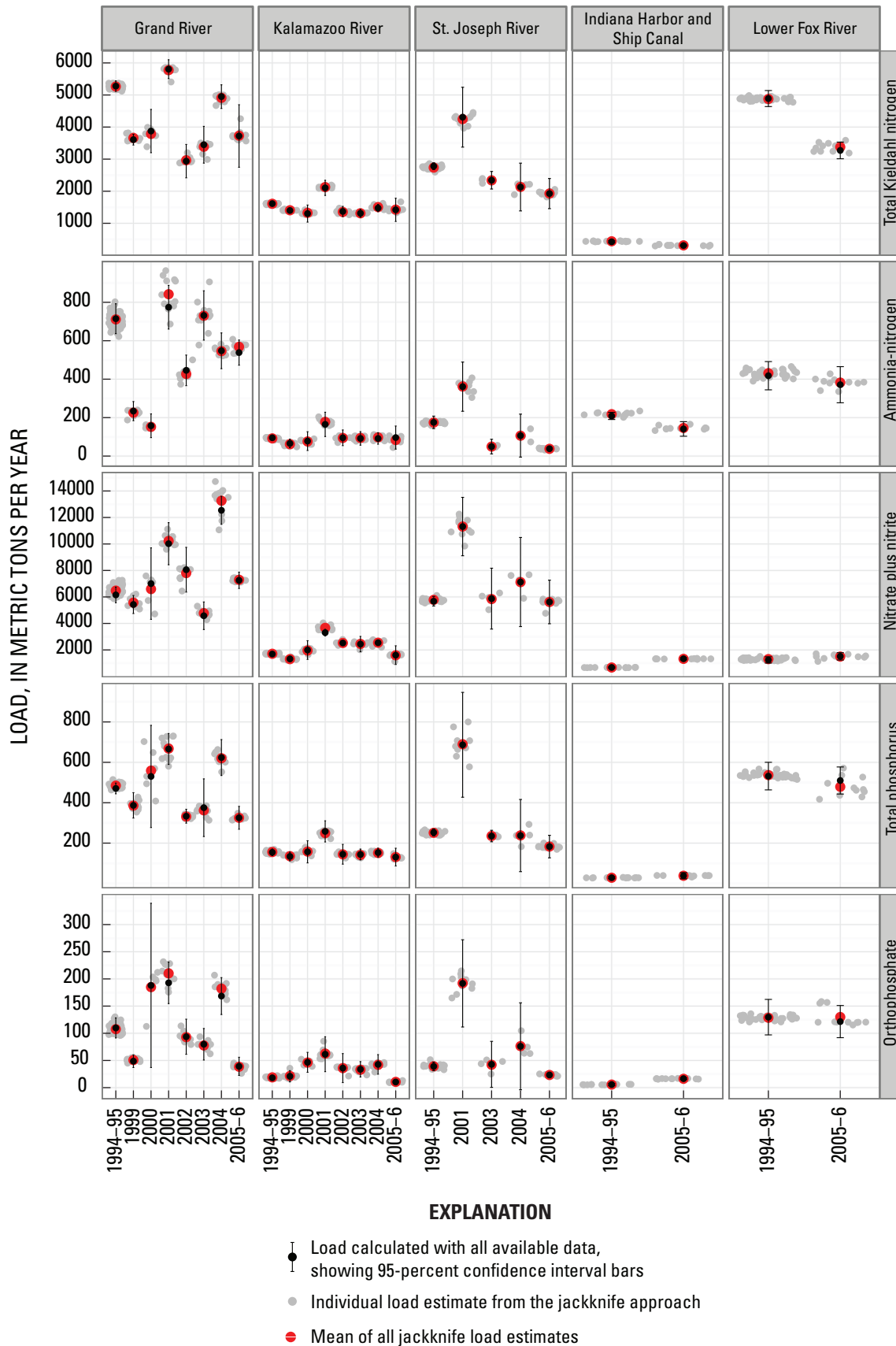
Figure 8. Calculated nutrient loads at five Lake Michigan tributary monitoring sites. (Note differences in y-axis scales among the plots.)
