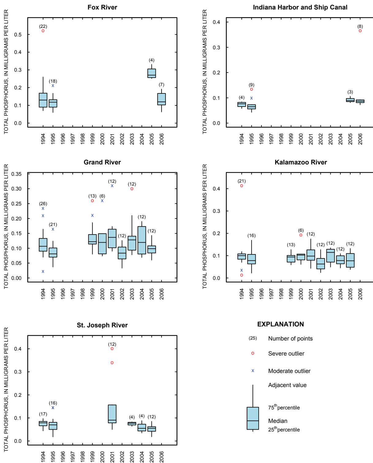
Figure 5. Total phosphorus concentrations at five Lake Michigan tributary monitoring sites, 1994–2006. (Note differences in y-axis scales among the plots.)
