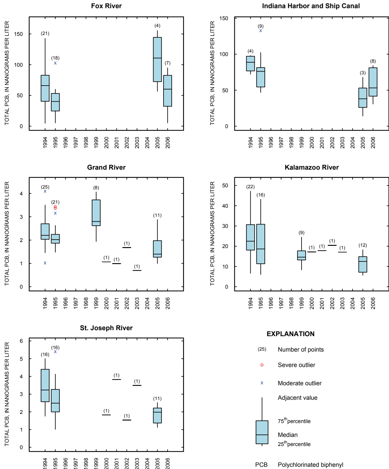
Figure 12. Total polychlorinated biphenyl (PCB) concentrations at five Lake Michigan tributary monitoring sites, 1994–2006.
