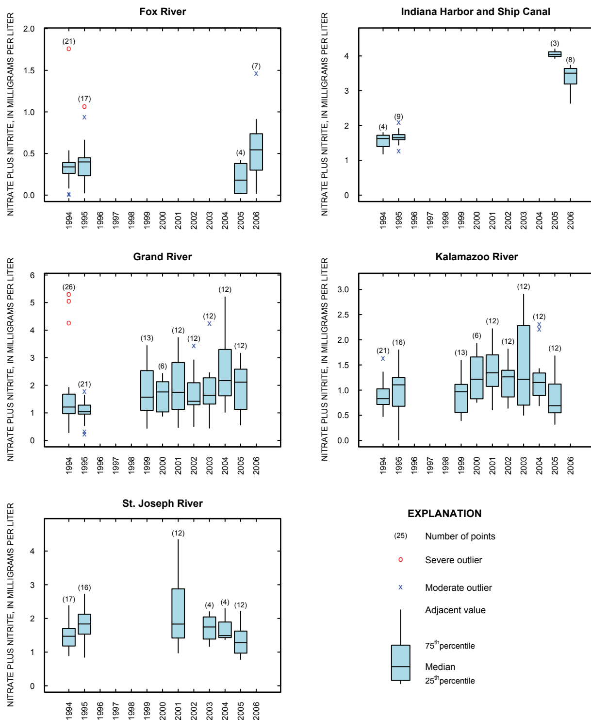
Figure 7. Nitrate plus nitrite concentrations at five Lake Michigan tributary monitoring sites, 1994–2006. (Note differences in y-axis scales among the plots.)
