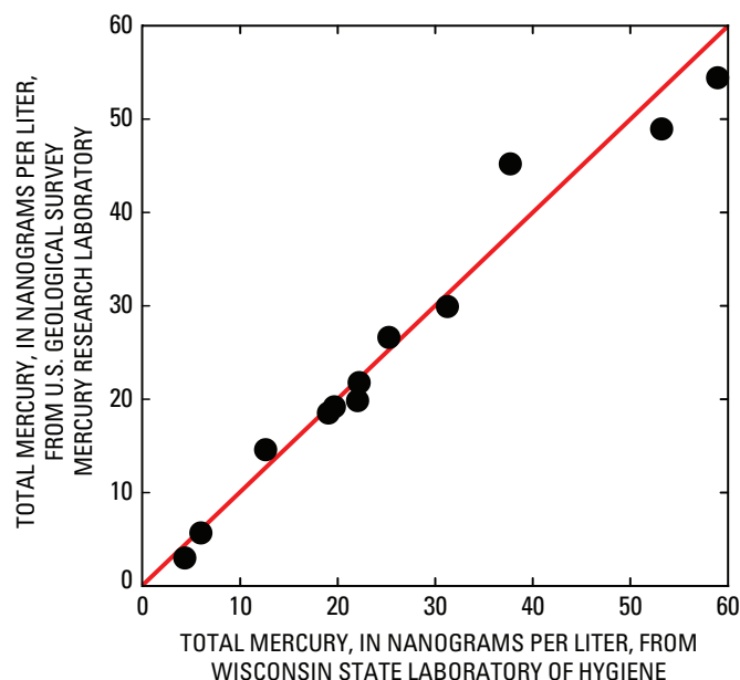
Figure 3. Comparison of total mercury analyses between the Wisconsin State Laboratory of Hygiene and the U.S. Geological Survey Mercury Research Laboratory. Red line is the line of perfect agreement.
