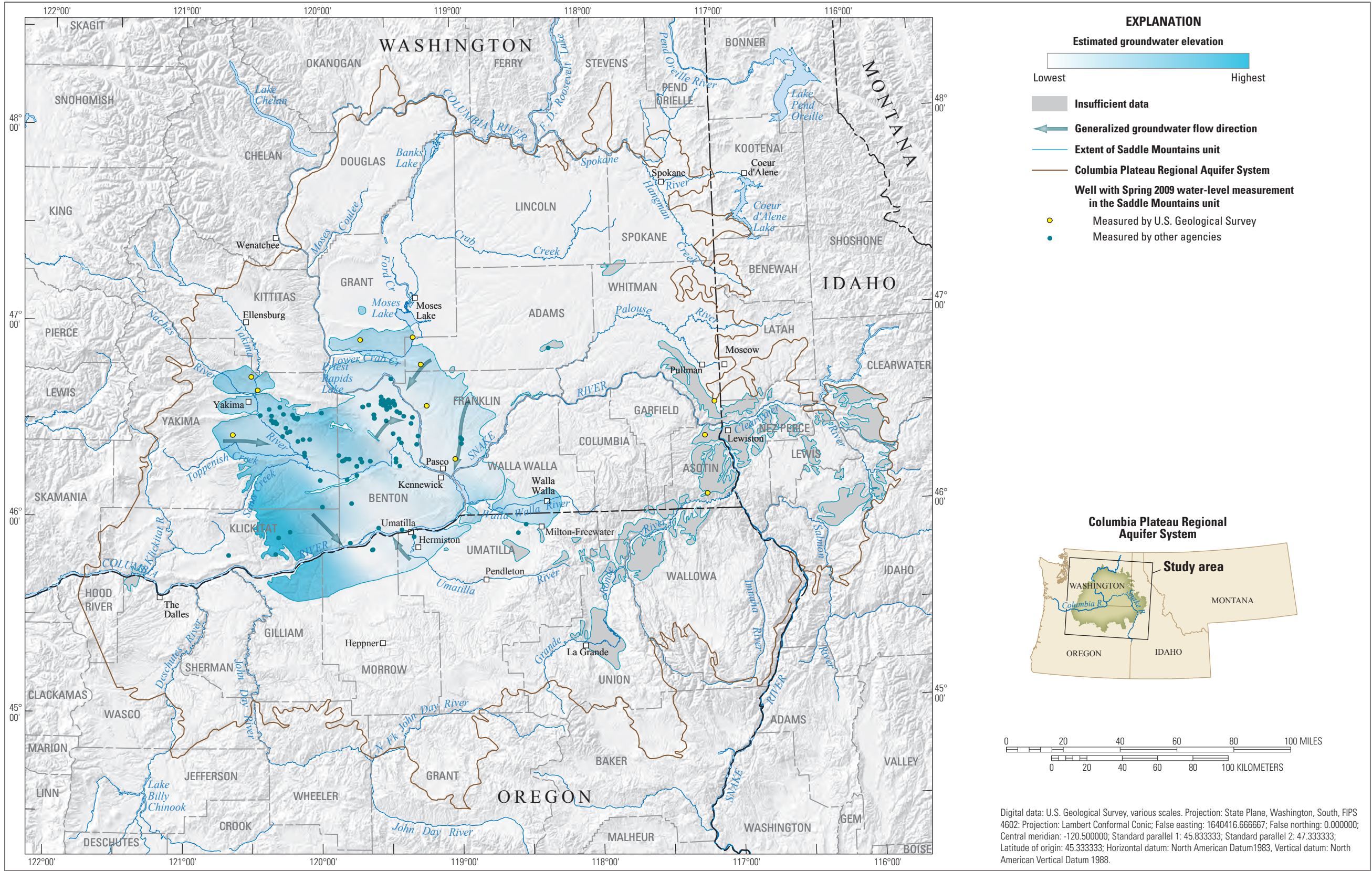
Locations of Wells and Estimated Groundwater Levels for the Saddle Mountains Unit, Columbia Plateau Regional Aquifer System, Washington, Oregon, and Idaho, Spring 2009
