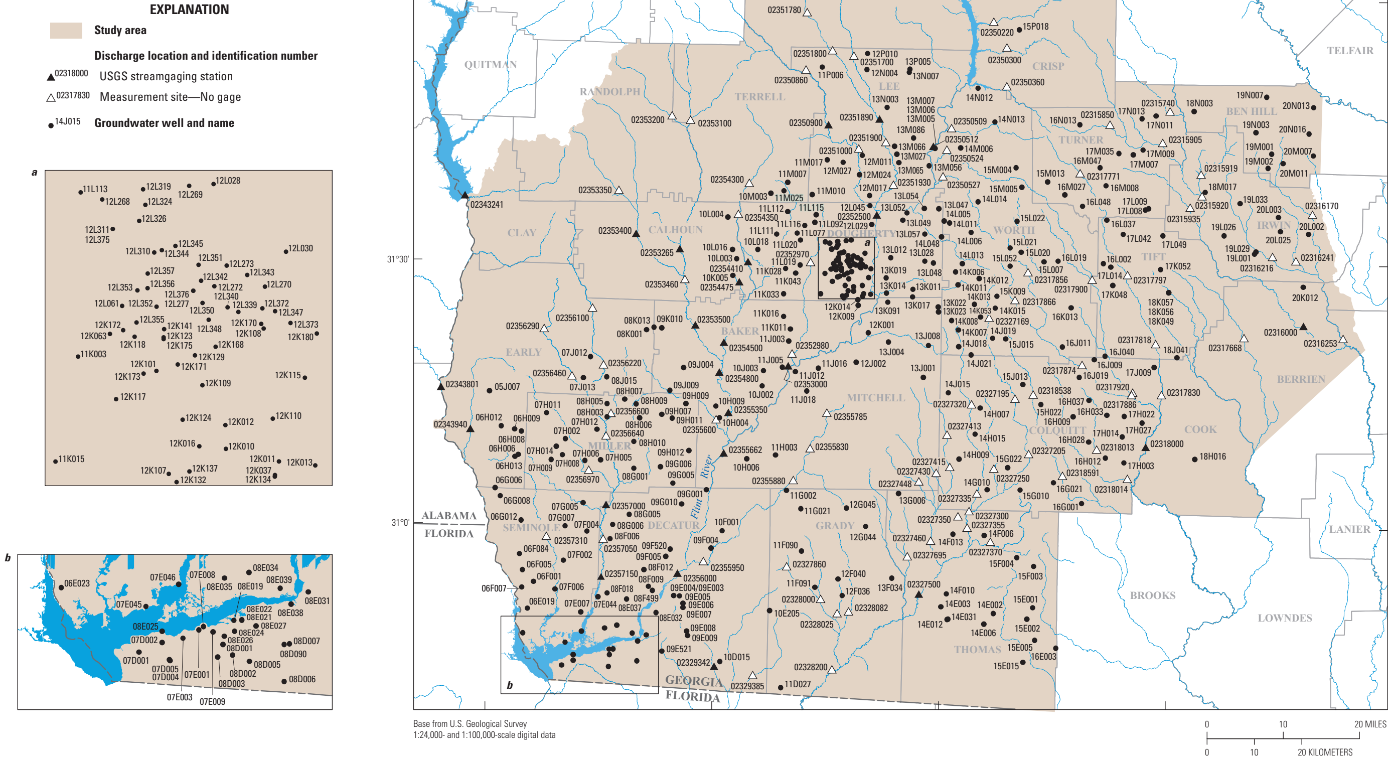
Figure A-1. Location of all measurements sites used to create a potentiometric surface of the Upper Floridan aquifer in south-central and southwestern Georgia during November 2008.
