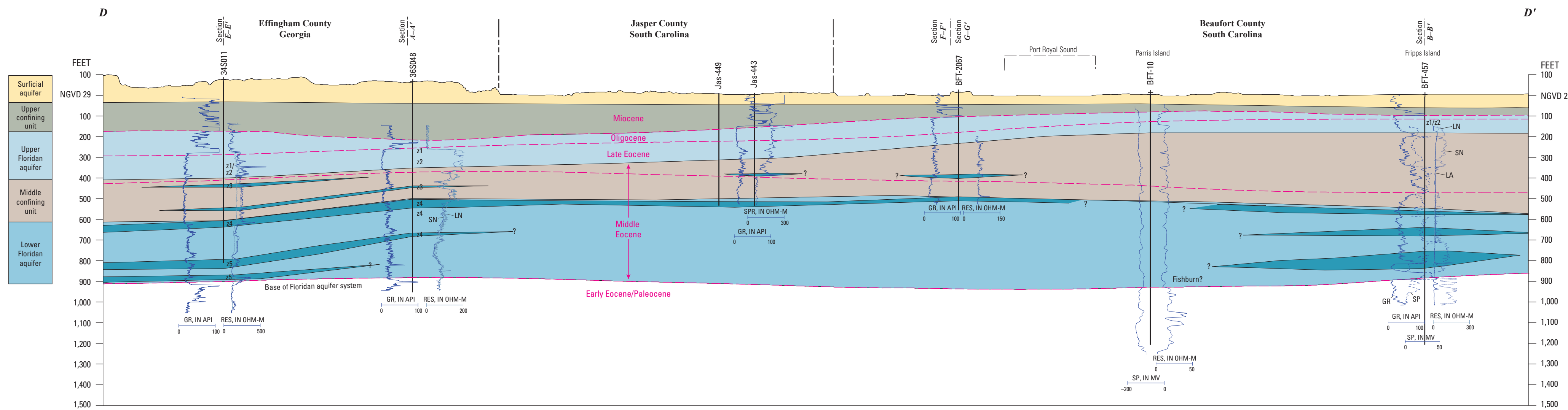
Geohydrologic cross sections A-A' through D-D', northern coastal area of Georgia and parts of South Carolina
