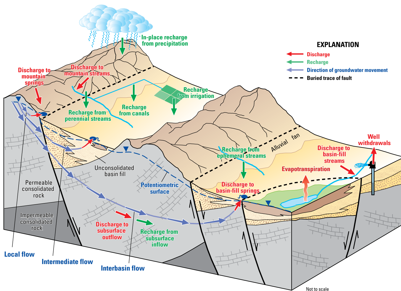
Figure C-1. Schematic diagram showing conceptualized groundwater flow in the Great Basin carbonate and alluvial aquifer system study area.
