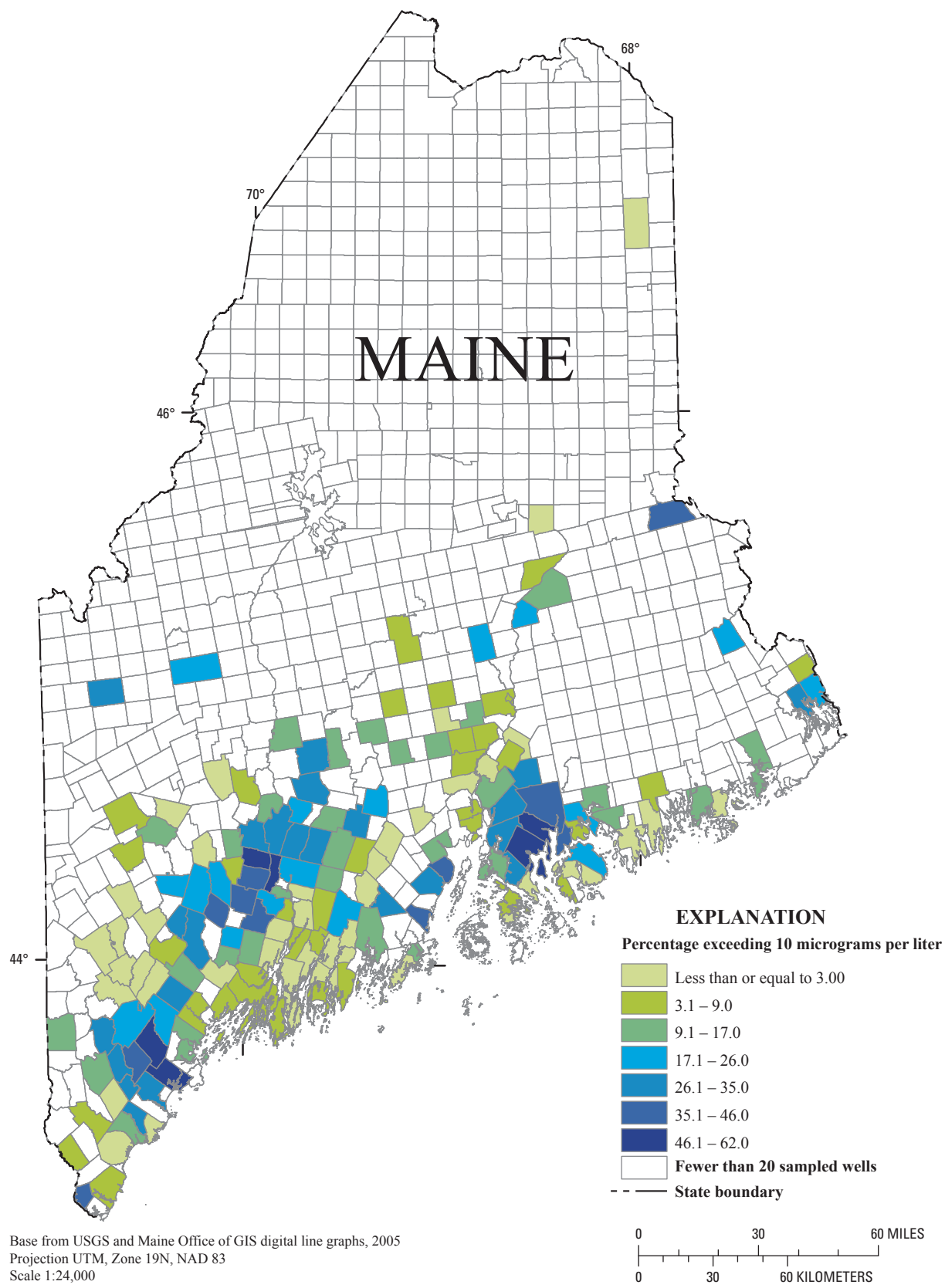
Figure B. Percentage of wells in each town with arsenic concentrations greater than 10 micrograms per liter in Maine, 2005–09. Towns shown have 20 or more wells.
