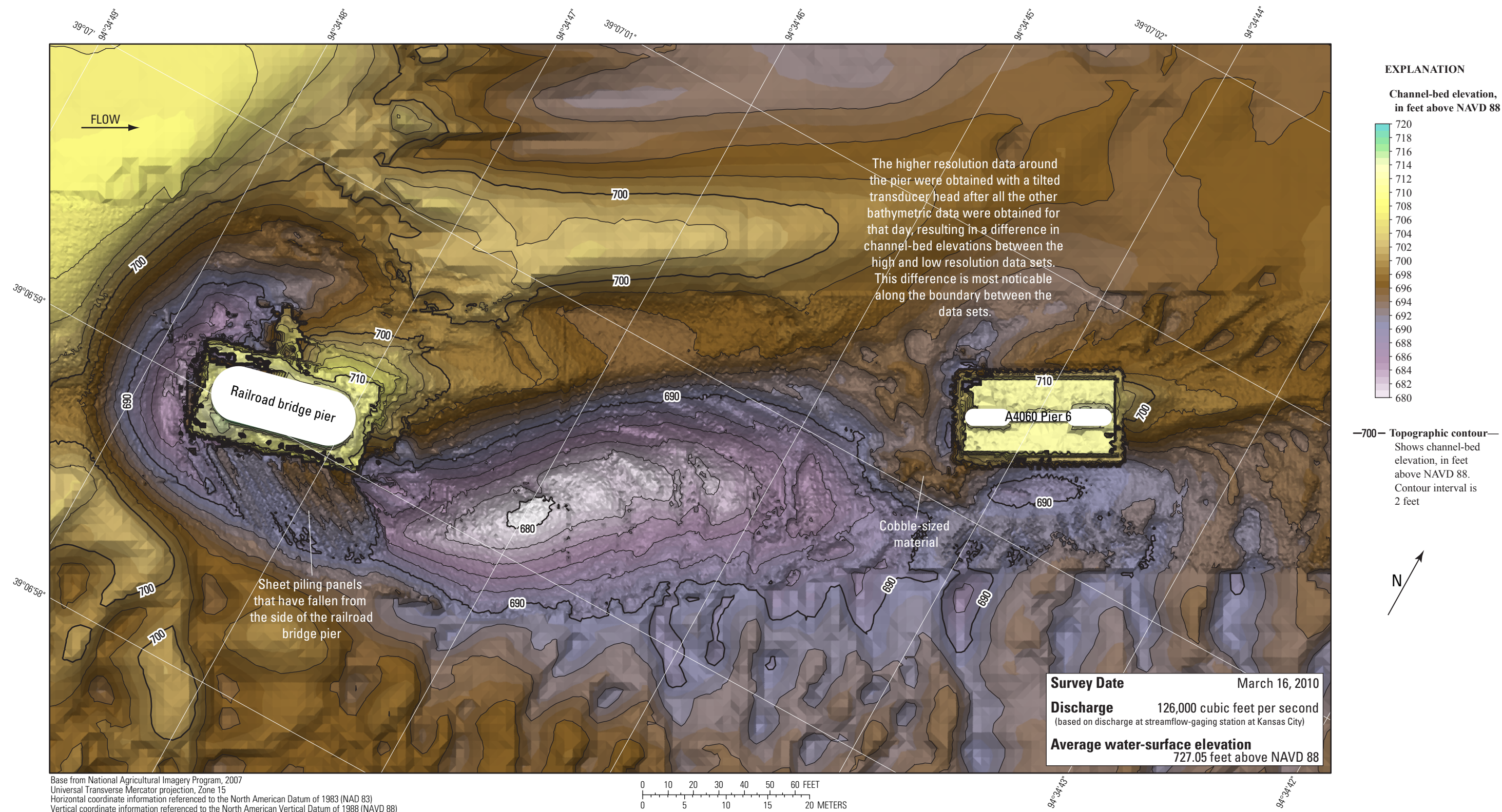
Figure 23. Bathymetric survey of the Missouri River channel in the vicinity of the right main channel pier of structure A4060 on State Highway 9 in Kansas City, Missouri.
