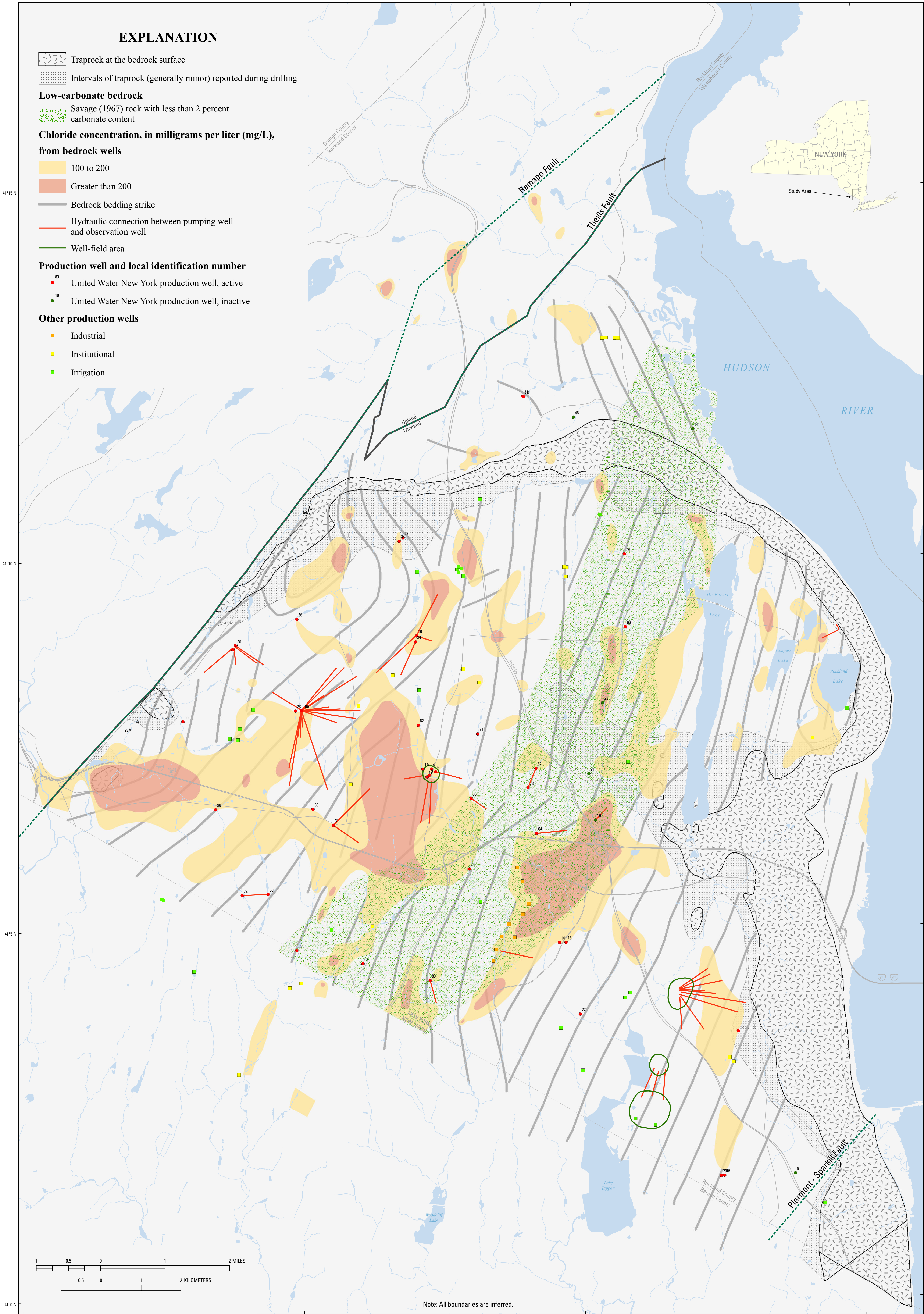
Figure 16B. Interpreted zonation of strike and dip in Newark basin bedrock with hydrogeologic data used in support of interpretation, Rockland County, New York
