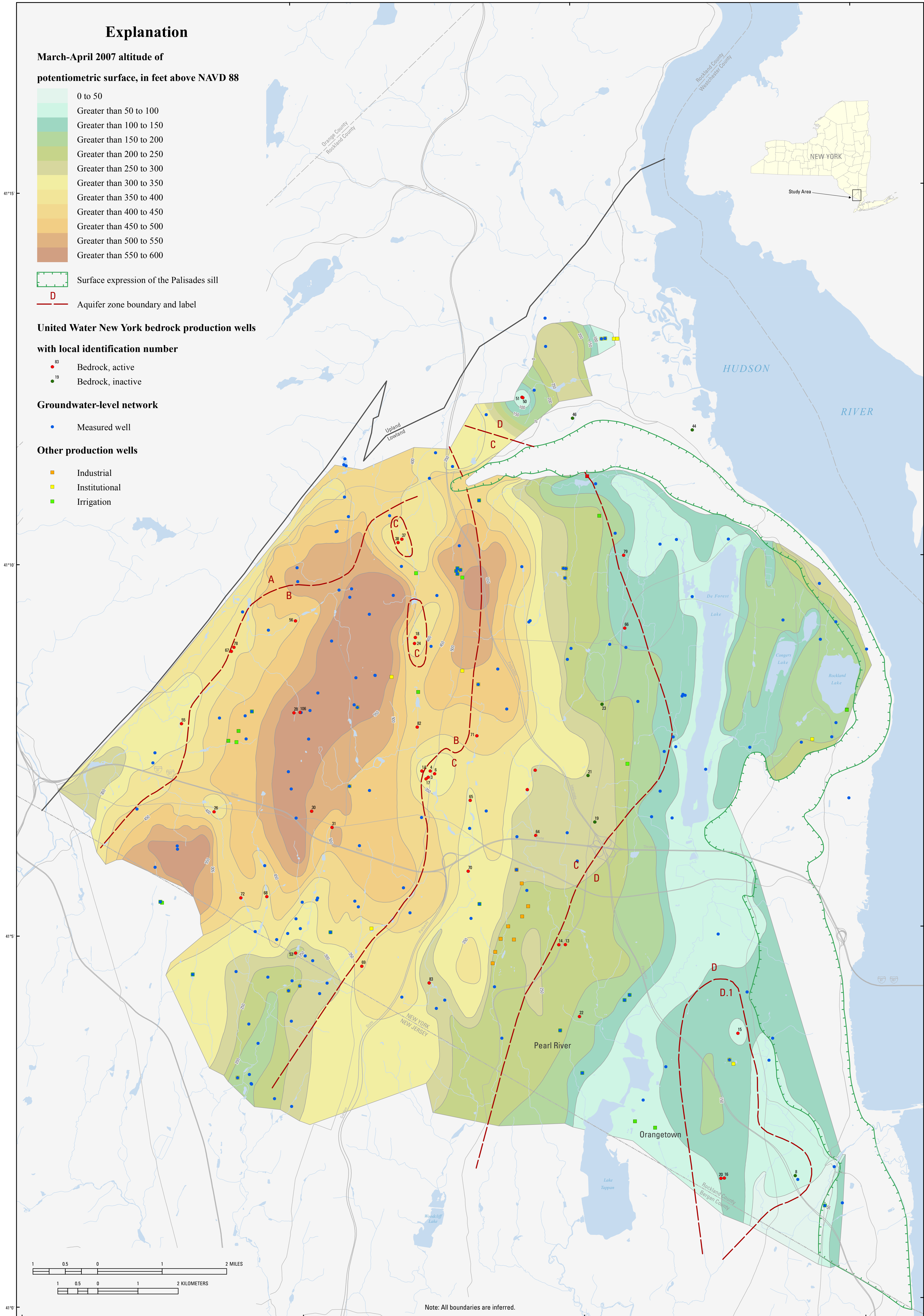
Figure 30. Spring 2007 potentiometric-surface map with points of groundwater withdrawal, Newark basin aquifer, Rockland County, New York
