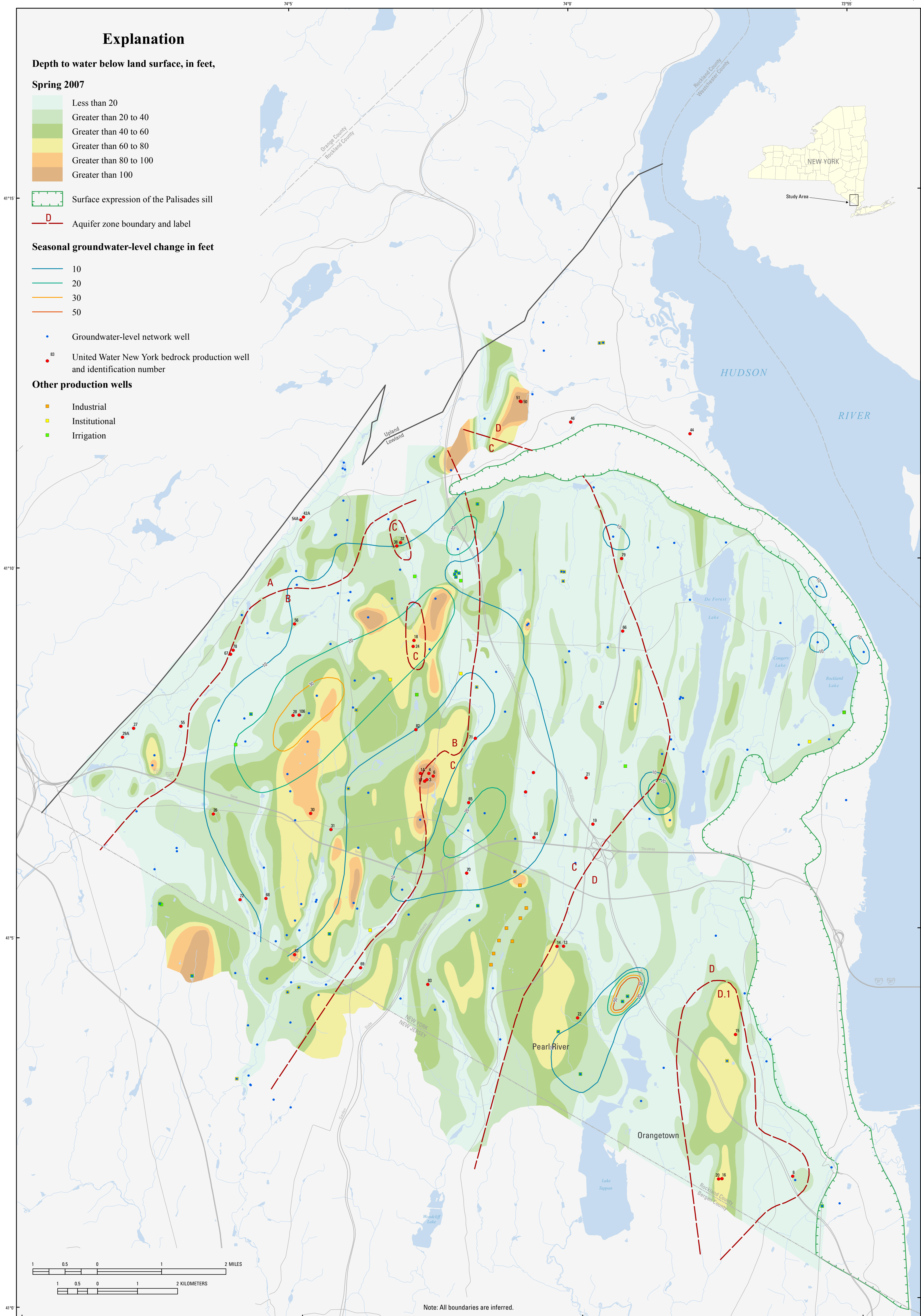
Figure 31. Seasonal groundwater-level change (Spring 2007 to Summer 2005), Newark basin aquifer, Rockland County, New York
