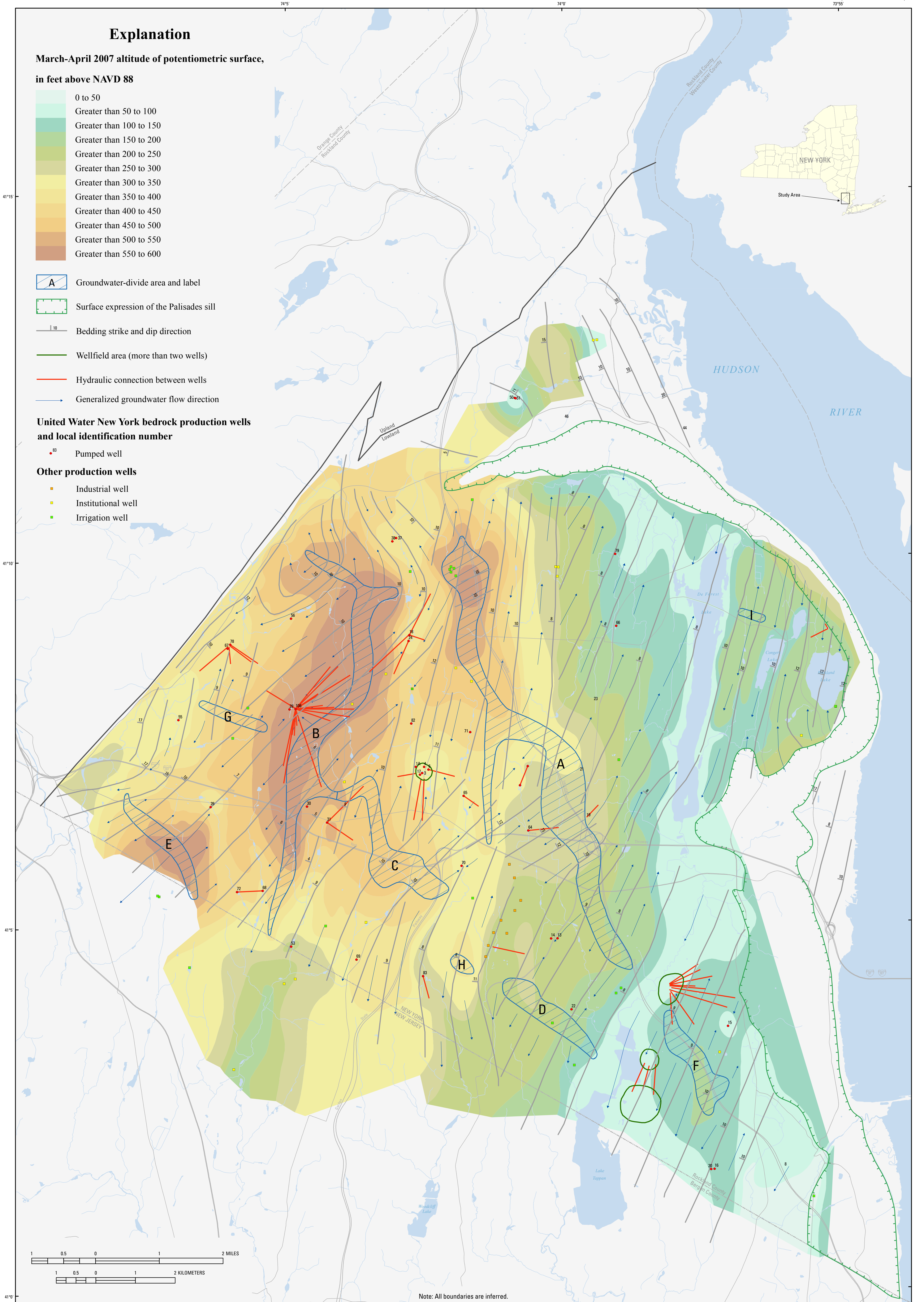
Figure 32. Newark basin aquifer groundwater-flow-system map, Spring 2007, Rockland County, New York
