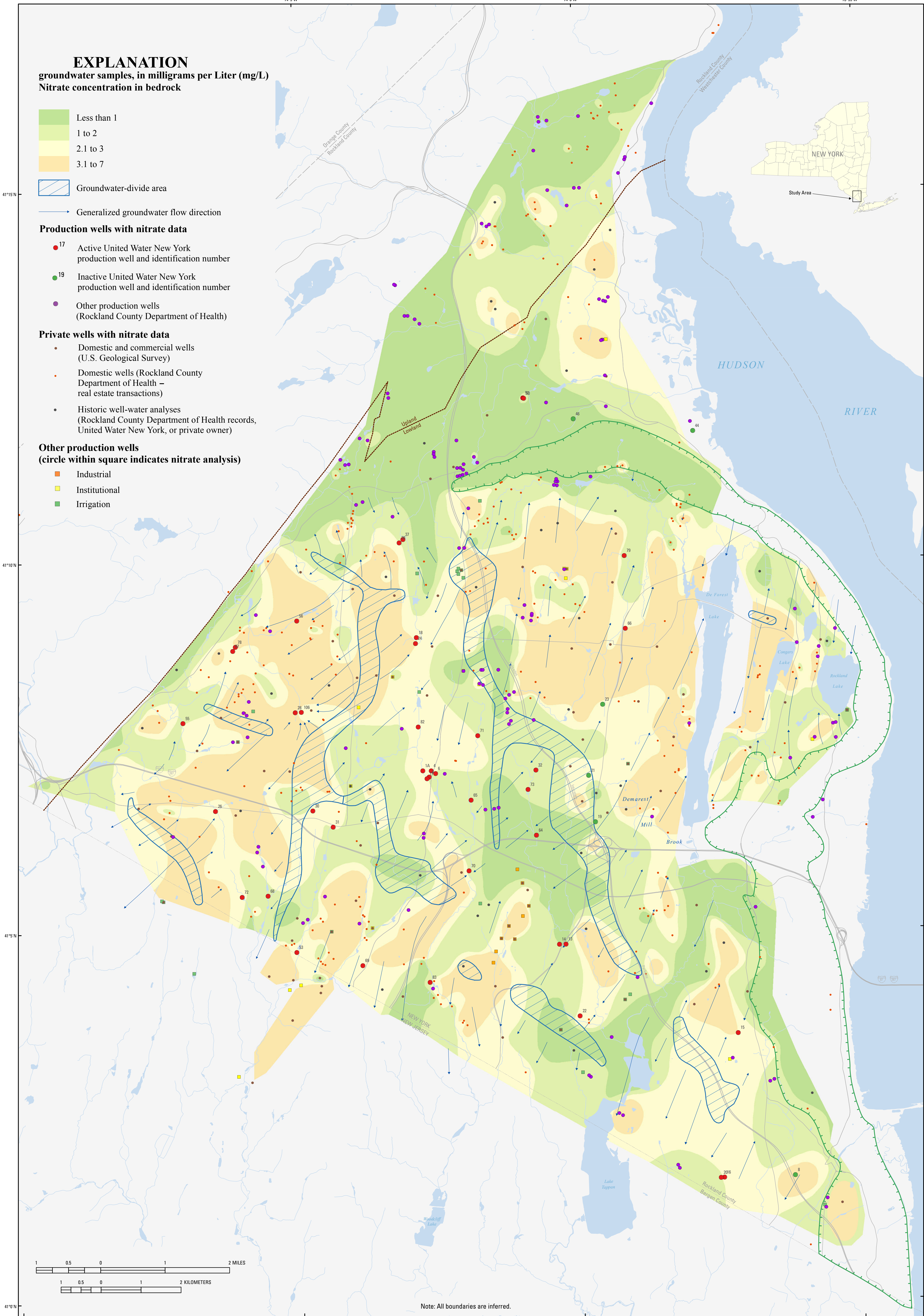
Figure 38. Distribution of nitrate in groundwater within the Newark basin aquifer and surrounding areas, Rockland County, New York
