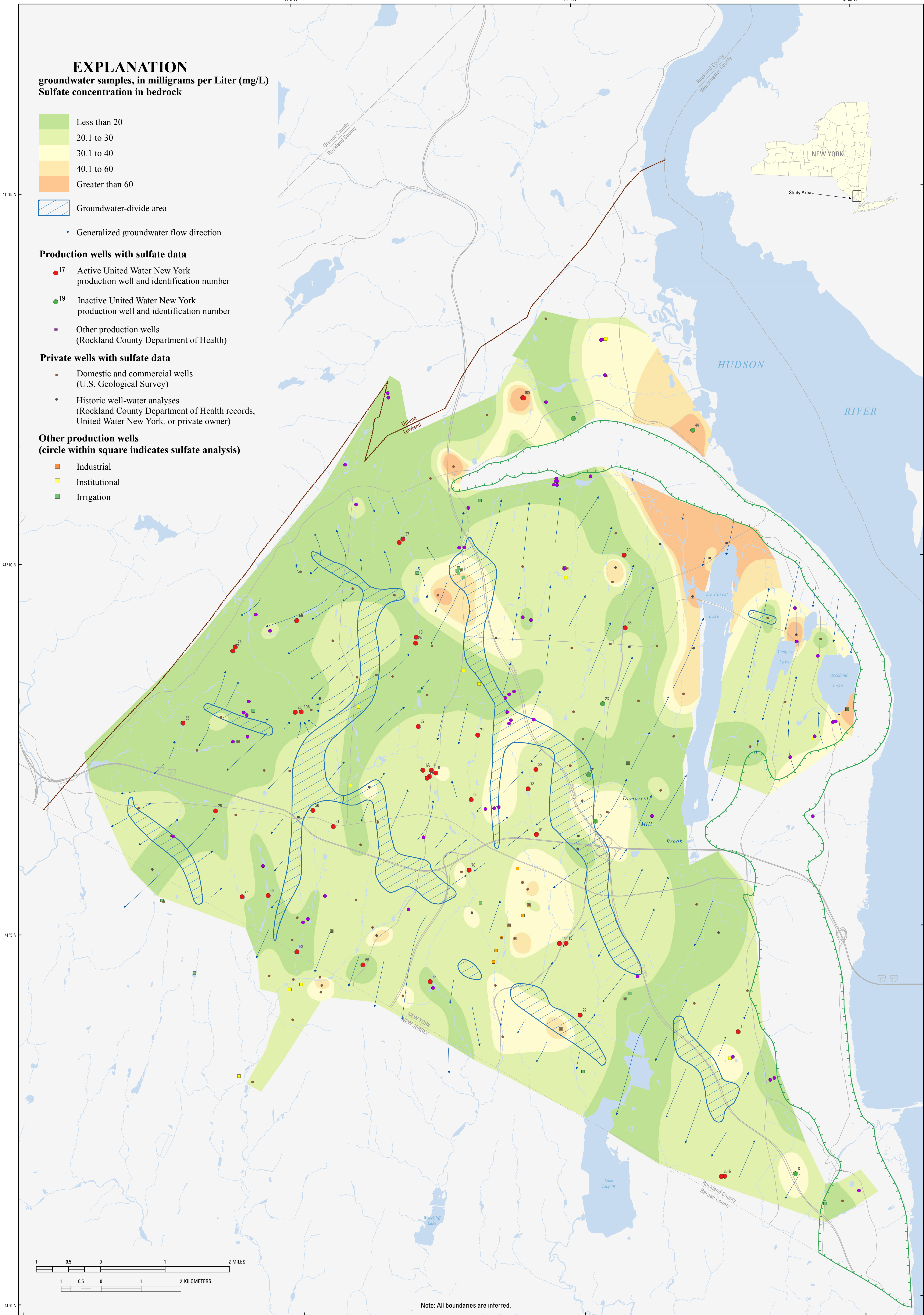
Figure 40. Distribution of sulfate in groundwater within the Newark basin aquifer and surrounding areas, Rockland County, New York
