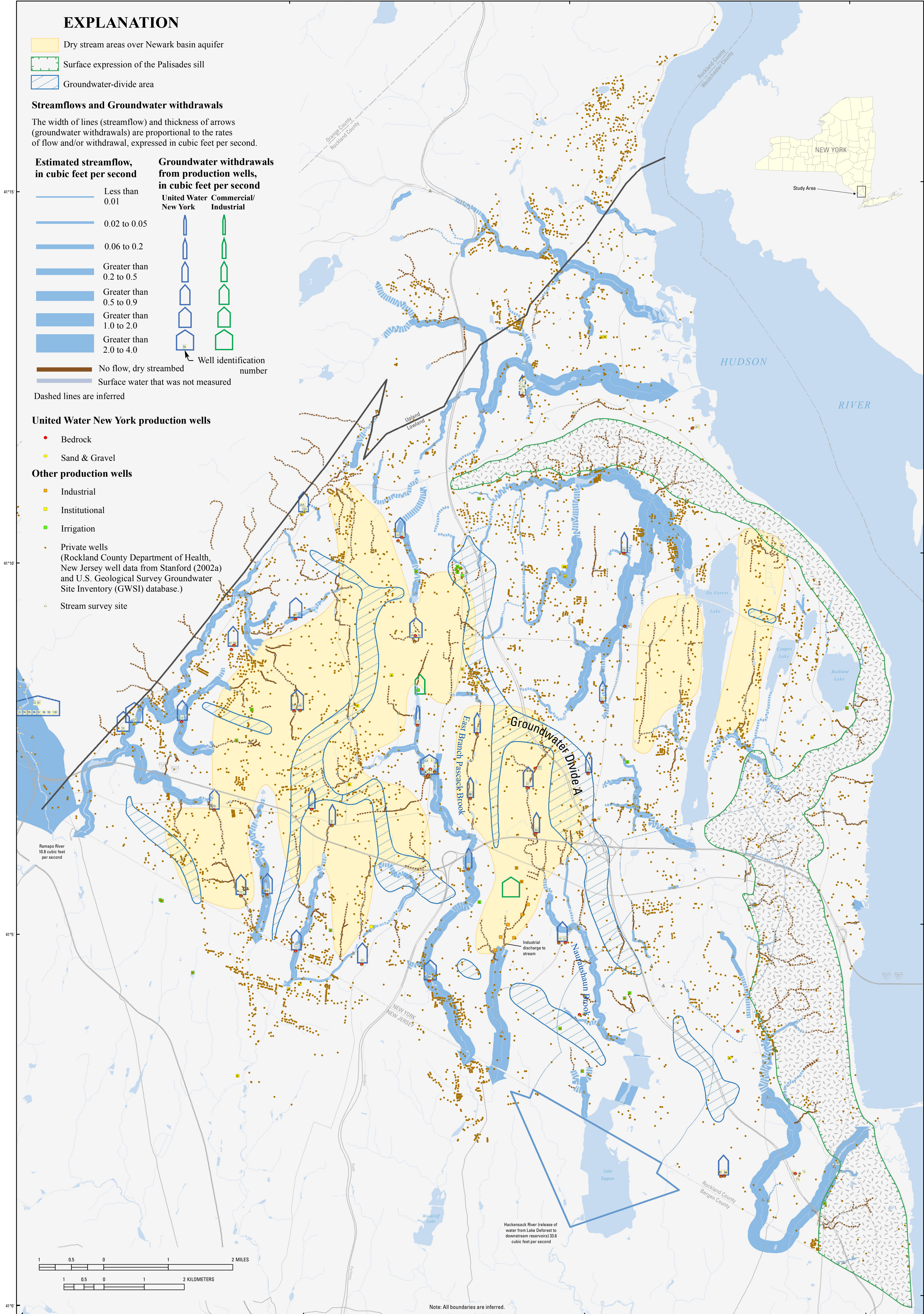
Figure 46. Estimated flow of streams on or adjacent to the Newark basin aquifer and pumping rates from production wells, September-October 2005, Rockland County, New York.
