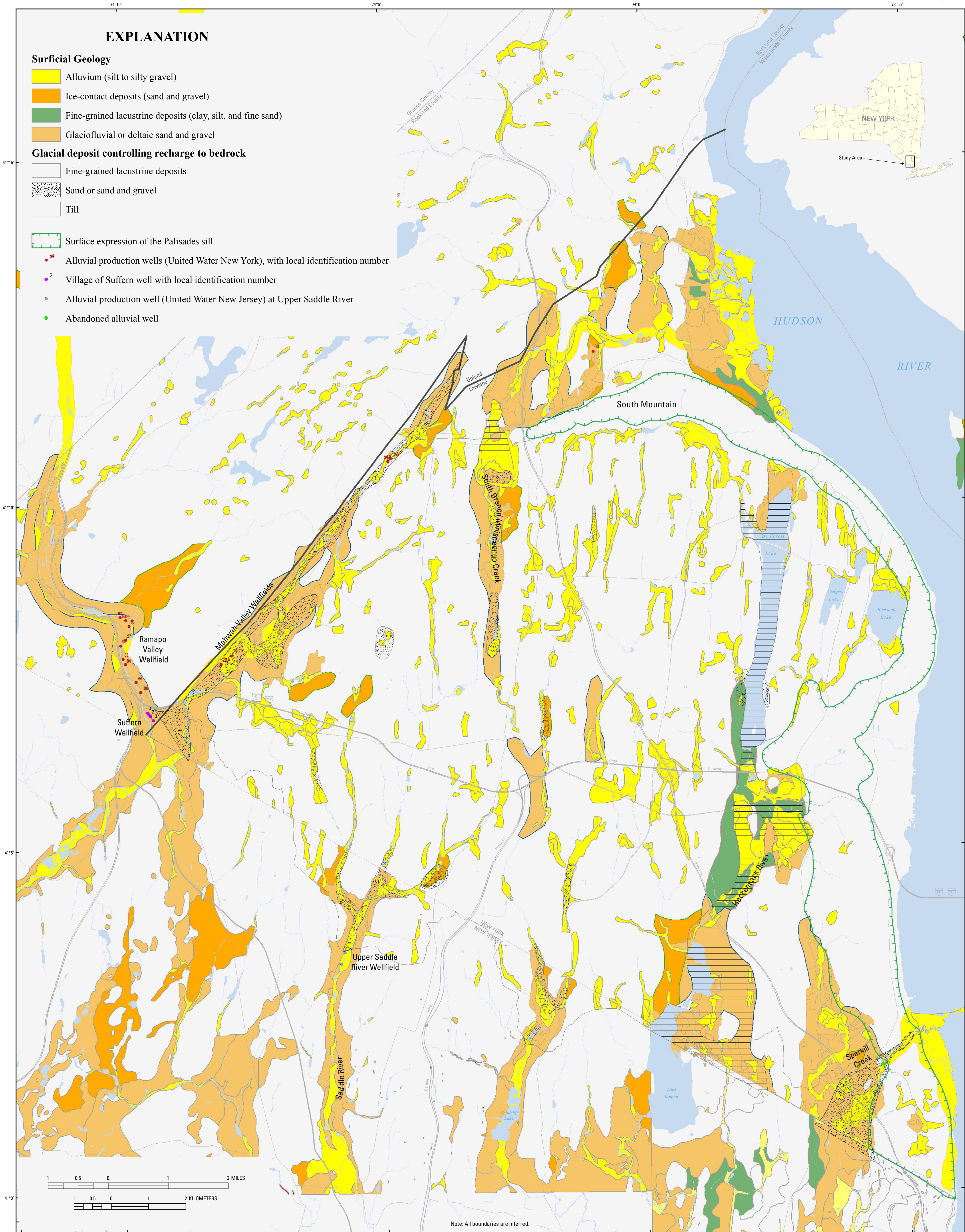
Figure 7A. Distribution of unconsolidated glacial and alluvial deposits in Rockland County, New York and the surrounding areas
