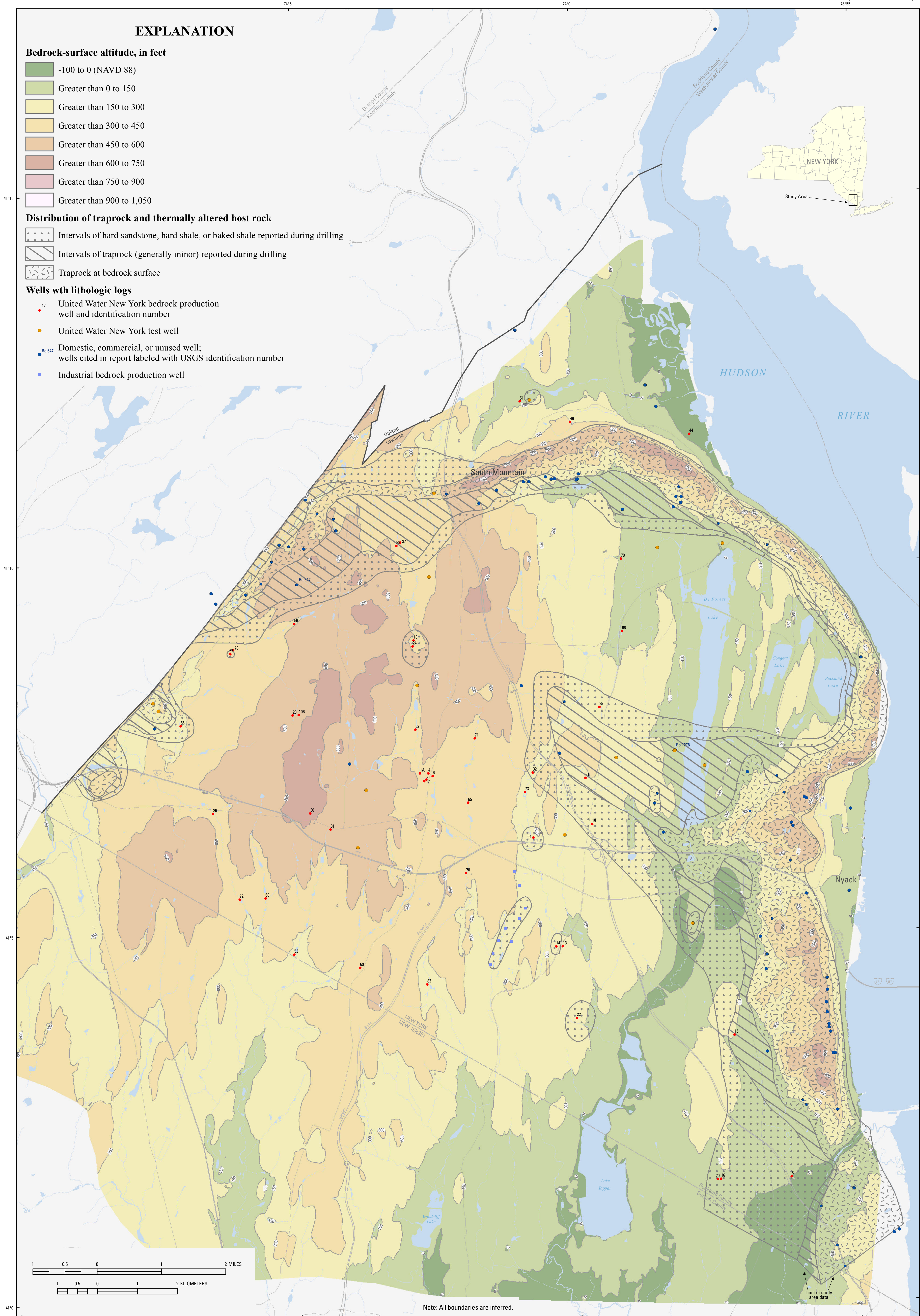
Figure 9. Distribution of (1) traprock and thermally altered host rock and (2) bedrock-surface altitude within the Newark basin, Rockland County, New York
