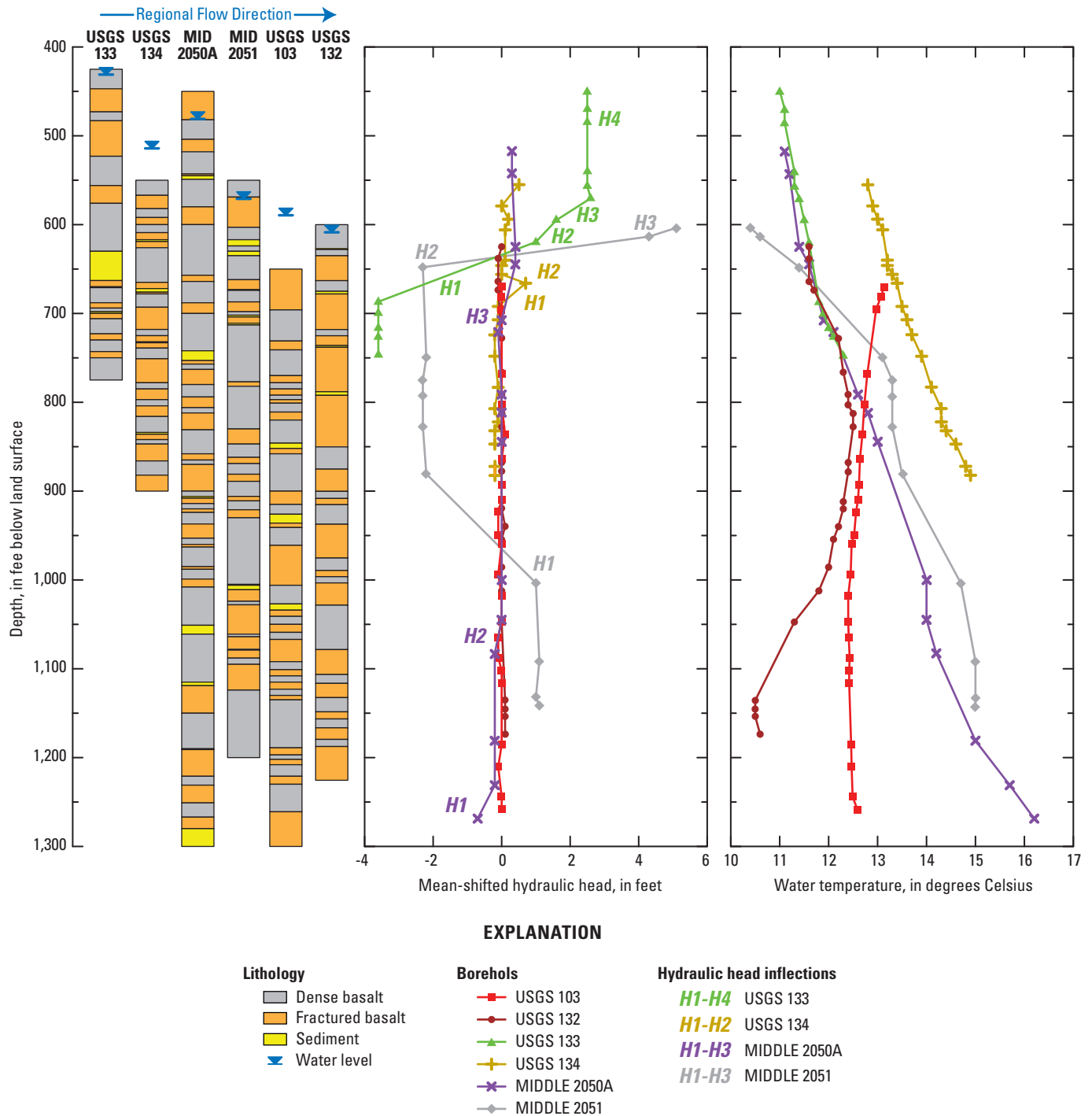
Figure 18. Comparison among borehole lithology logs and mean-shifted hydraulic head and water temperature profiles for boreholes USGS 103, USGS 132, USGS 133, USGS 134, MIDDLE 2050A, and MIDDLE 2051, Idaho National Laboratory, Idaho, June 2008.
