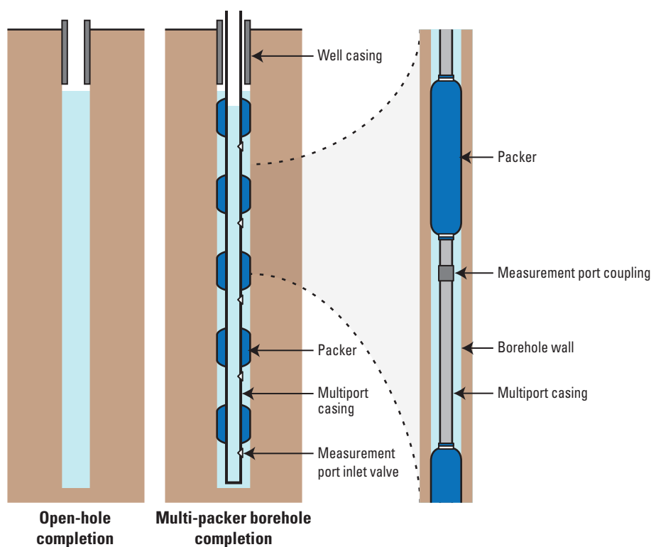
Figure 2. Open-hole and multi-packer borehole completions, eastern Snake River Plain aquifer, Idaho National Laboratory, Idaho, 2007–08.
