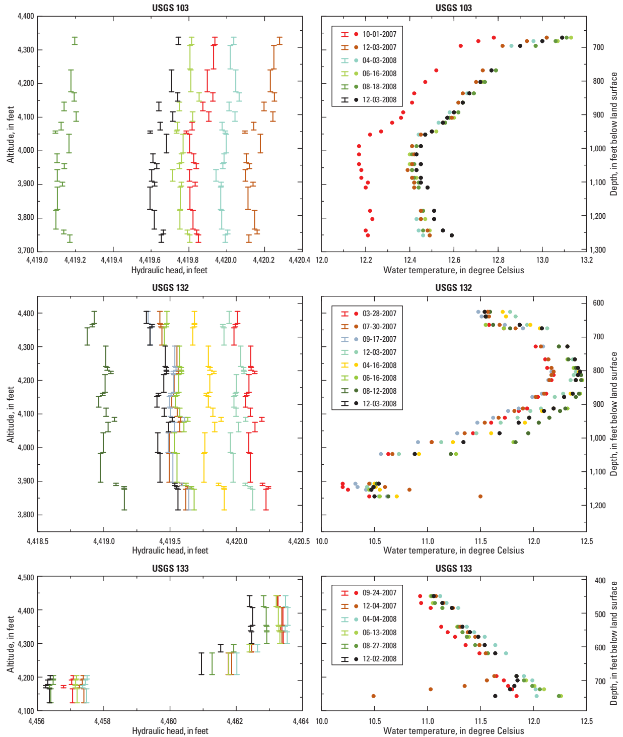
Figure 11. Vertical hydraulic head and water temperature profiles at boreholes USGS 103, USGS 132, USGS 133, USGS 134, MIDDLE 2050A, and MIDDLE 2051, Idaho National Laboratory, Idaho. Profiles are based on quarterly measurements made during 2007 and 2008.
