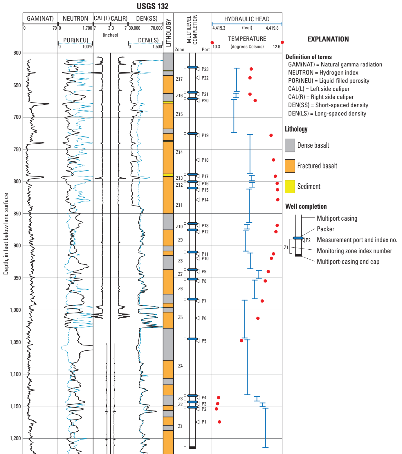
Figure 13. Geophysical traces of natural gamma, neutron, caliper, and gamma-gamma dual density; lithology log; multilevel completion; and hydraulic head and water temperature profiles for borehole USGS 132, Idaho National Laboratory, Idaho, June 2008.
