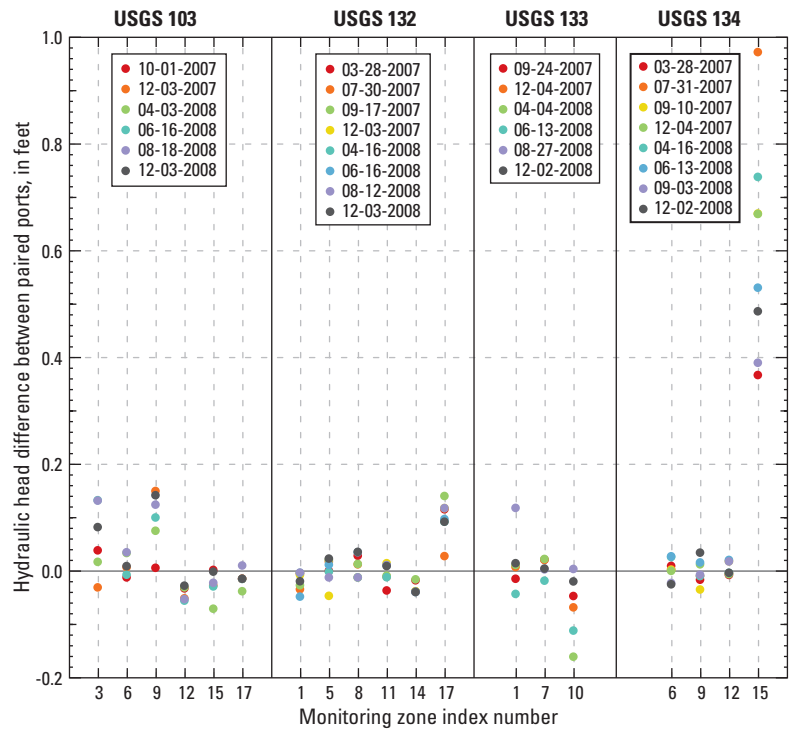
Figure 10. Hydraulic head differences between paired-ports, measurement ports in the same monitoring zone, in boreholes USGS 103, USGS 132, USGS 133, and USGS 134, Idaho National Laboratory, Idaho, 2007–08.
