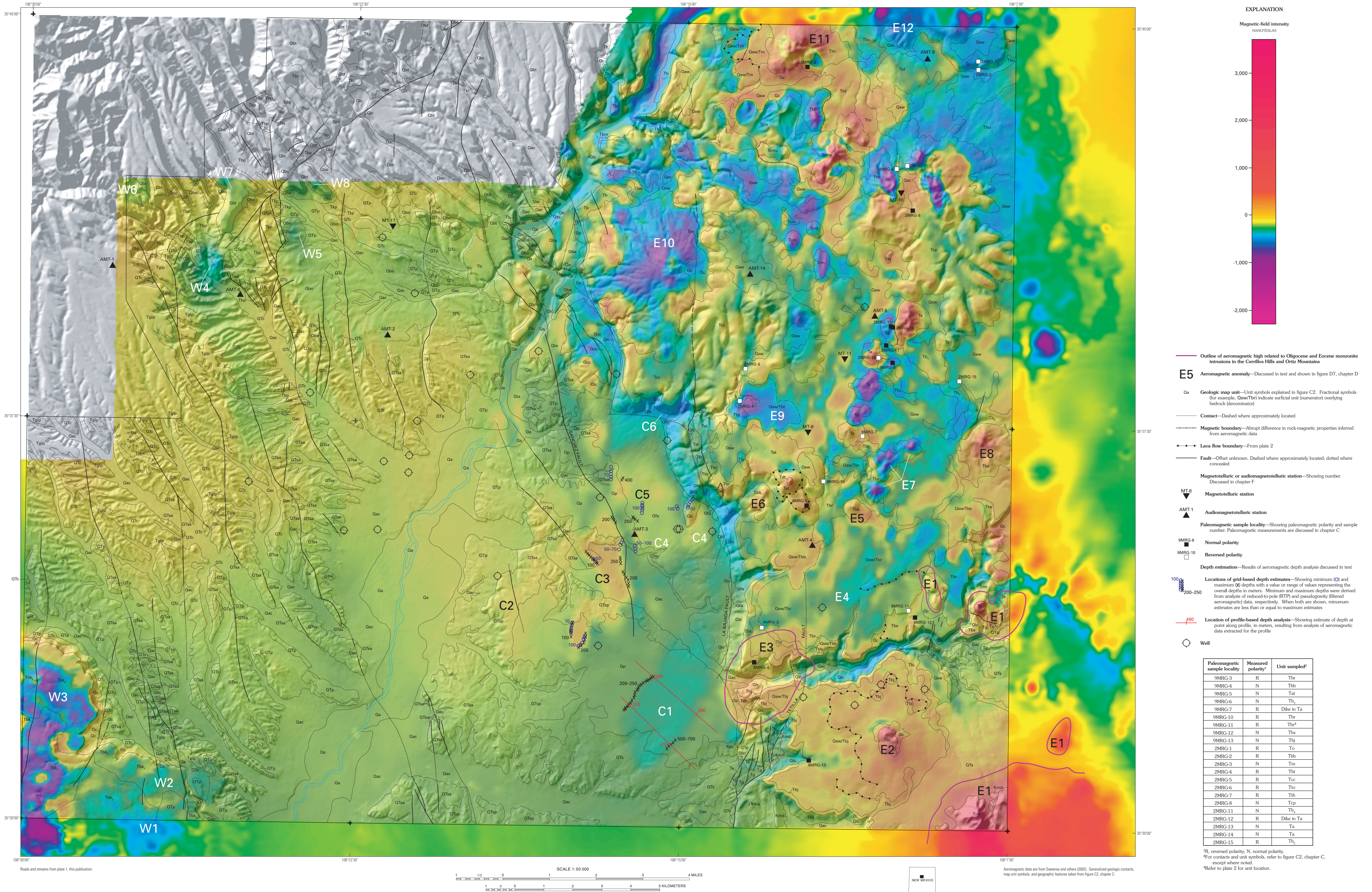
MAP SHOWING REDUCED-TO-POLE AEROMAGNETIC DATA, GEOLOGY, AND TOPOGRAPHY FOR THE COCHITI PUEBLO AREA, NEW MEXICO
