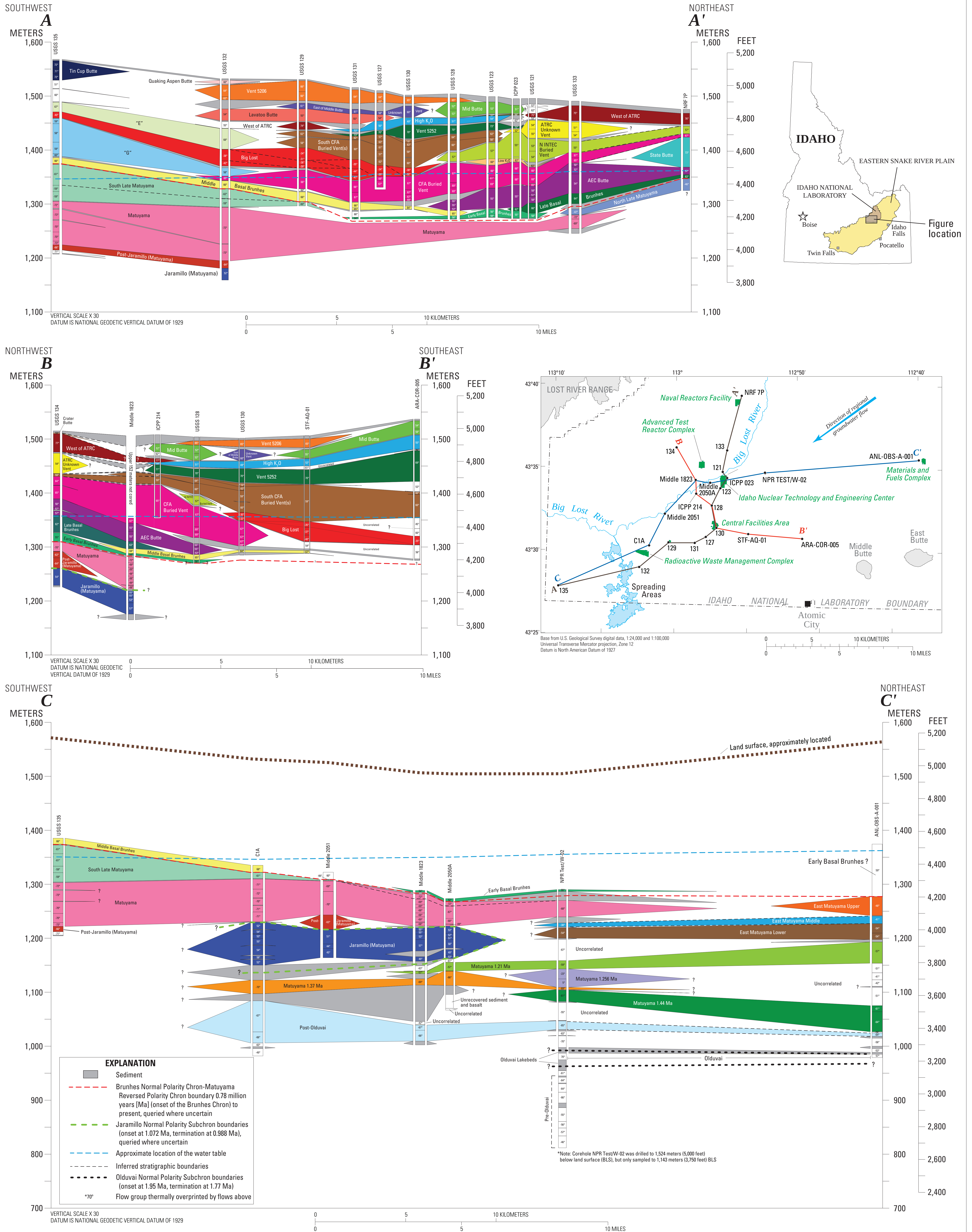
Map and Cross-sections of Subsurface Stratigraphy Interpreted from Paleomagnetic Inclination Data from Coreholes in the Southern Part of the Idaho National Laboratory, Idaho
