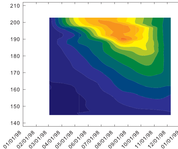
TIME-DEPTH DISTRIBUTION OF TEMPERATURE NEAR BULL SHOALS LAKE DAM.
