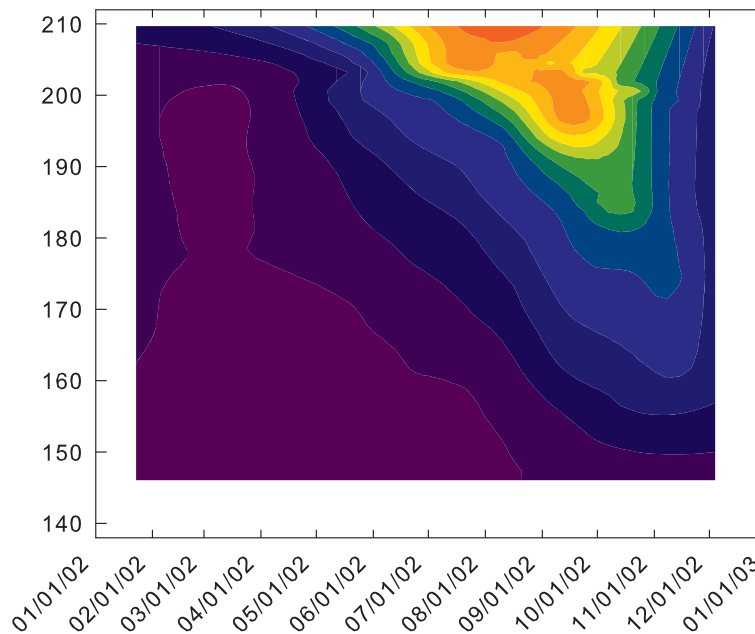
TIME-DEPTH DISTRIBUTION OF TEMPERATURE NEAR BULL SHOALS LAKE DAM.
