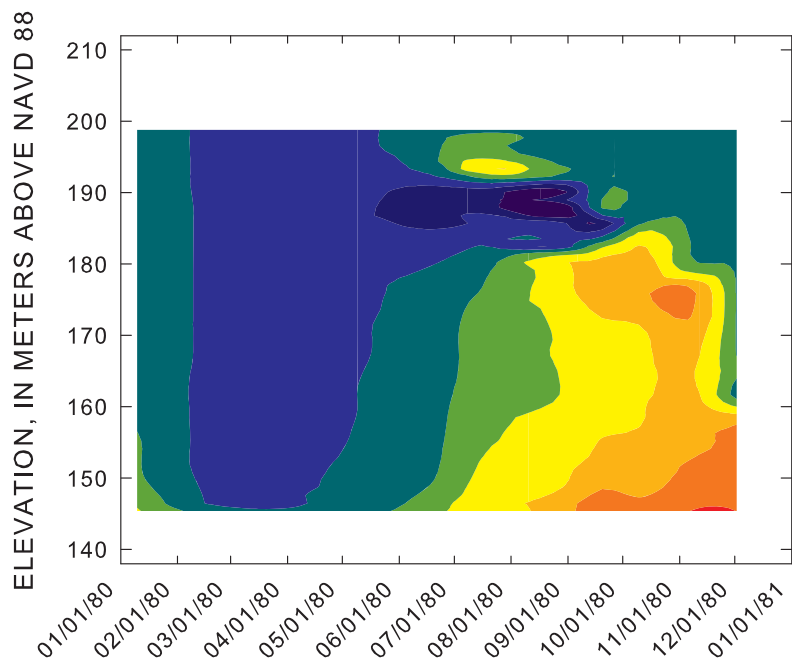
TIME-DEPTH DISTRIBUTION OF DISSOLVED OXYGEN NEAR BULL SHOALS LAKE DAM.
