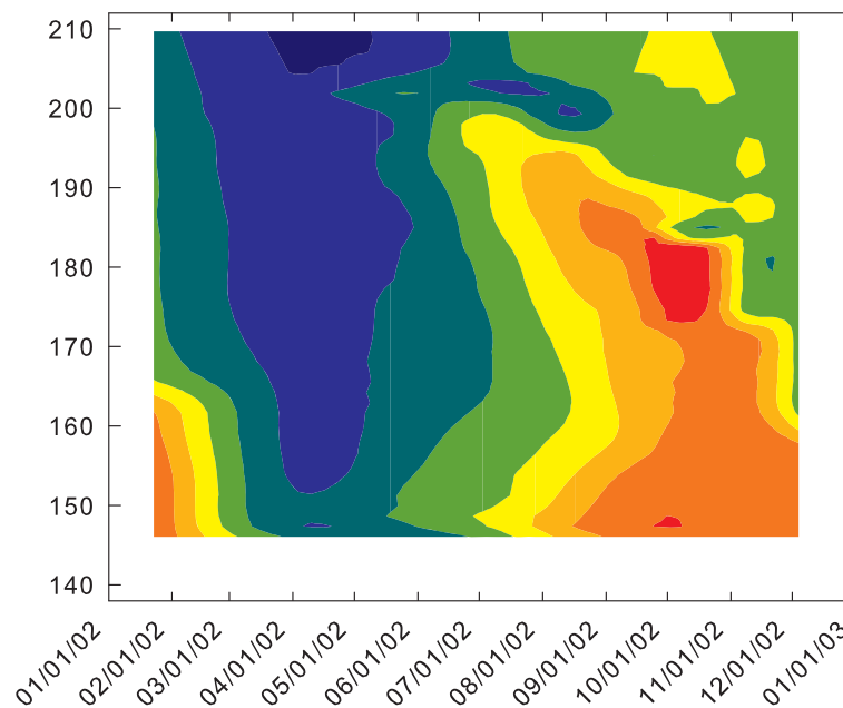
TIME-DEPTH DISTRIBUTION OF DISSOLVED OXYGEN NEAR BULL SHOALS LAKE DAM.
