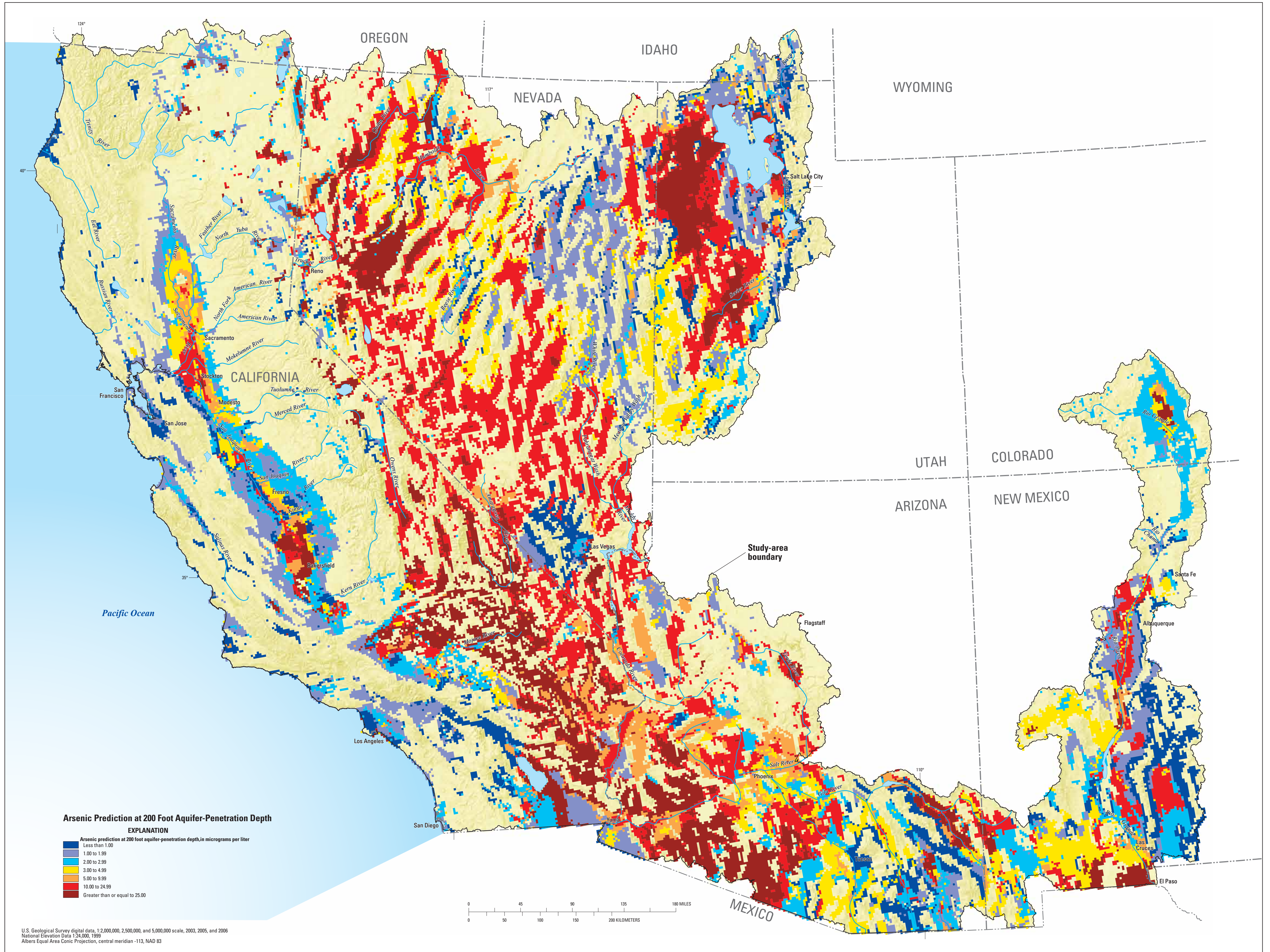
Appendix 9. Observed and predicted arsenic concentrations in basin-fill aquifers of the Southwest Principal Aquifers study area
