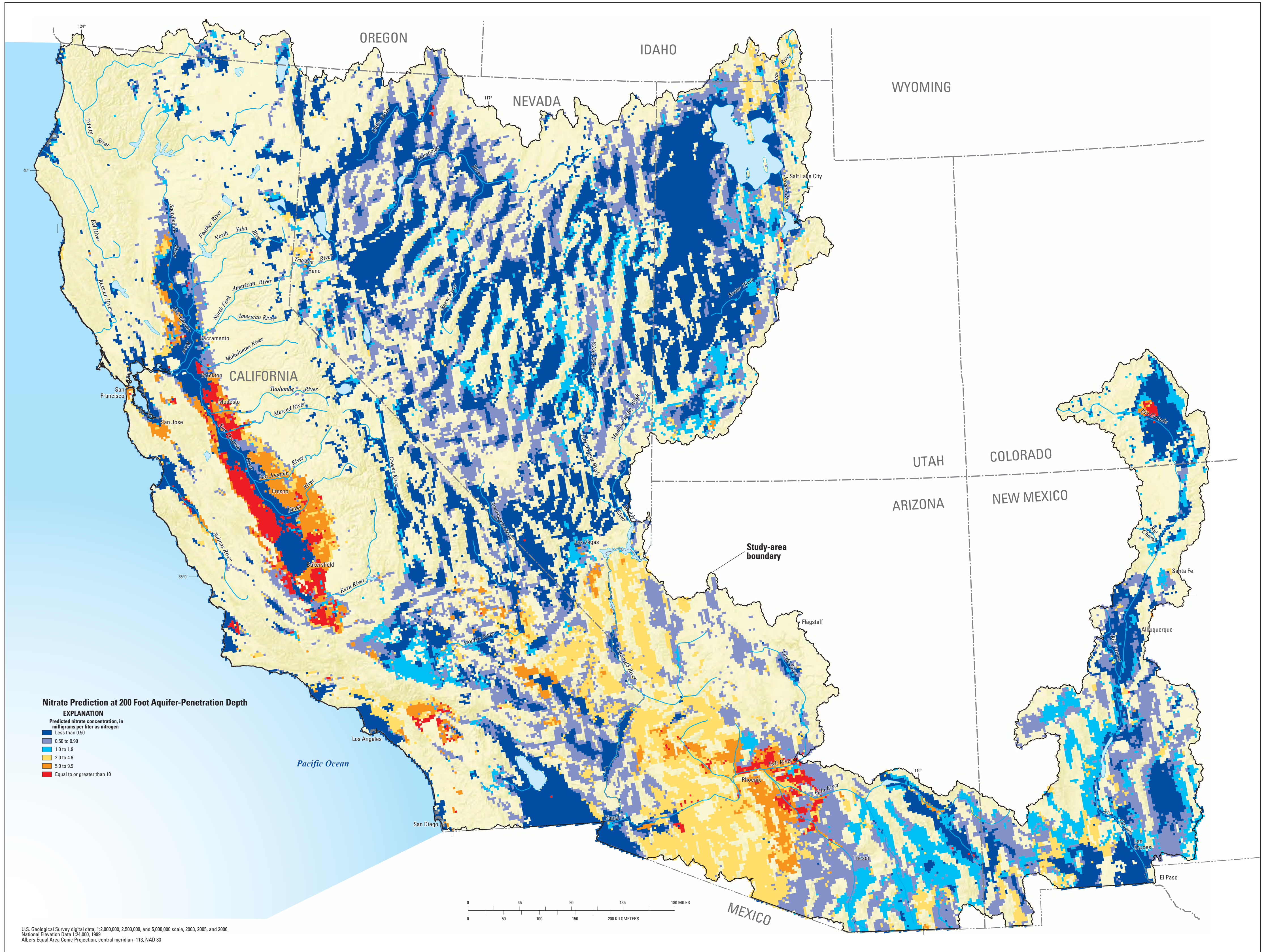
Appendix 8. Observed and predicted nitrate concentrations in basin-fill aquifers of the Southwest Principal Aquifers study area
