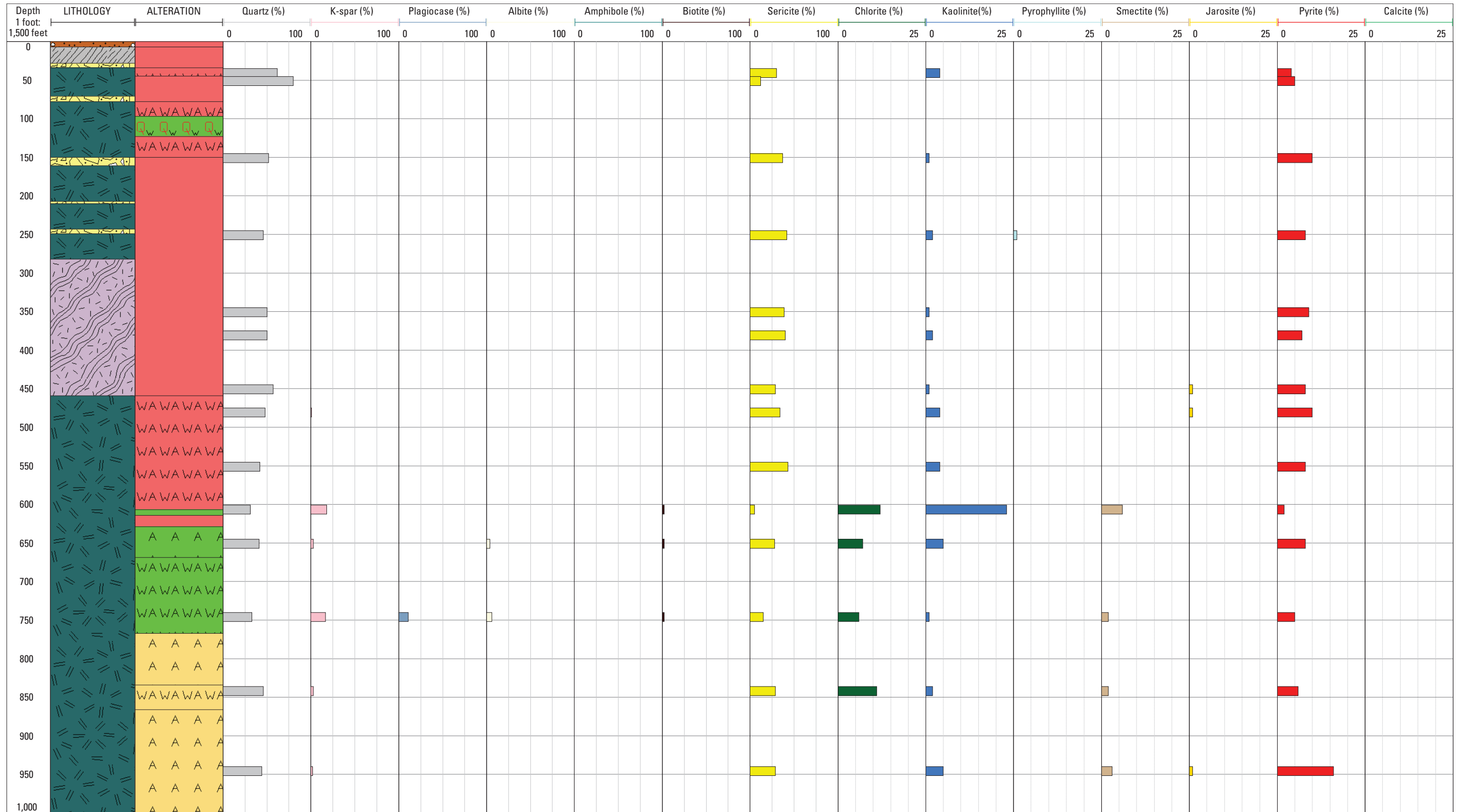
Figure 4. Core logs showing lithology, alteration assemblages, and quantitative mineralogy in drill holes A, WP1. B, WP2. C, WP3. D, WP4. E, HCBW1. F, HCBW3. See Appendix A for key to all lithology and alteration types.
