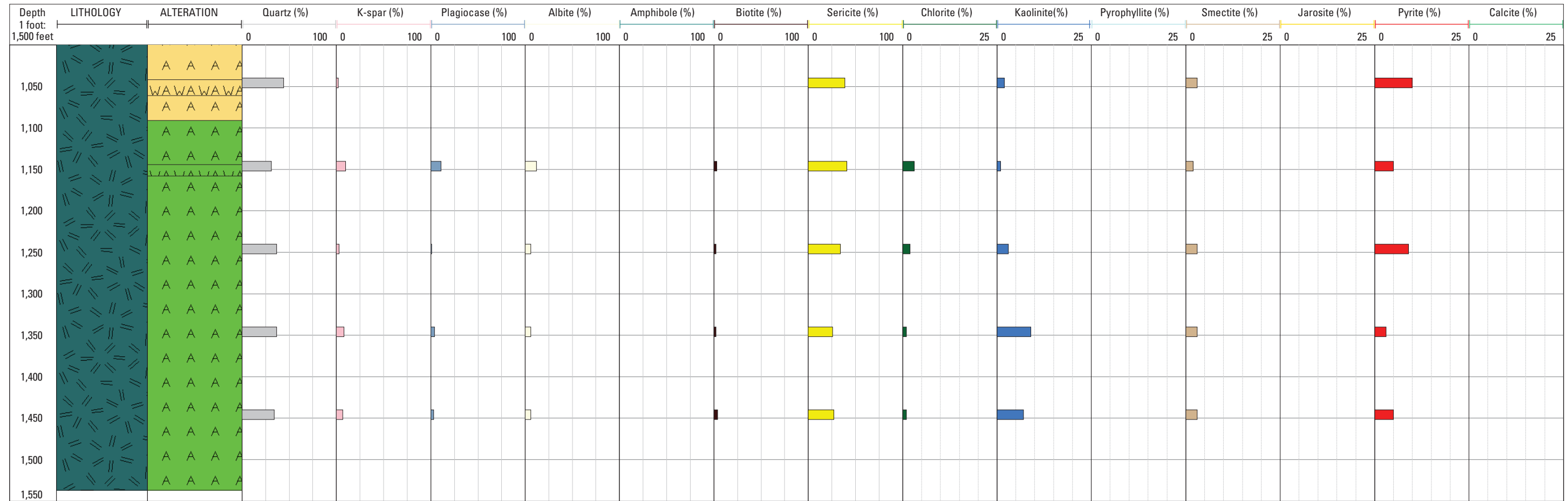
Figure 4. Core logs showing lithology, alteration assemblages, and quantitative mineralogy in drill holes A, WP1. B, WP2. C, WP3. D, WP4. E, HCBW1. F, HCBW3. See Appendix A for key to all lithology and alteration types.—Continued
