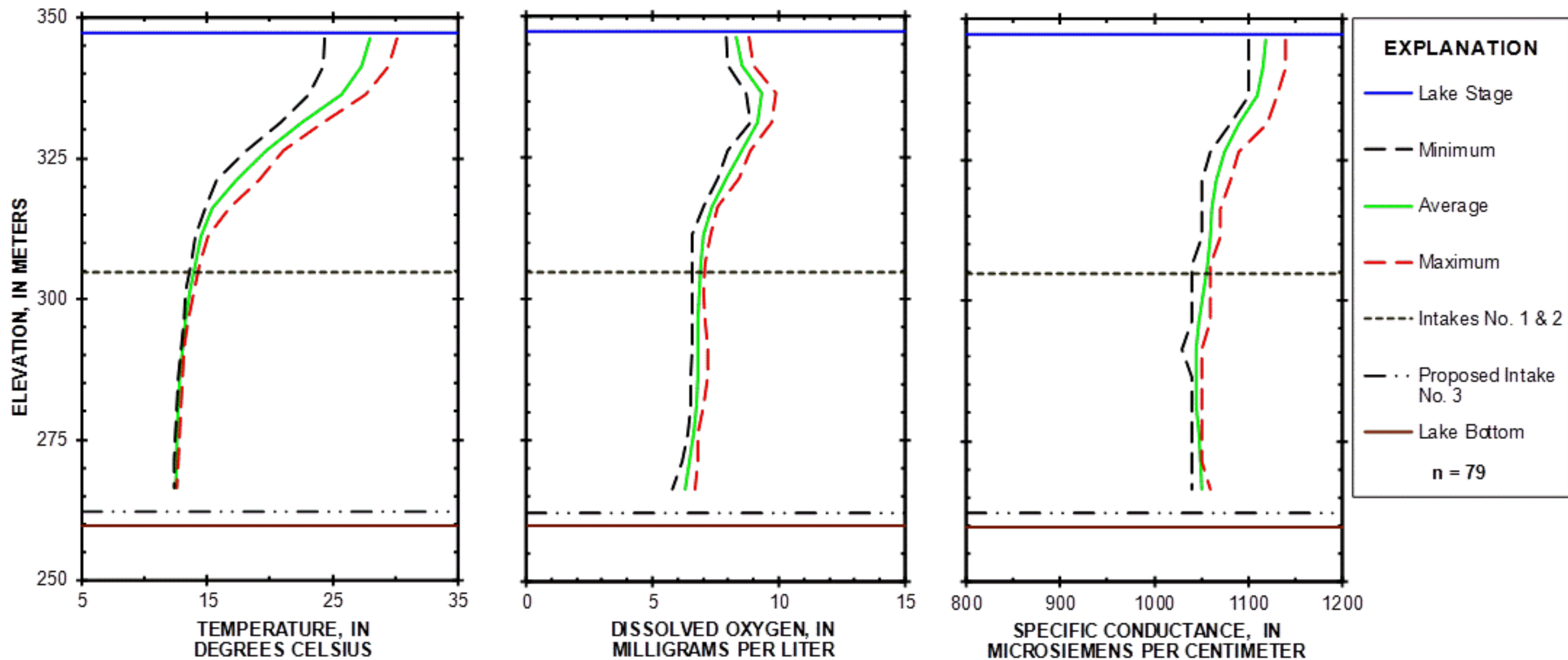
USGS Water-Quality Monitoring Station, Sentinel Island, Lake Mead: 07-01-05 through 07-31-05
