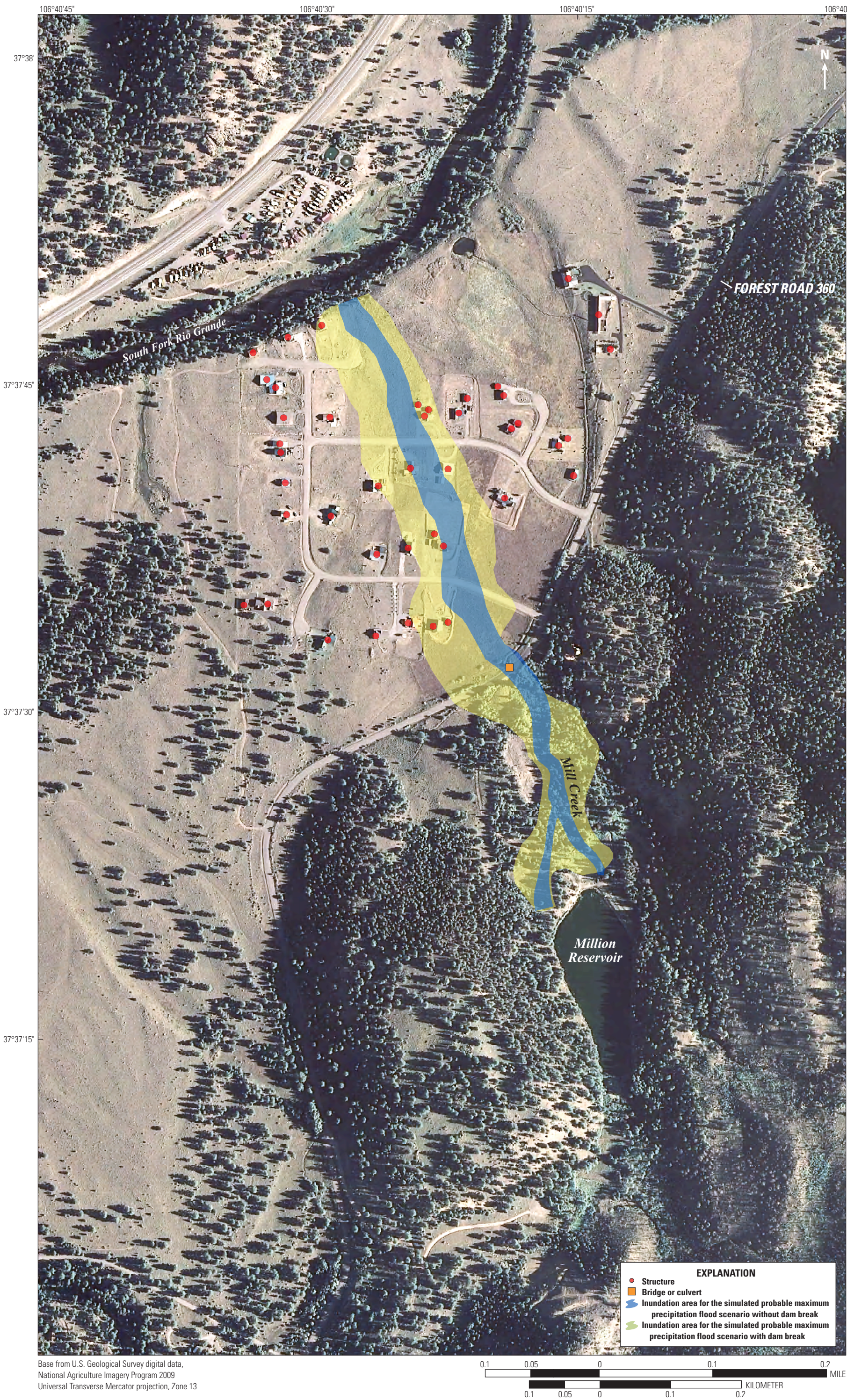
Figure 32. Flood inundation map for a simulated dam breach at Million Reservoir from a probable maximum precipitation, 24-hour inflow design flood.
