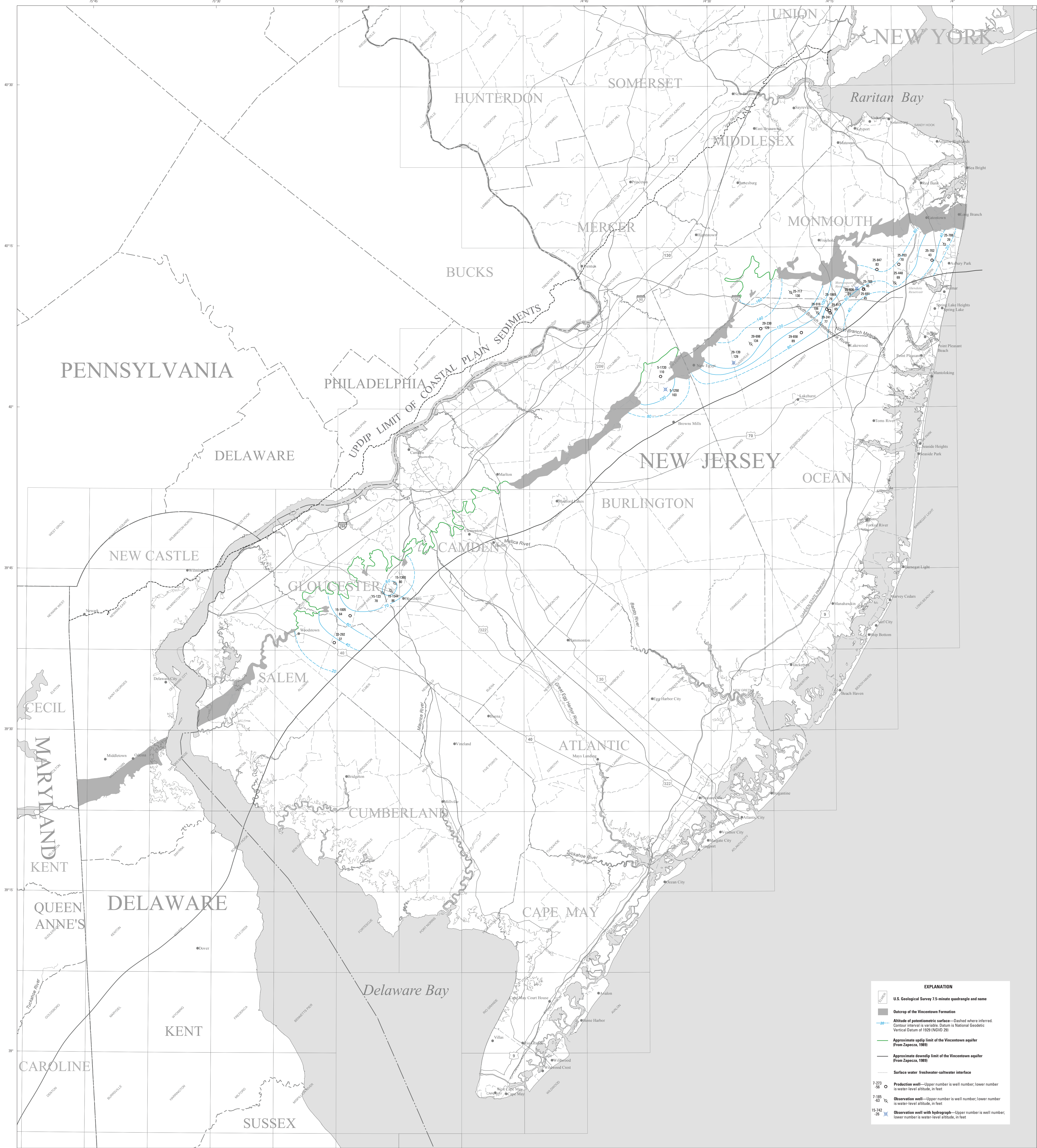
Potentiometric Surface of the Vincentown aquifer, 2008
