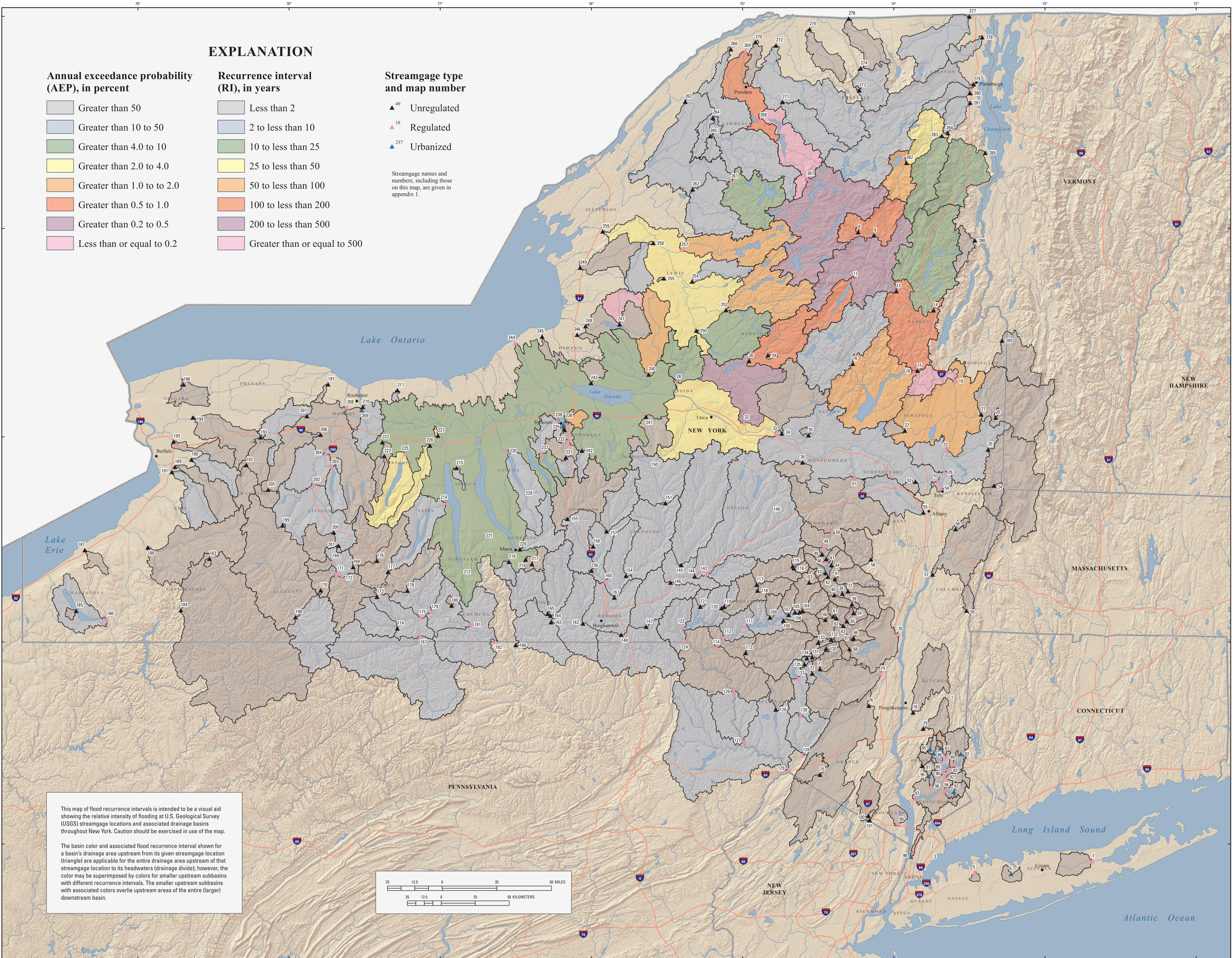
Figure 11. Annual exceedance probabilities (AEPs) and recurrence intervals (RIs) for the flood of April 26 to May 9, 2011, in selected U.S. Geological Survey streamgage basins in New York.
