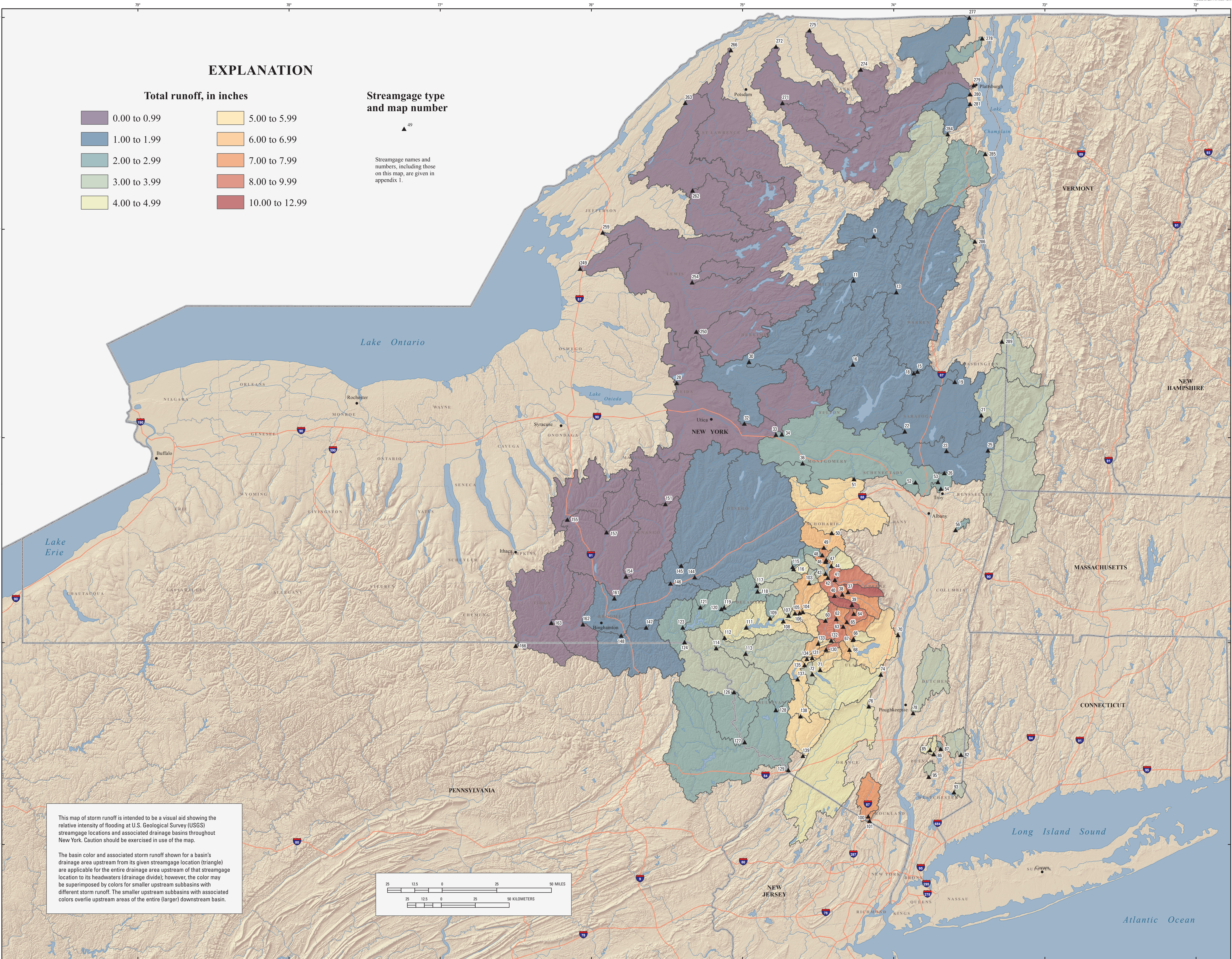
Figure 31. Total storm runoff in inches for August 27 to September 2, 2011, in selected U.S. Geological Survey streamgauge basins in New York.
