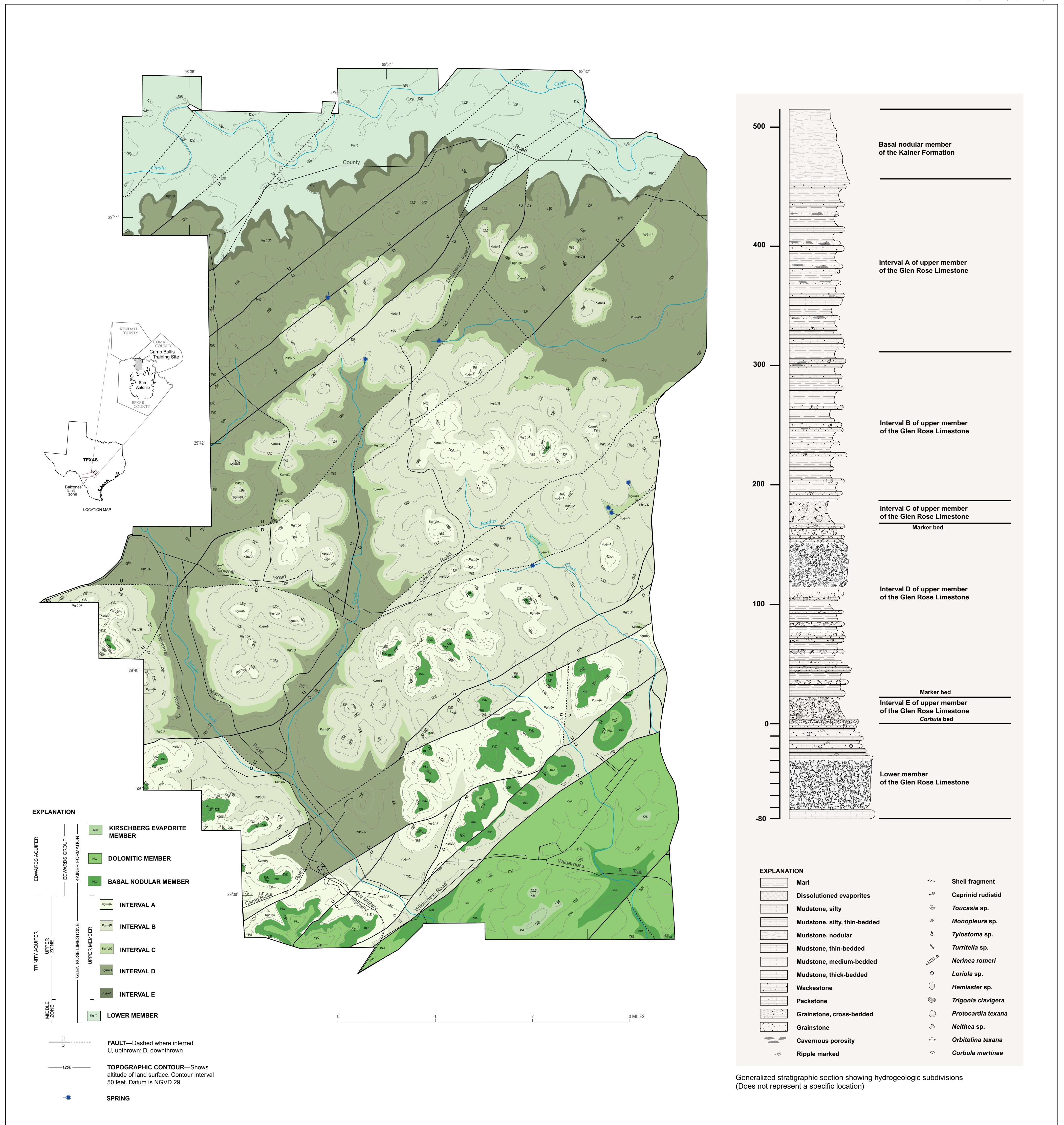
MAP SHOWING HYDROGEOLOGIC SUBDIVISIONS OF THE EDWARDS AND TRINITY AQUIFERS THAT CROP OUT; AND GENERALIZED STRATIGRAPHIC SECTION, CAMP BULLIS TRAINING SITE, BEXAR COUNTY, TEXAS
